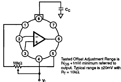
FIGURE 1. SUGGESTED V_{OS} ADJUSTMENT AND COMPENSATION HOOK UP
