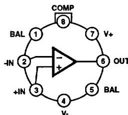
HA-2548 (TO-99 CAN) TOP VIEW
