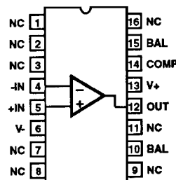
HA-2548 (300 mil SOIC) TOP VIEW
