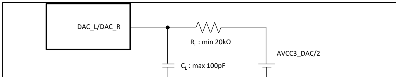
Figure 8-8: R_L is Connected to AVCC3_DAC/2 (Example)
