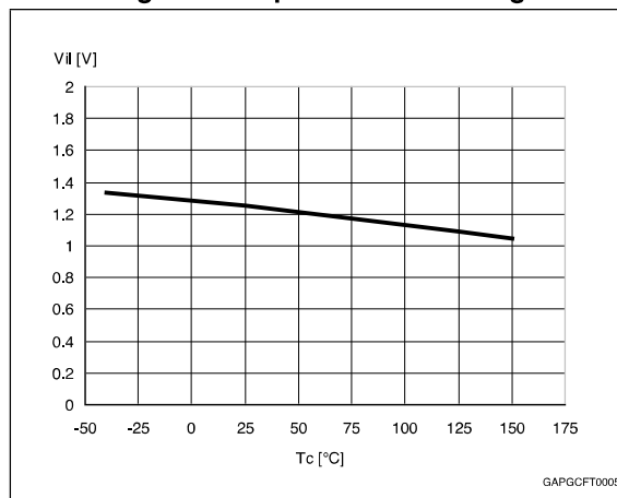
Figure 18. Input low level voltage
