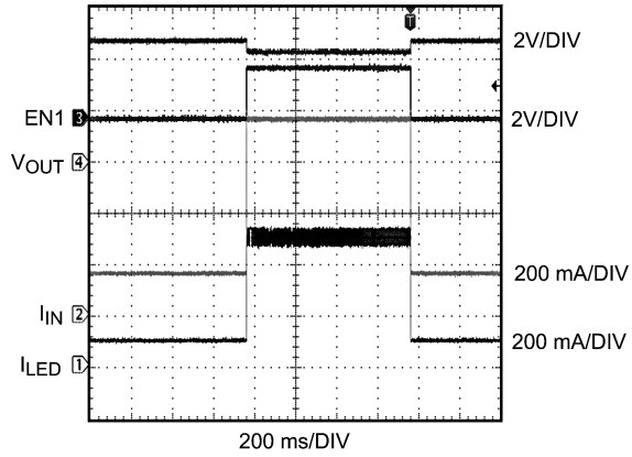
Torch to Flash Mode Transition EN2 = V_{IN} = 3.6V , I_{LED}(\text{Flash}) = 500\text{ mA} , Gain = 1.5x
