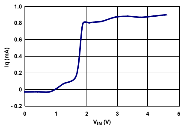
FIGURE 3. QUIESCENT CURRENT vs V_{IN} (ENAB = HI)
