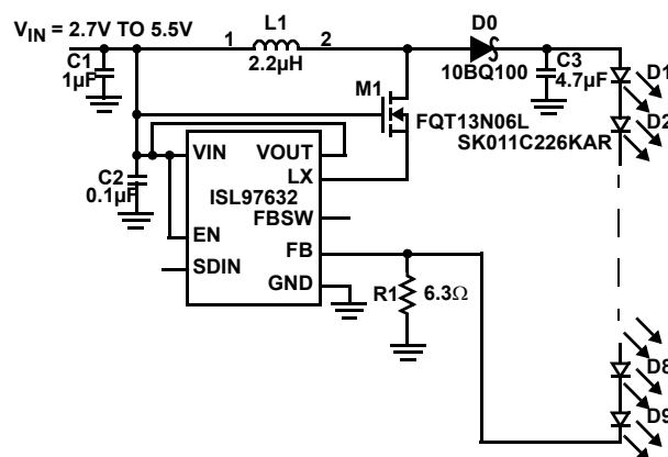
FIGURE 9. CONCEPTUAL 9 LEDs HIGH VOLTAGE DRIVER
