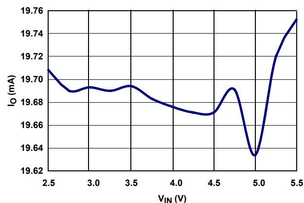
FIGURE 5. LINE REGULATION
