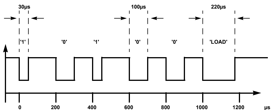
FIGURE 1. 1-WIRE XSD INTERFACE
