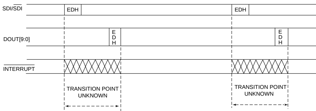
Fig. 11 \text{INTERRUPT} Timing
