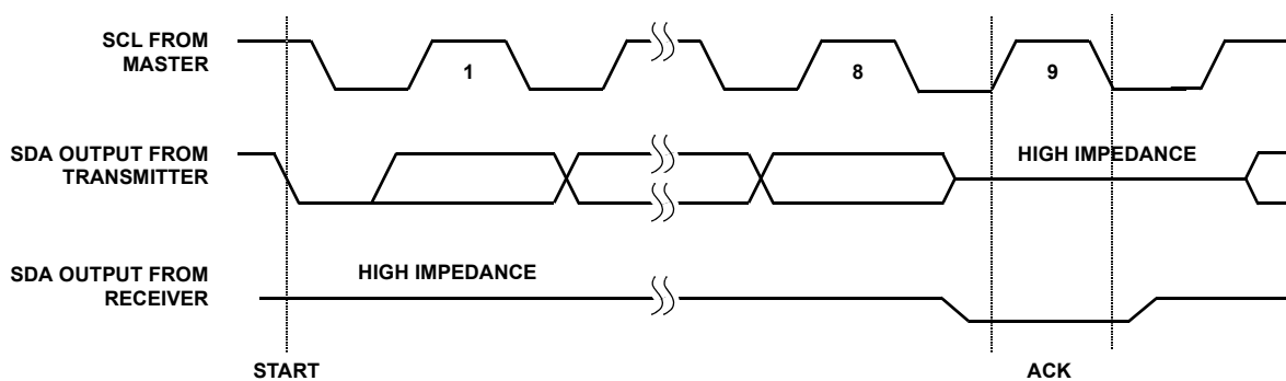
FIGURE 17. ACKNOWLEDGE RESPONSE FROM RECEIVER
