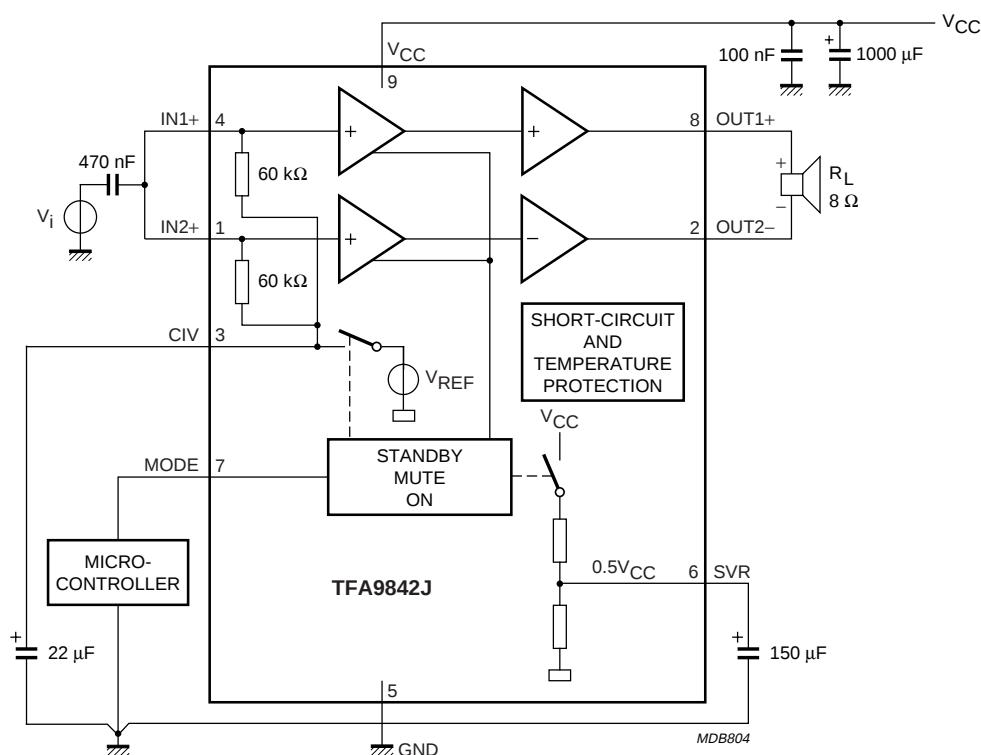
Fig 13. BTL application diagram.
