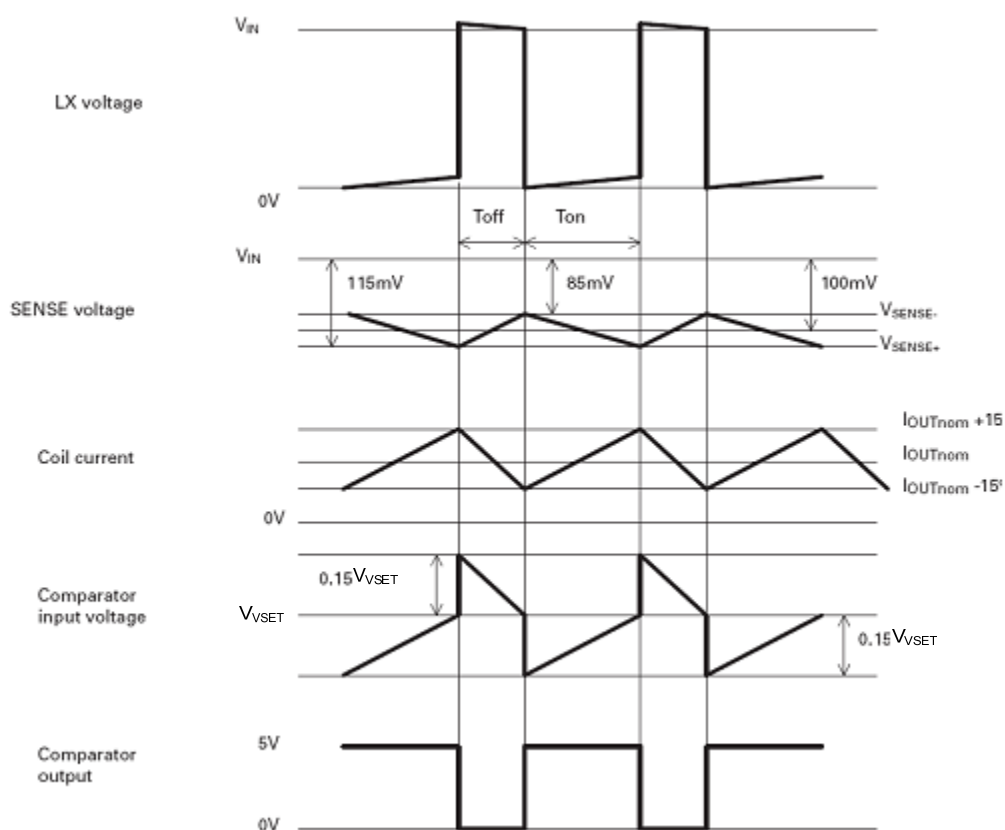
Figure 1. Operating Waveforms
