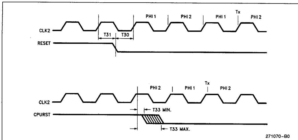
Figure 69. Reset Timing
