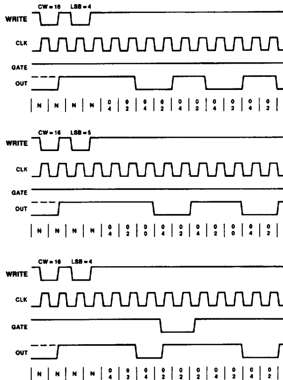
Figure 46. Mode 3
