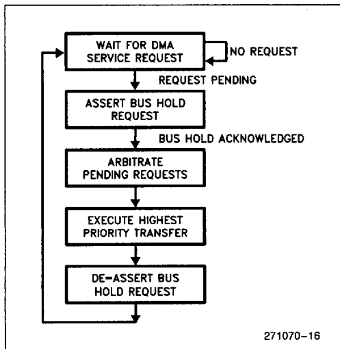
Figure 15. Flow of DMA Controller Operation
