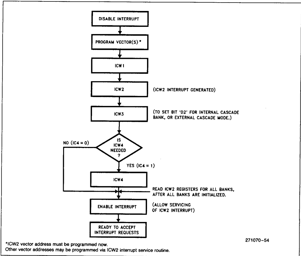
Figure 42. Initialization Sequence
