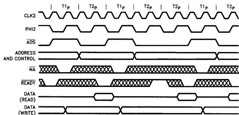
Figure 12. Pipelined Bus Cycles
