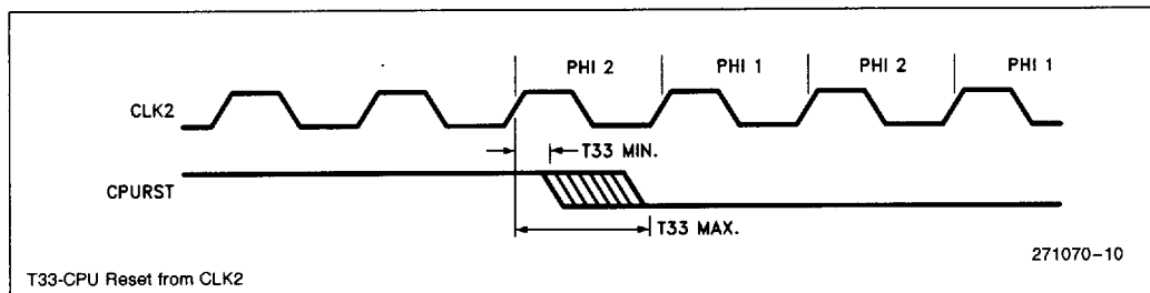
Figure 9. CPURST Timing
