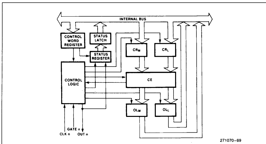
Figure 44. Internal Block Diagram of A Counter
