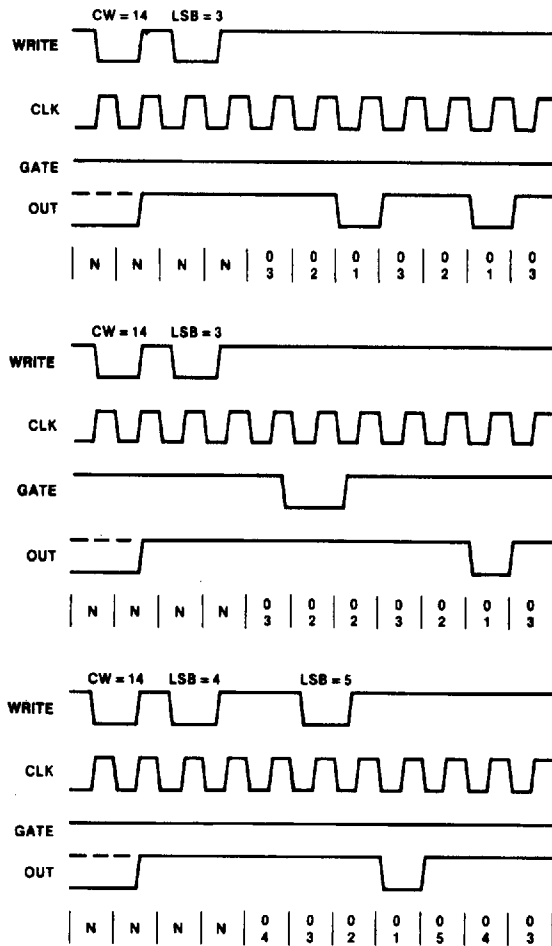
Figure 45. Mode 2
