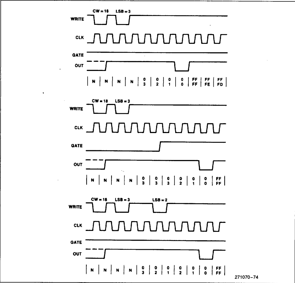
Figure 47. Mode 4
