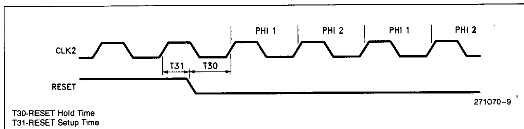
Figure 8. RESET Timing
