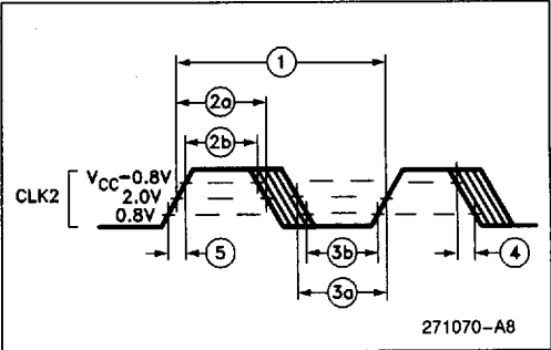
Figure 67. CLK2 Timing
