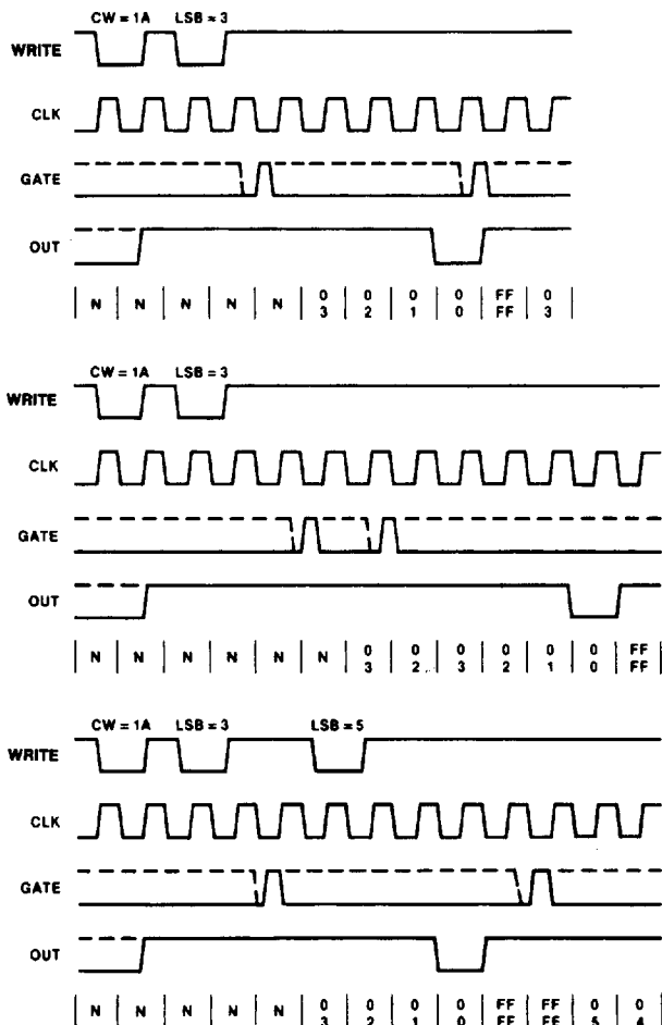
Figure 48. Mode 5
