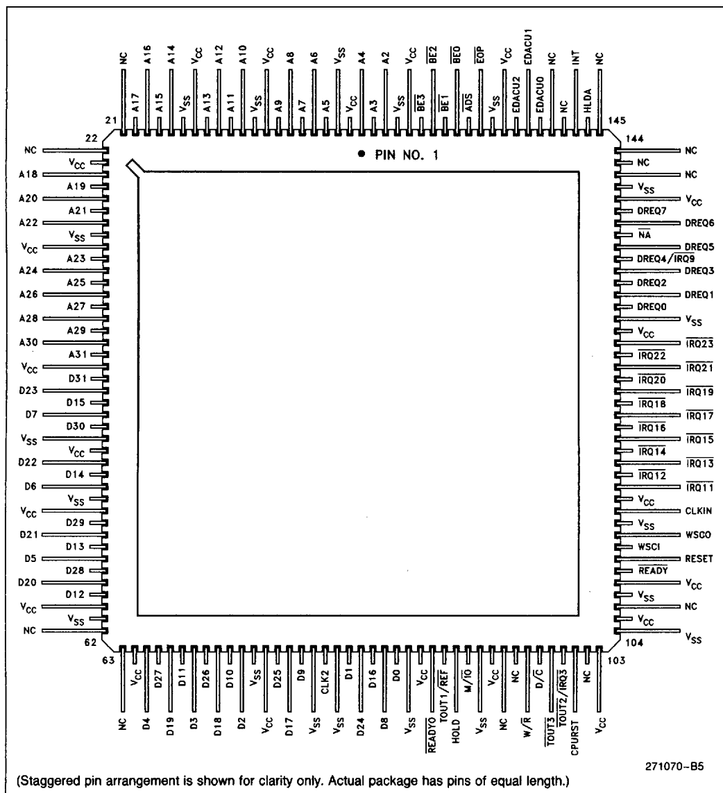
Figure 64. M82380 164-Lead CQFP Pinout (View from Top Side)
