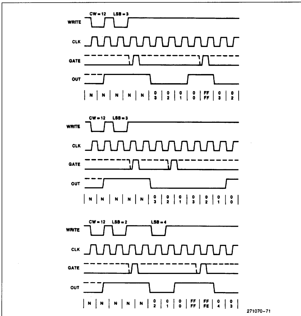
Figure 44. Mode 1
