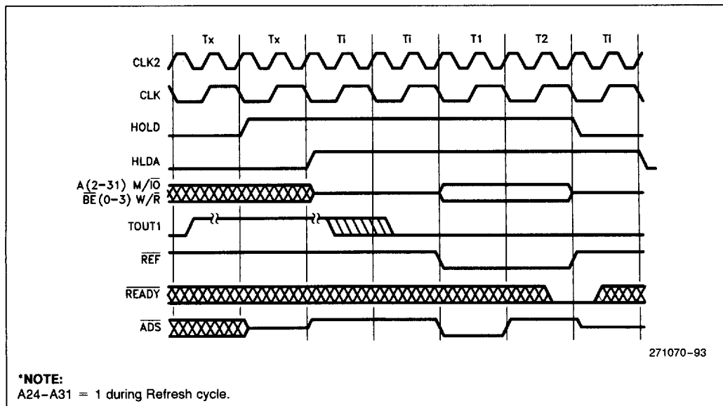
Figure 58. M82380 Refresh Cycle
