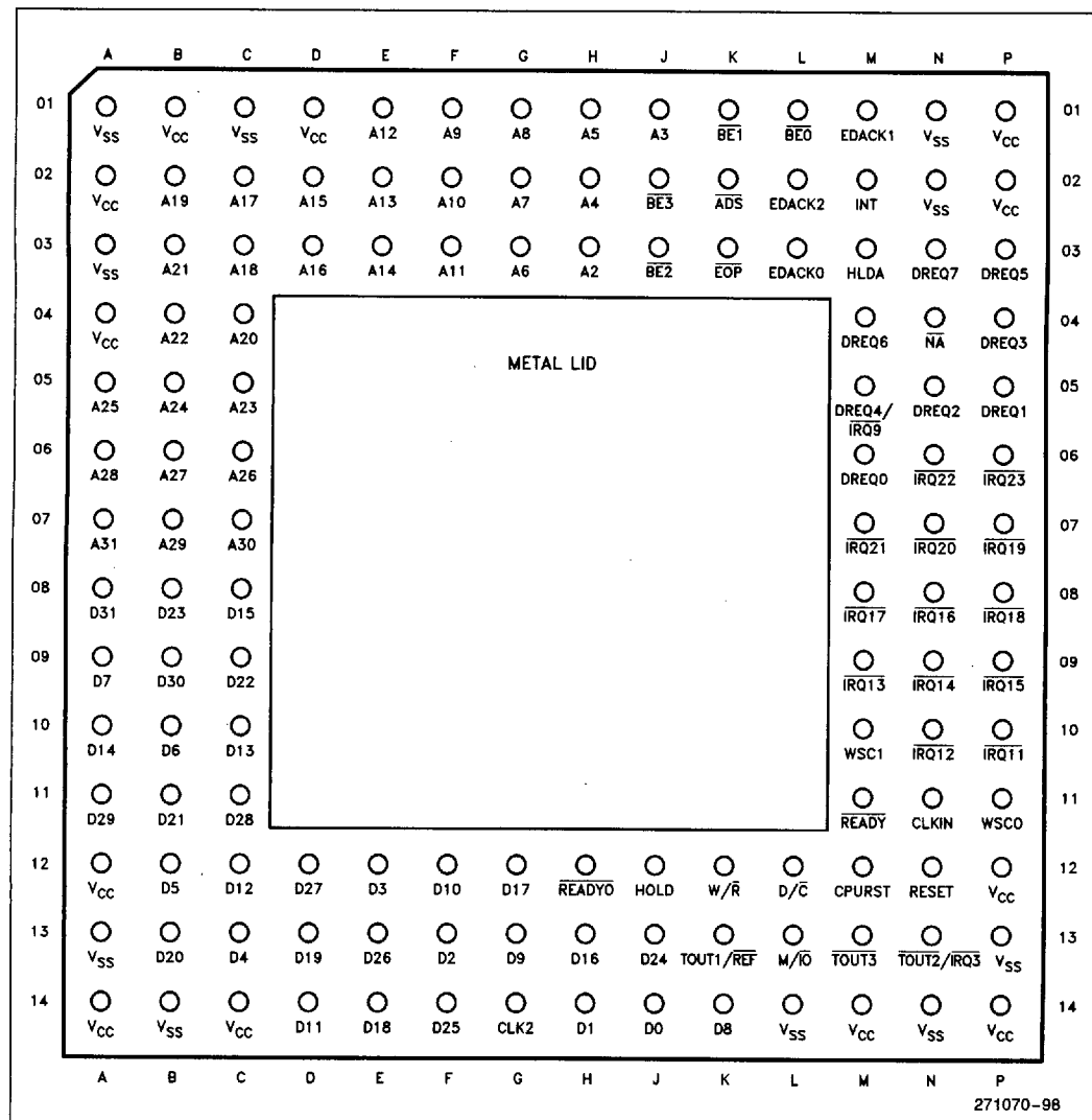
Figure 63. M82380 PGA Pinout—View from PIN side
