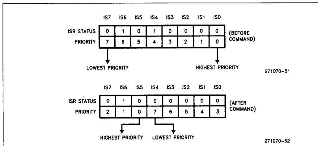
Figure 40. Rotate On Non-Specific EOI Command
