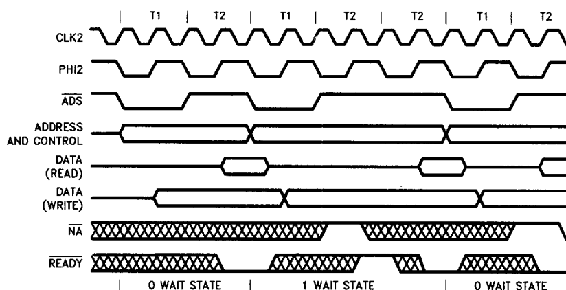
Figure 11. Non-Pipelined Bus Cycles
