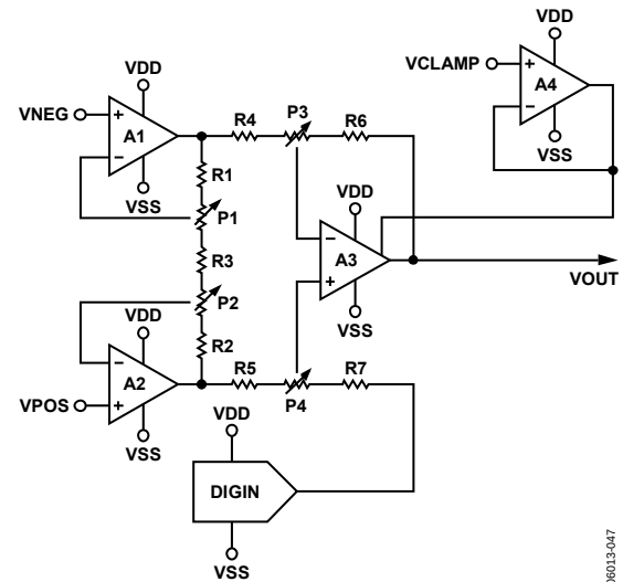
Figure 45. Functional Schematic
