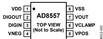
Figure 2. 8-Lead SOIC Pin Configuration
