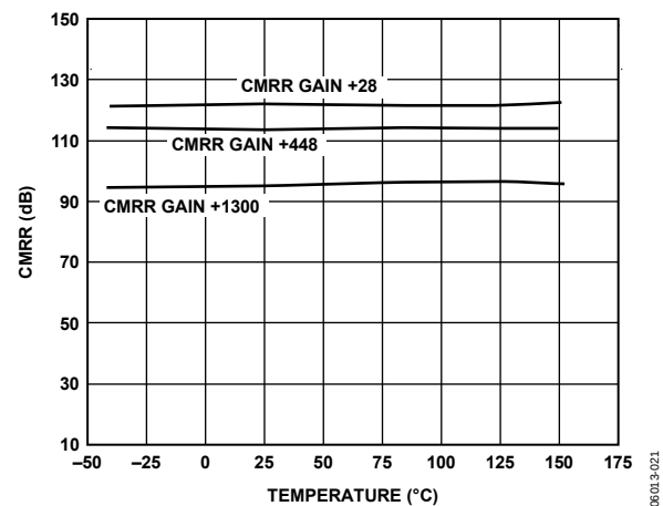
Figure 21. CMRR vs. Temperature at Different Gains, V_{SY} = 5\text{ V}
