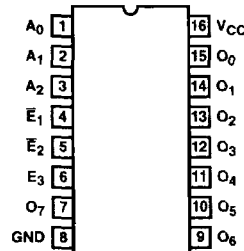
CD74FCT238T (QSOP, SOIC) TOP VIEW
