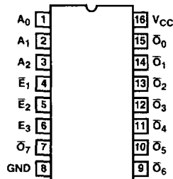
CD74FCT138T, (QSOP, SOIC) TOP VIEW
