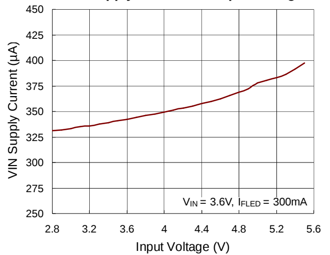
VIN Supply Current vs. Input Voltage
