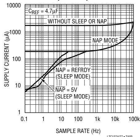
Supply Current vs Sample Rate with Sleep and Nap Modes
