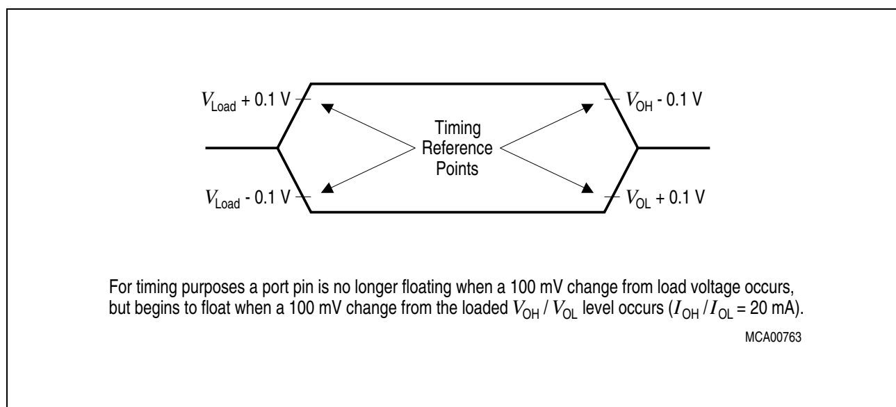
Figure 14 Float Waveforms
