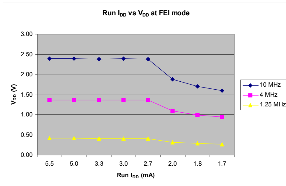
Figure 16. Typical Run I_{\text{DD}} vs. V_{\text{DD}} for FEI Mode
