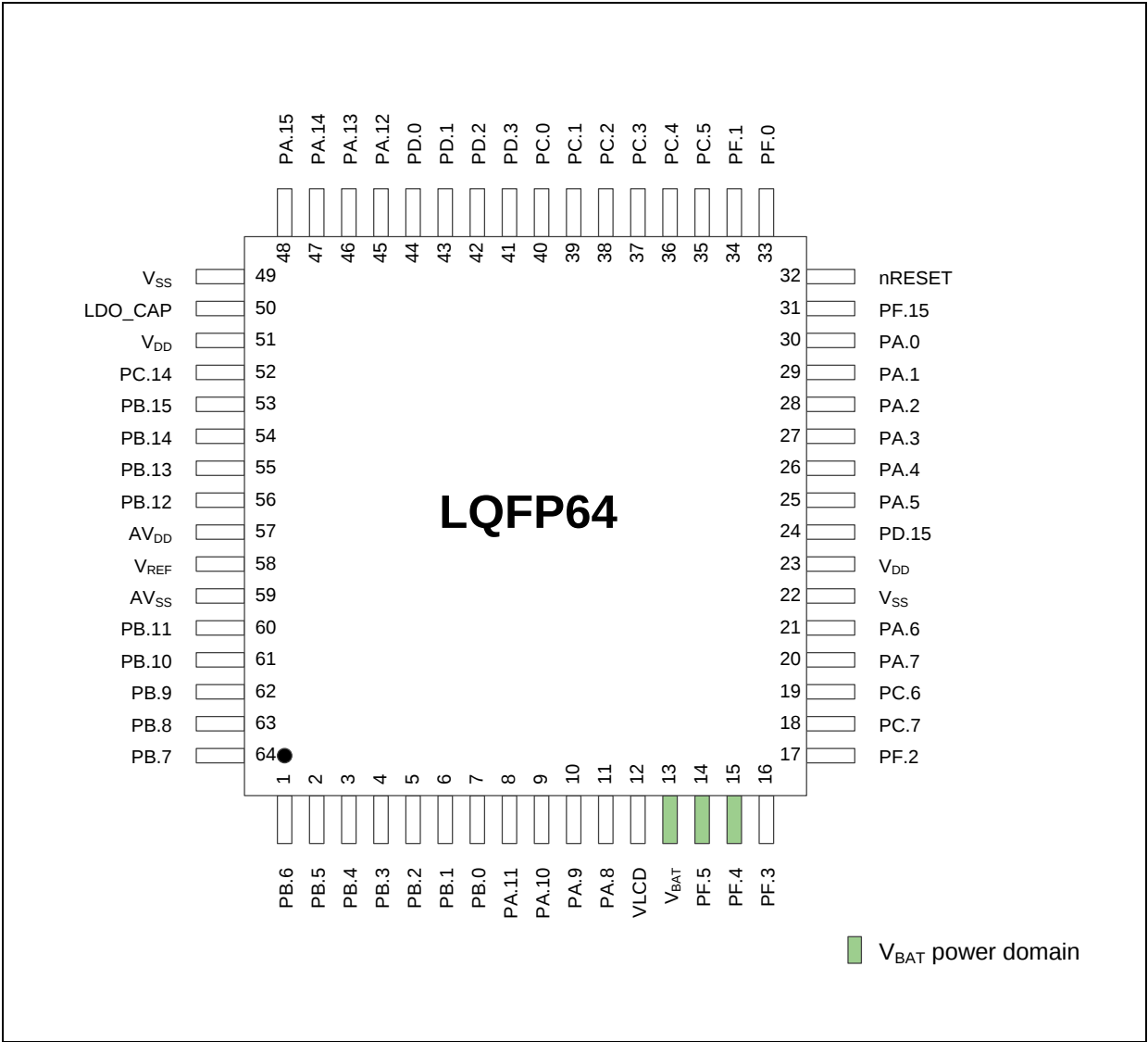
Figure 4.1-15 M256 Series LQFP 64-pin Diagram with V_{BAT}
