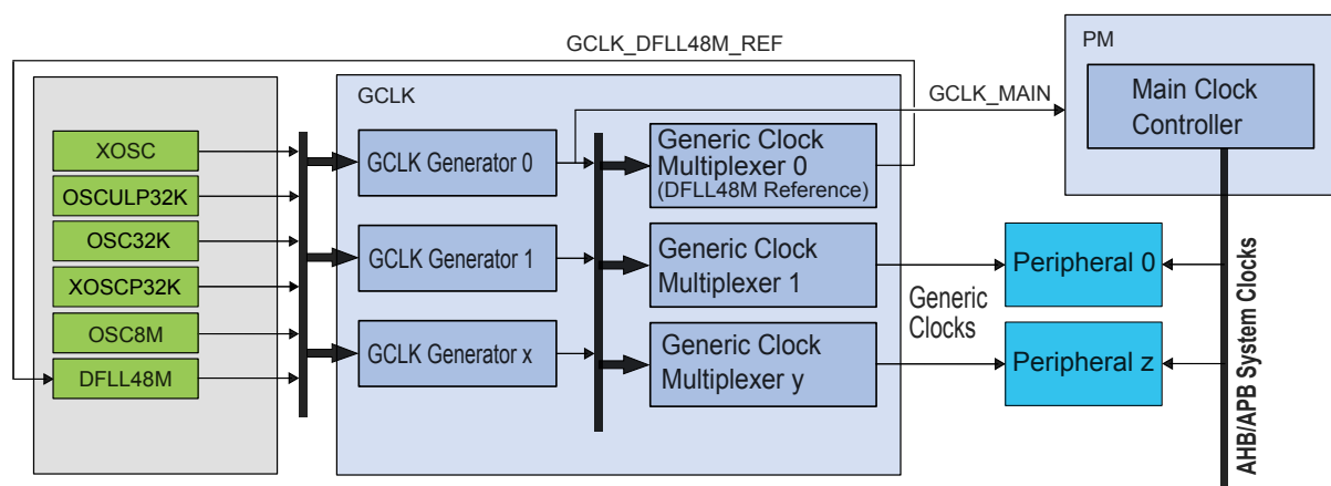
Figure 14-1. Clock distribution
