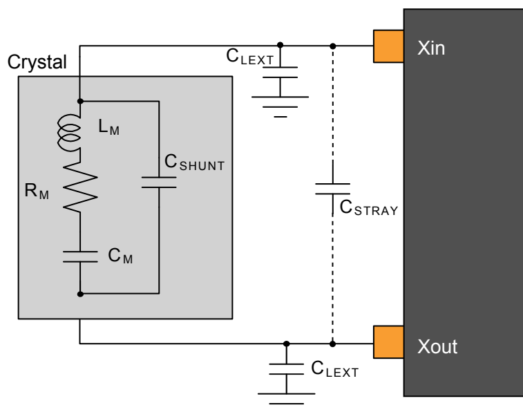
Figure 40-4. Oscillator Connection
