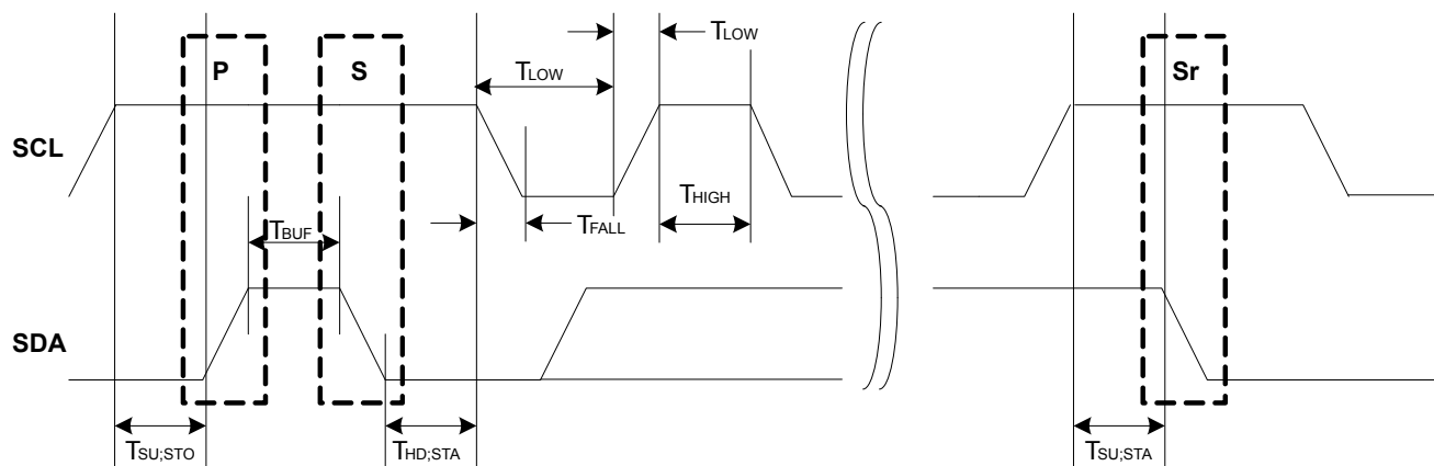
Figure 27-6. SCL Timing
