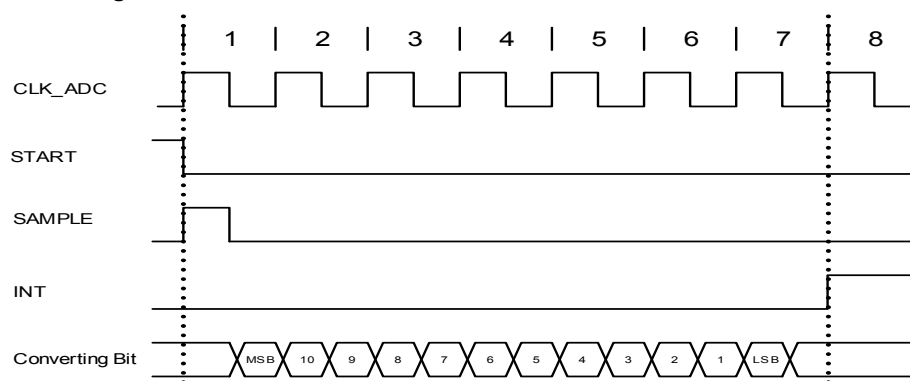
Figure 29-3. ADC Timing for One Conversion in Differential Mode without Gain
