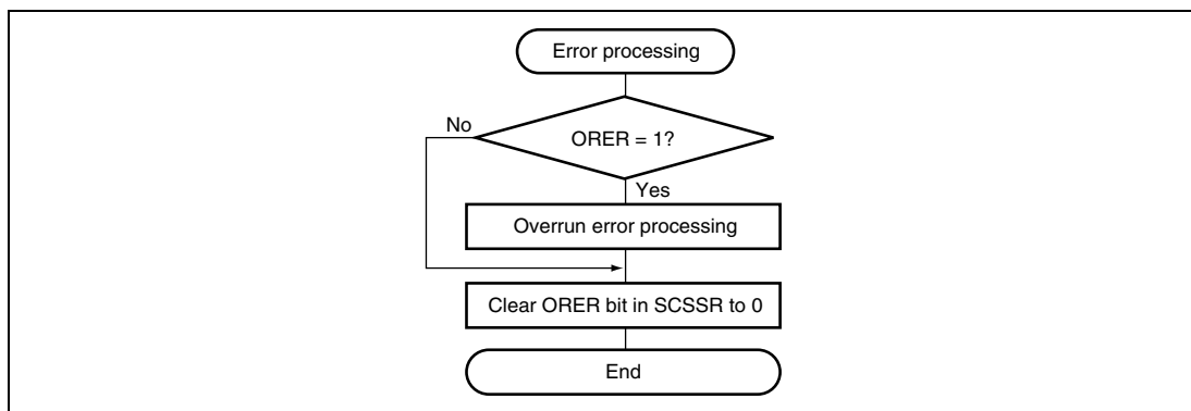
Figure 14.21 Sample Flowchart for Serial Data Receiving (cont)
