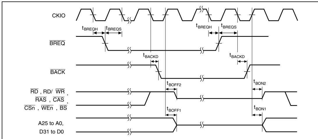
Figure 24.14 Bus Release Timing
