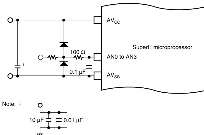
Figure 19.11 Example of Analog Input Protection Circuit
