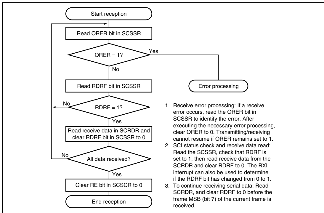
Figure 14.21 Sample Flowchart for Serial Data Receiving
