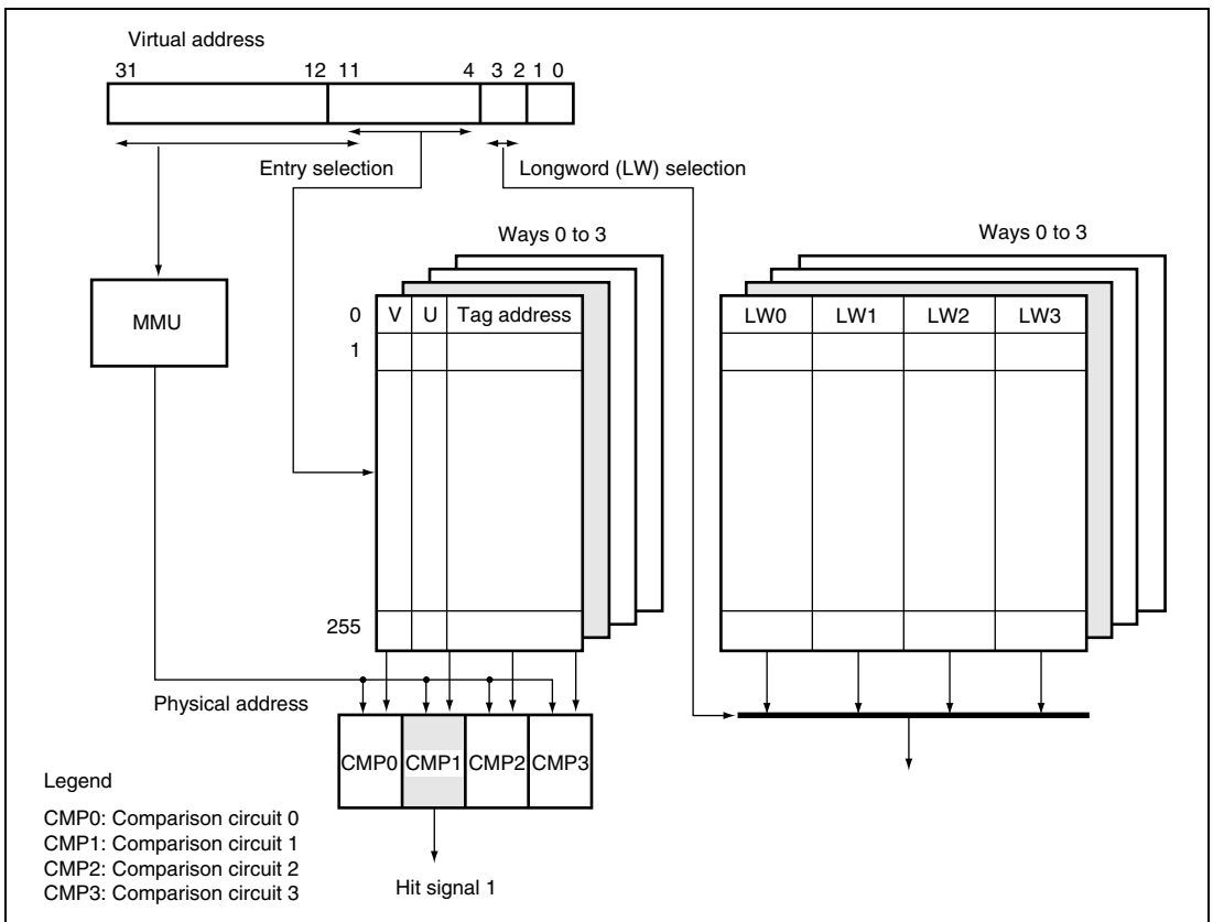
Figure 5.2 Cache Search Scheme (Normal Mode)
