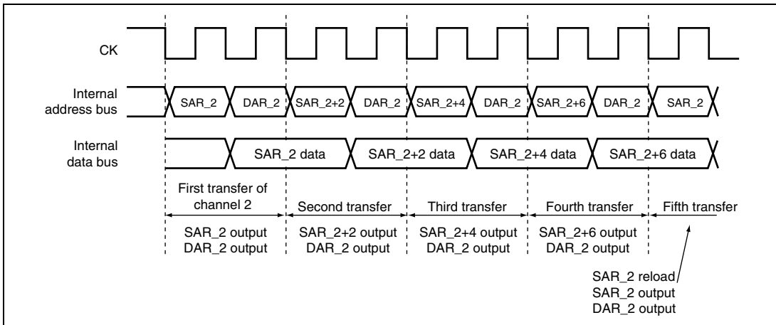
Figure 9.25 Timing Chart of Source Address Reload Function
