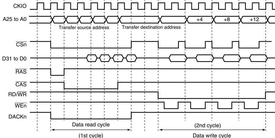
Figure 9.8 Example of DMA Transfer Timing in the Direct Address Mode in the Dual Address Mode (16-byte Transfer, Transfer Source: Synchronous DRAM, Transfer Destination: Ordinary Memory)
