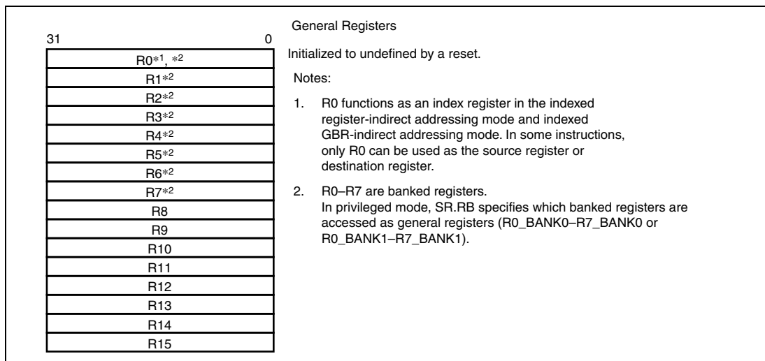
Figure 2.2 General Registers
