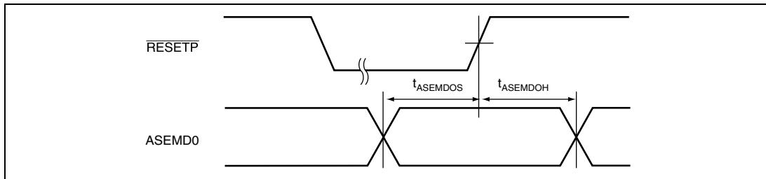
Figure 24.58 ASEMDO Input Timing
