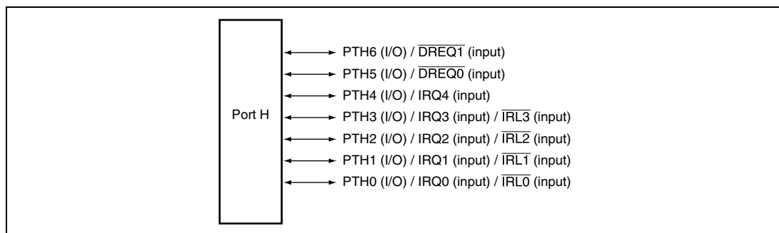
Figure 18.8 Port H
