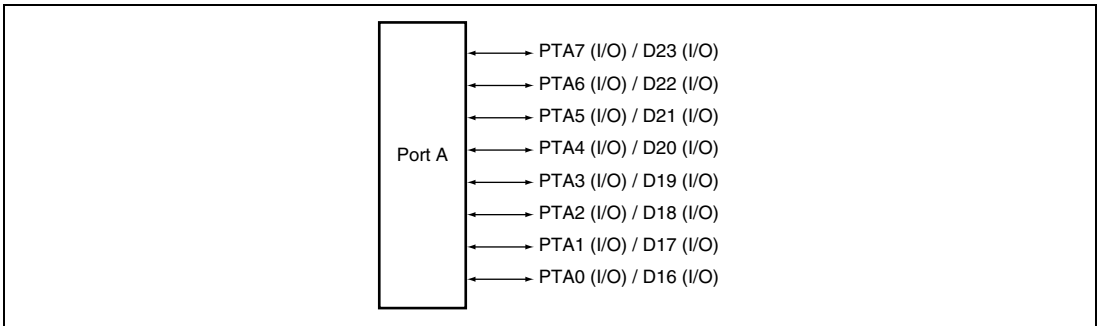
Figure 18.1 Port A
