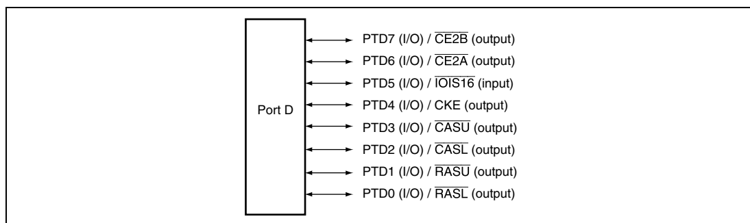
Figure 18.4 Port D
