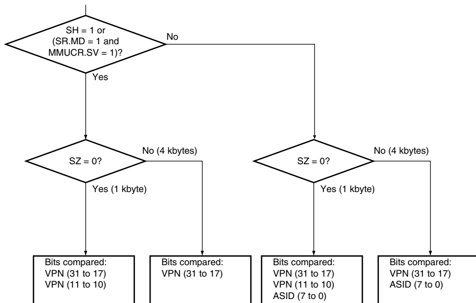
Figure 3.7 Objects of Address Comparison
