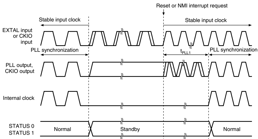
Figure 24.7 Oscillation Settling Time at Standby Return (Return by IRQ or IRL)
