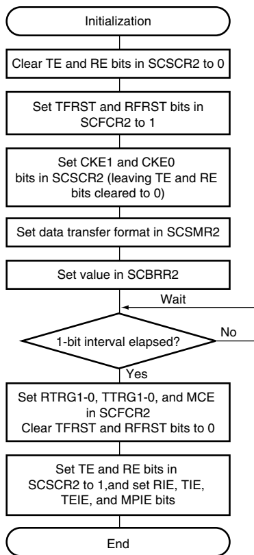
Figure 16.5 Sample SCIF Initialization Flowchart
