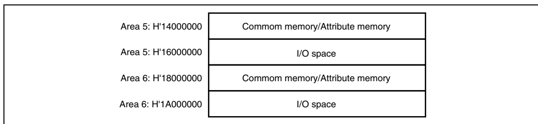
Figure 8.4 PCMCIA Space Allocation
