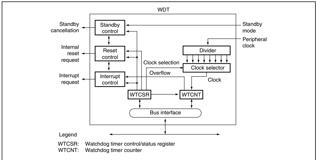
Figure 11.1 Block Diagram of the WDT
