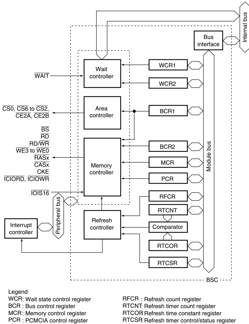
Figure 8.1 BSC Functional Block Diagram
