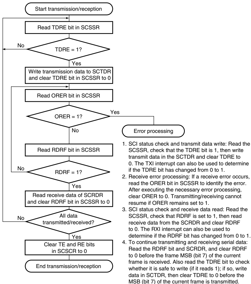
Figure 14.23 Sample Flowchart for Serial Data Transmitting/Receiving
