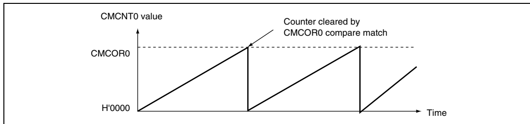
Figure 9.27 Counter Operation
