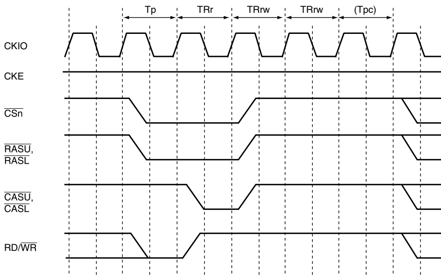
Figure 8.25 Synchronous DRAM Auto-Refresh Timing
