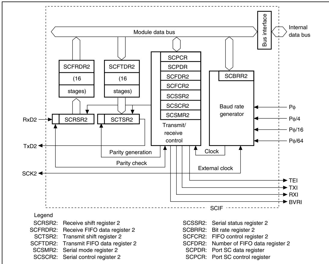
Figure 16.1 SCIF Block Diagram
