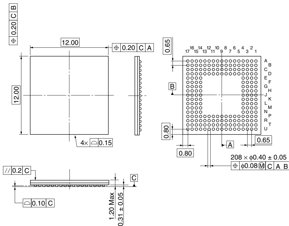
Figure D.2 Package Dimensions (TBP-208AV)
