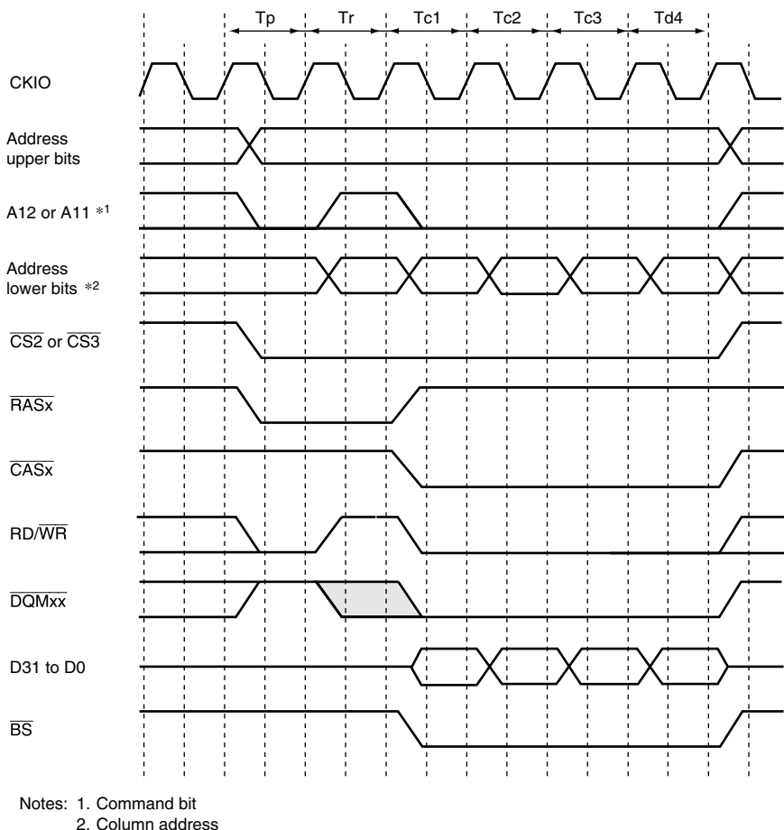
Figure 8.23 Burst Write Timing (Different Row Addresses)
