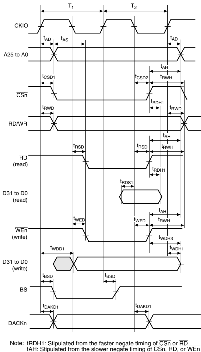
Figure 24.16 Basic Bus Cycle (No Wait)
