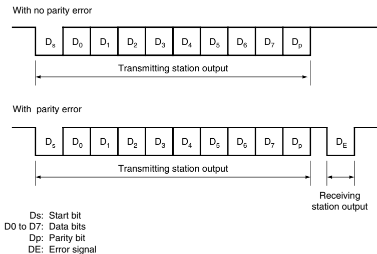
Figure 15.3 Data Format for Smart Card Interface
