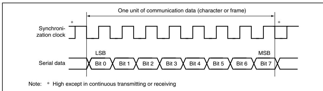
Figure 14.17 Data Format in Clock Synchronous Communication
