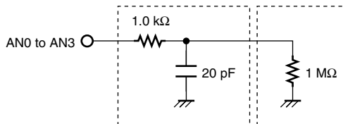
Figure 19.12 Analog Input Pin Equivalent Circuit
