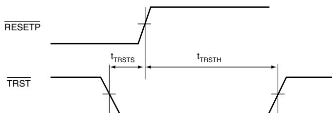
Figure 24.56 TRST Input Timing (Reset Hold)
