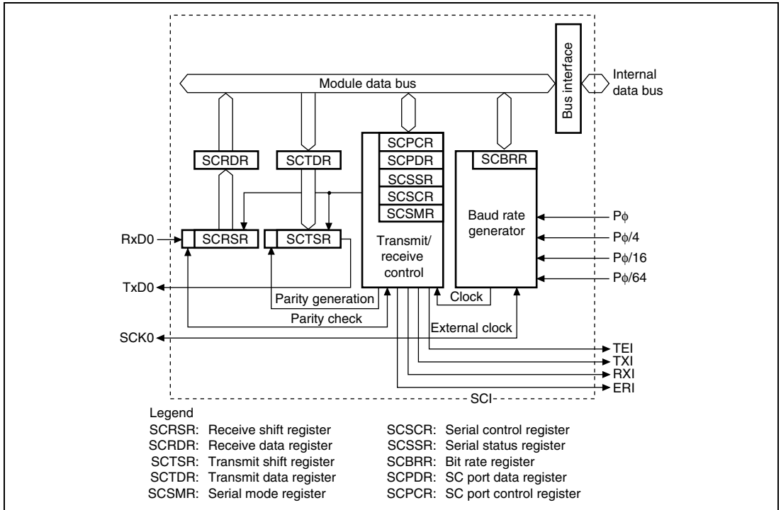
Figure 14.1 SCI Block Diagram
