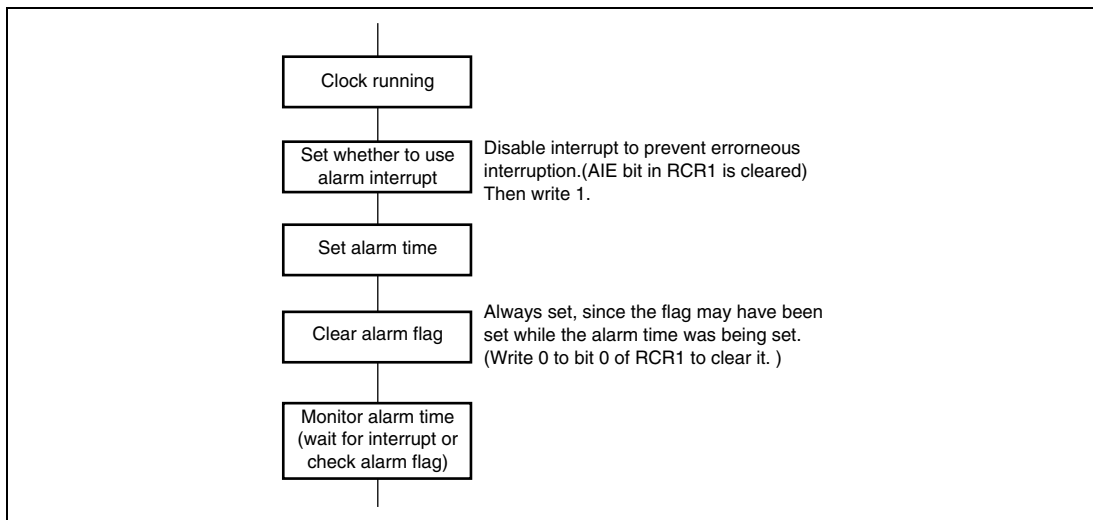
Figure 13.4 Using the Alarm Function
