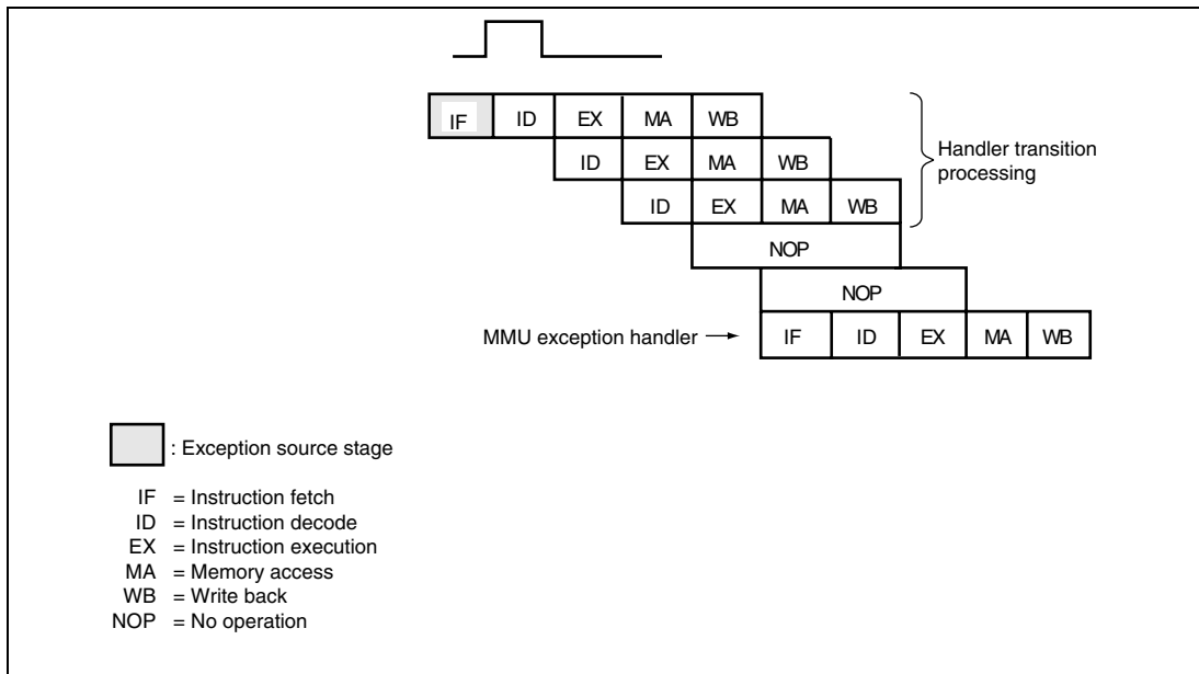
Figure 3.11 MMU Exception Signals in Instruction Fetch
