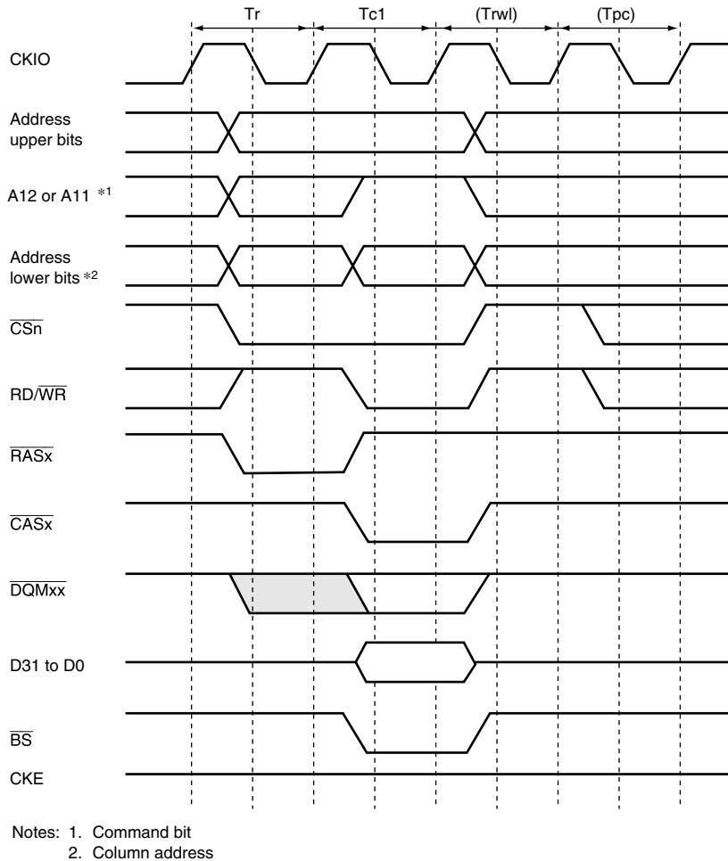
Figure 8.17 Basic Timing for Synchronous DRAM Single Write
