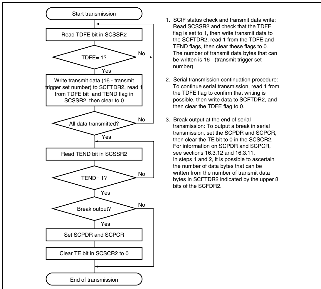
Figure 16.6 Sample Serial Transmission Flowchart
