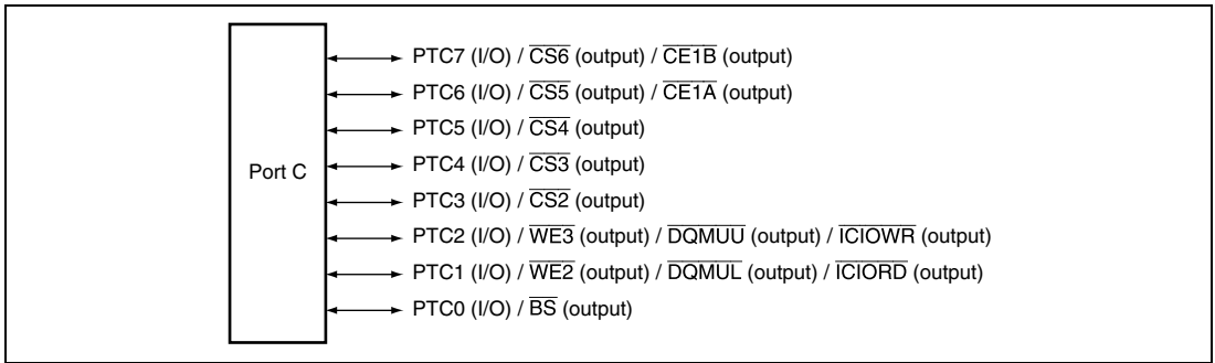
Figure 18.3 Port C
