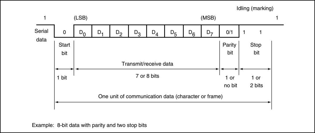
Figure 14.5 Data Format in Asynchronous Communication
