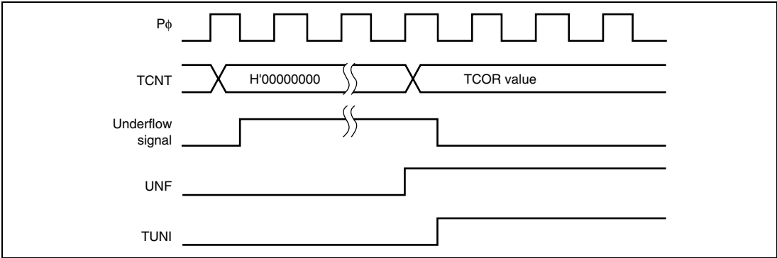
Figure 12.8 UNF Set Timing
