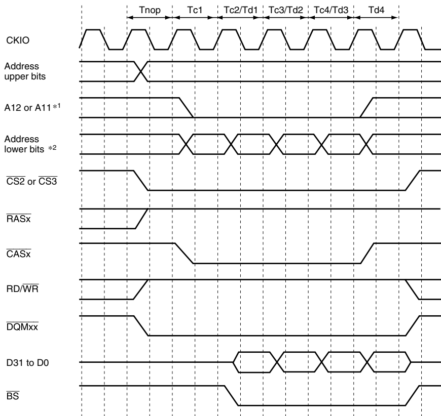
Figure 8.19 Burst Read Timing (Same Row Address)
