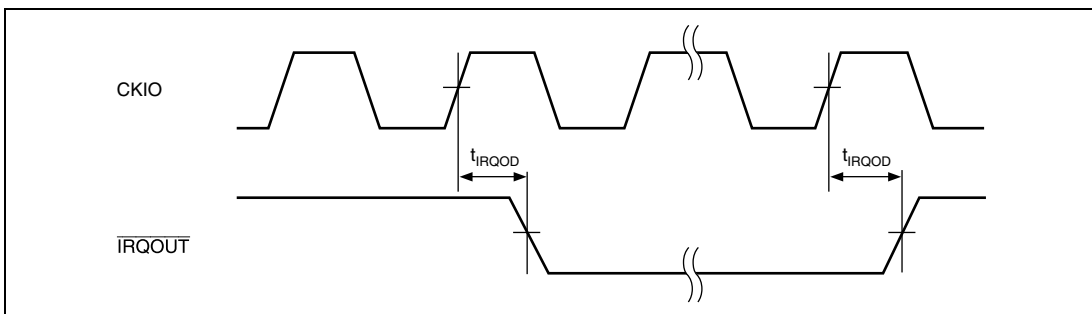
Figure 24.13 \overline{\text{IRQOUT}} Timing
