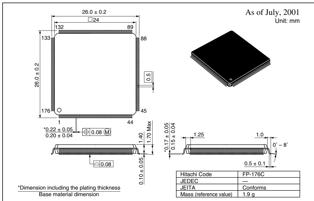
Figure D.1 Package Dimensions (FP-176C)
