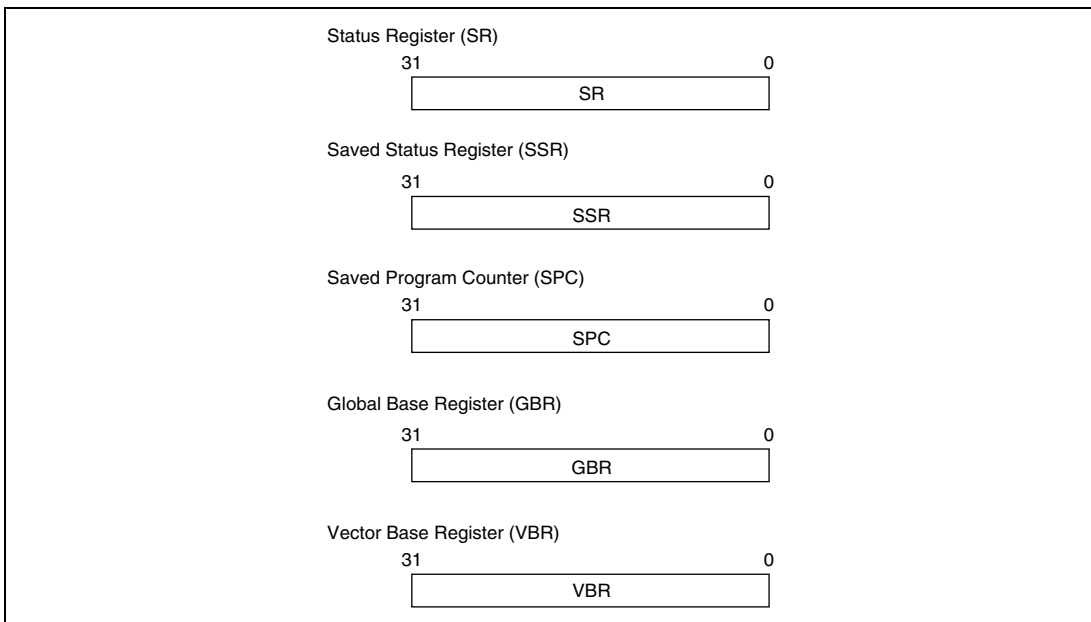
Figure 2.4 Control Registers
