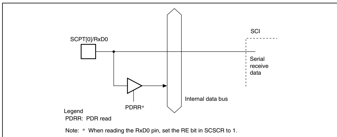
Figure 14.4 SCPT[0]/Rx0 Pin
