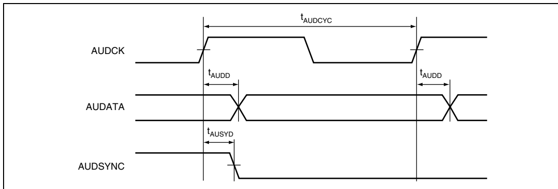
Figure 24.59 AUD Timing
