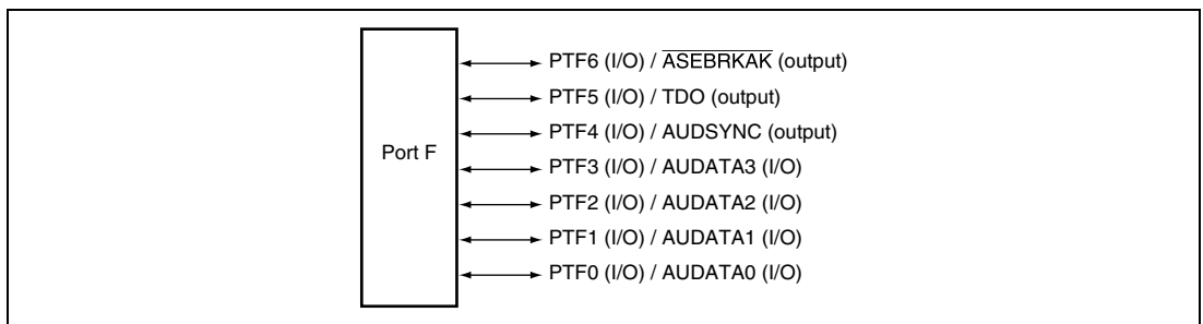
Figure 18.6 Port F
