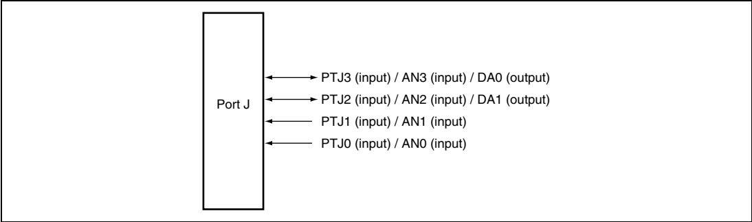
Figure 18.9 Port J
