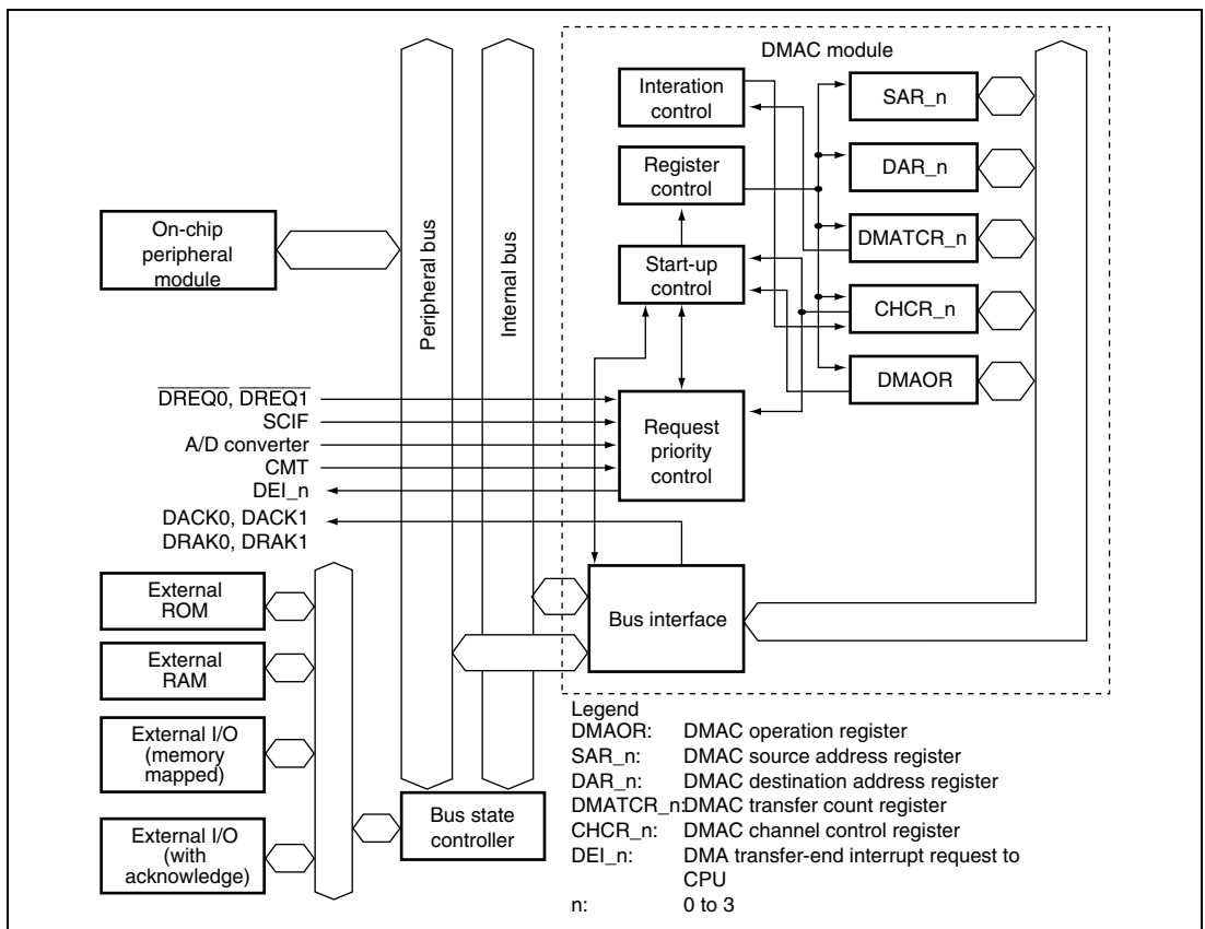
Figure 9.1 DMAC Block Diagram
