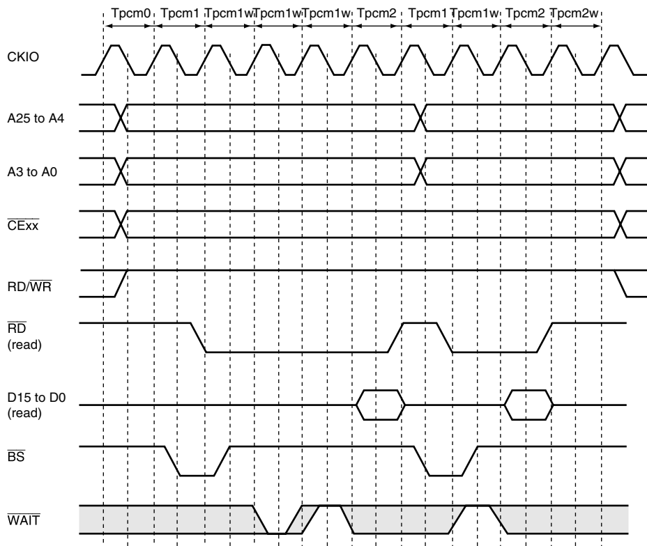
Figure 8.35 Wait Timing for PCMCIA Memory Card Interface Burst Access
