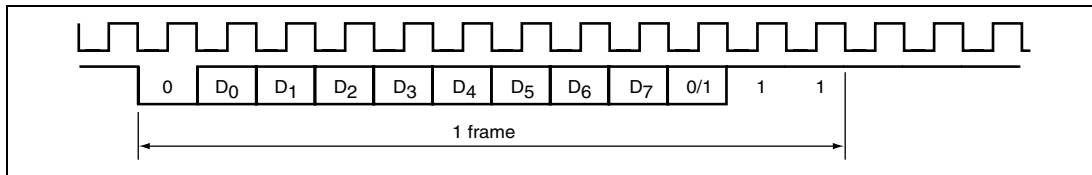
Figure 14.6 Output Clock and Serial Data Timing (Asynchronous Mode)
