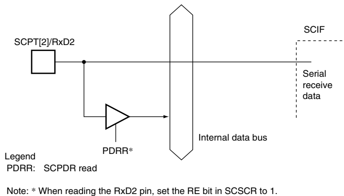
Figure 16.4 SCPT[2]/Rx2D Pin
