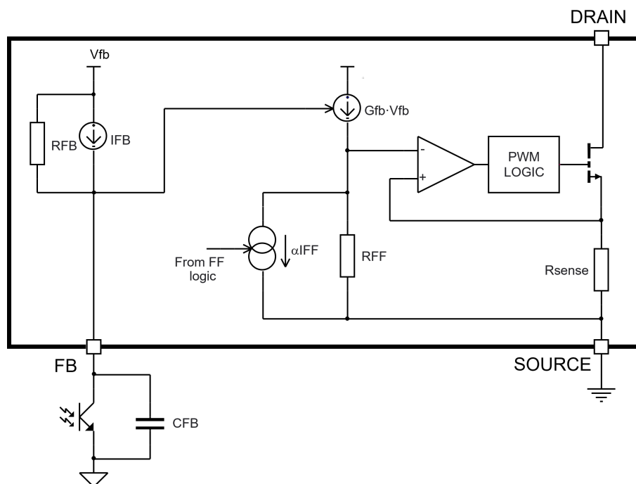
Figure 14. Burst-mode operation
