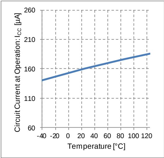
Figure 13. Circuit Current at Operation vs Temperature
