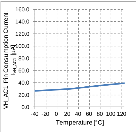
Figure 17. VH_AC1 Pin Consumption Current vs Temperature
