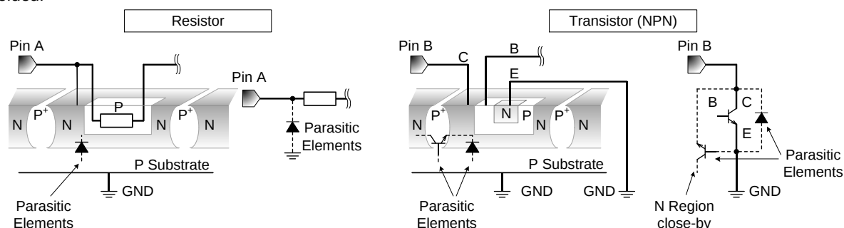
Figure 25. Example of IC Structure
