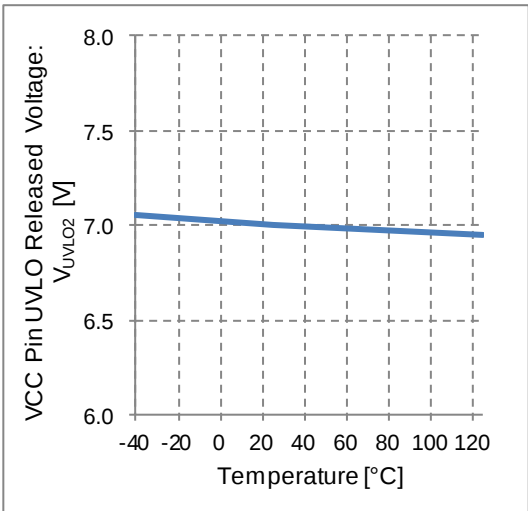
Figure 15. VCC Pin UVLO Released Voltage vs Temperature
