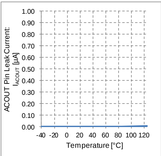
Figure 19. ACOUT Pin Leak Current vs Temperature
