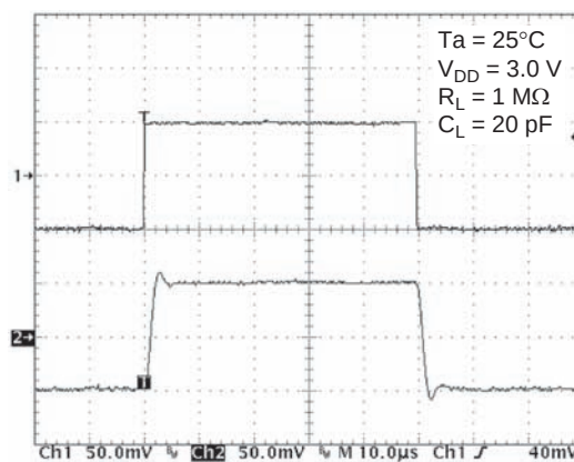
Figure 1-20. HA1630D01 Small Signal Transient Response
