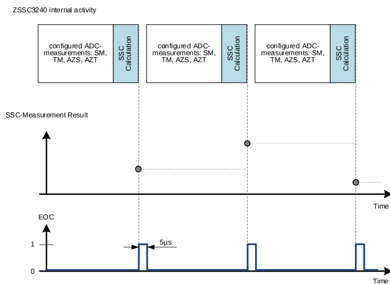
Figure 22. EOC-Behavior: Signalization of End-of-Conversion ( INT\_setup = 00_{BIN} )
