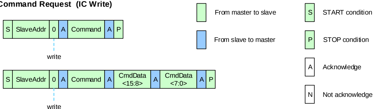
Figure 10. I2C Command Request
