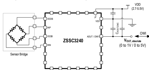
Analog Sensor with Absolute Voltage Out
