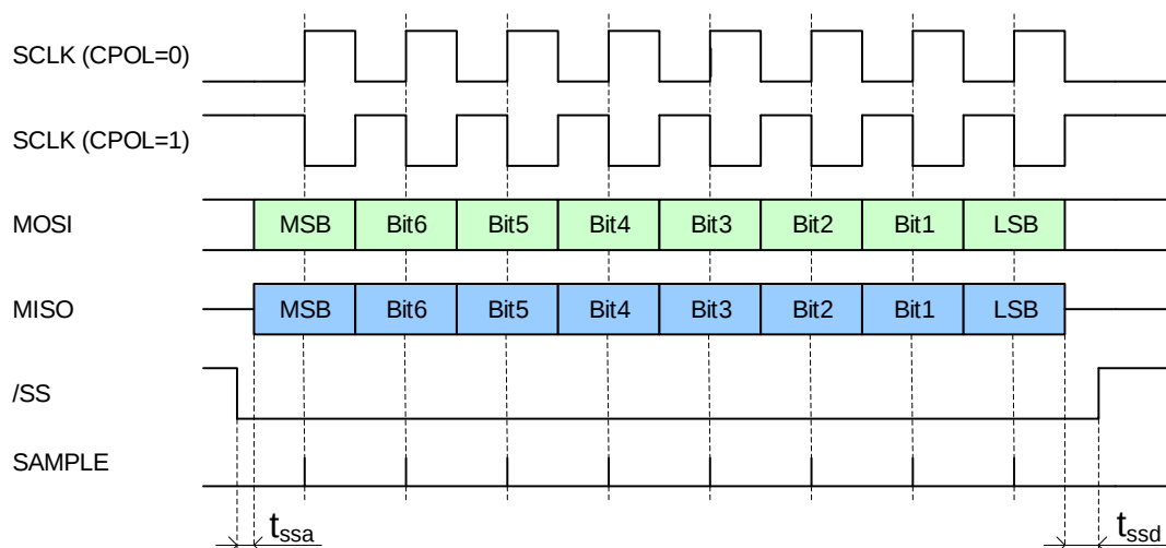
Figure 5. SPI Configuration CPHA=0
