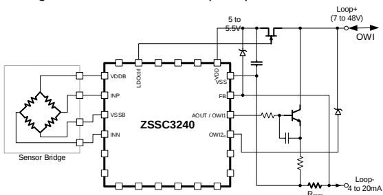
Analog Sensor with Current Loop Output, OUI, and External JFET
