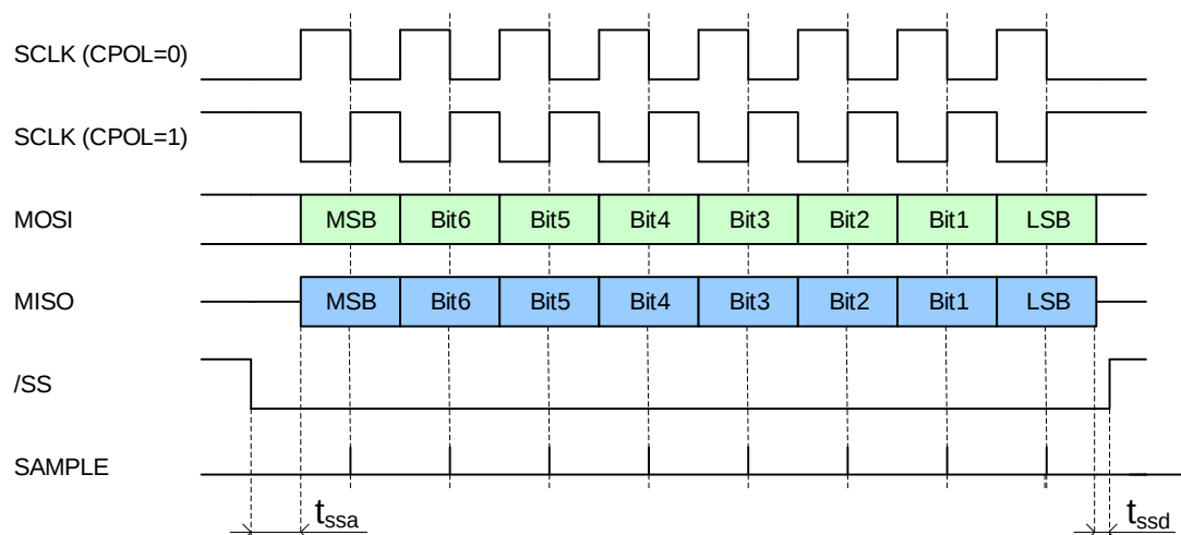
Figure 6. SPI Configuration CPHA=1
