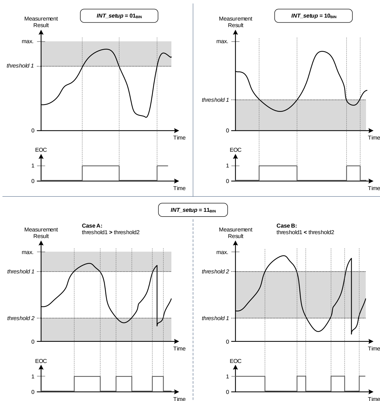
Figure 23. EOC and Interrupt Thresholds
