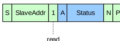
Figure 12. I2C Read Status
