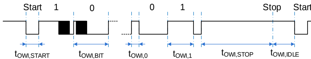
Figure 14. OWI Timing Diagram
