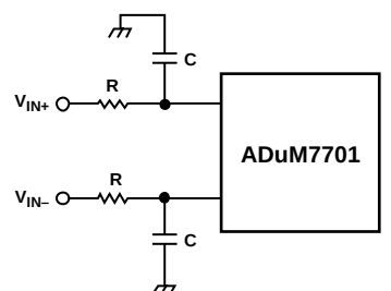
Figure 29. RC Low-Pass Filter Input Network
