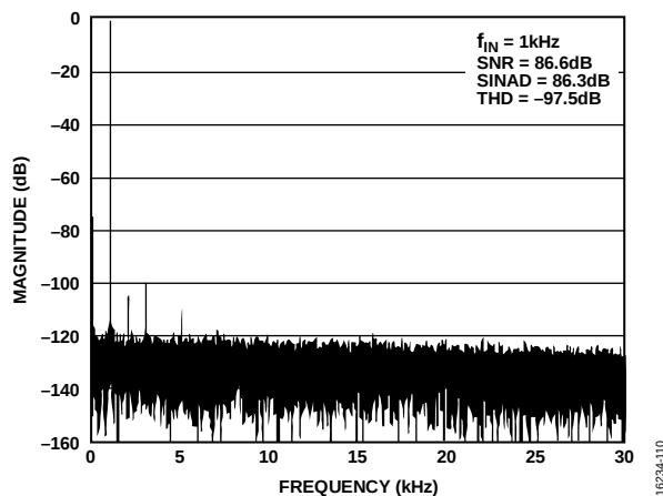
Figure 10. Typical Fast Fourier Transform (FFT)
