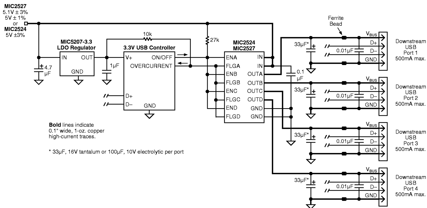
4-Port Self-Powered Hub
