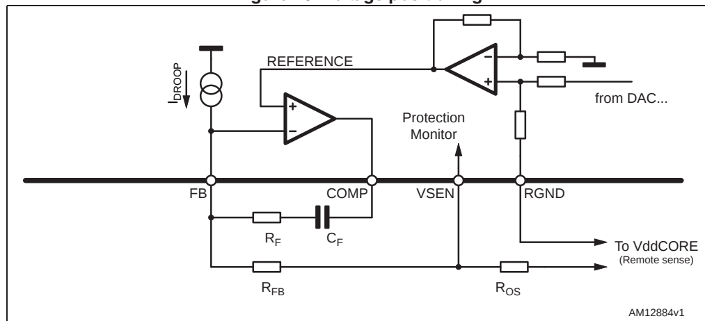
Figure 10. Voltage positioning
