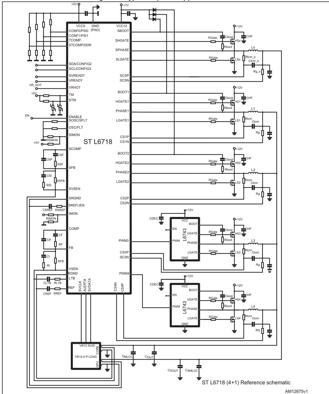
Figure 1. Typical 4-phase application circuit
