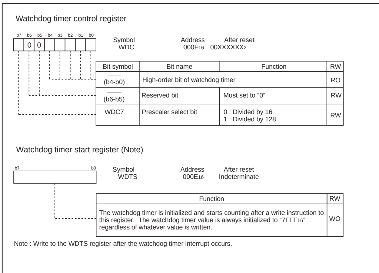
Figure 1.10.2. WDC Register and WDTN Register
