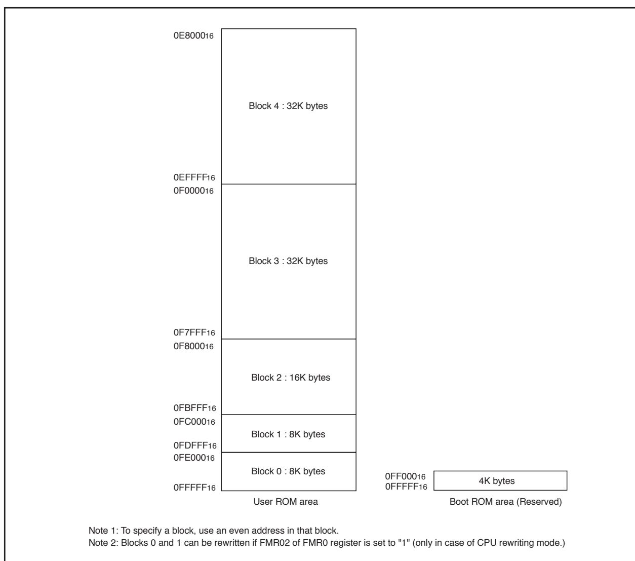
Figure 1.20.2. Flash Memory Block Diagram (ROM Capacity 96K bytes)
