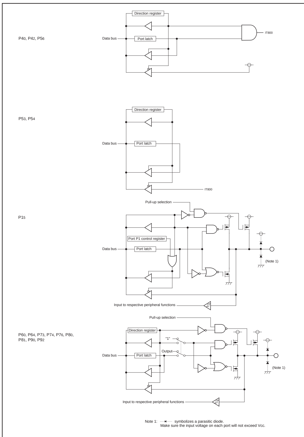
Figure 1.18.1. I/O Ports (1)
