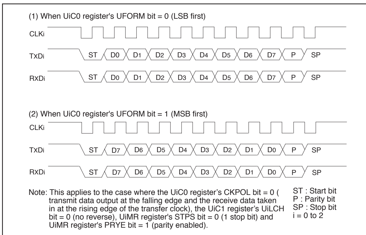
Figure 1.15.3. Transfer Format
