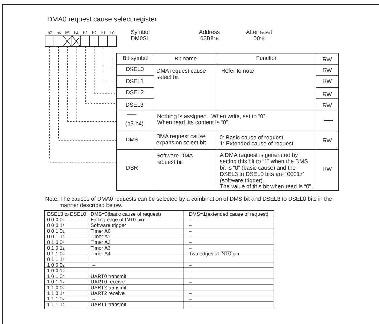
Figure 1.11.2. DM0SL Register
