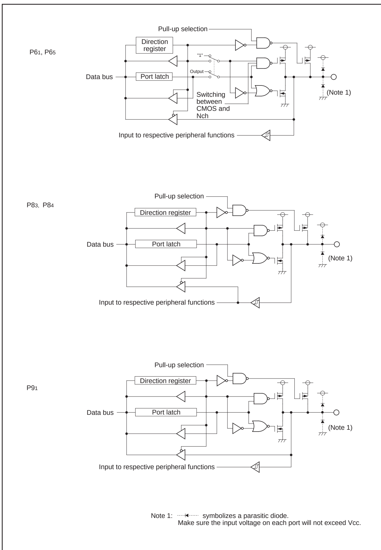
Figure 1.18.2. I/O Ports (2)
