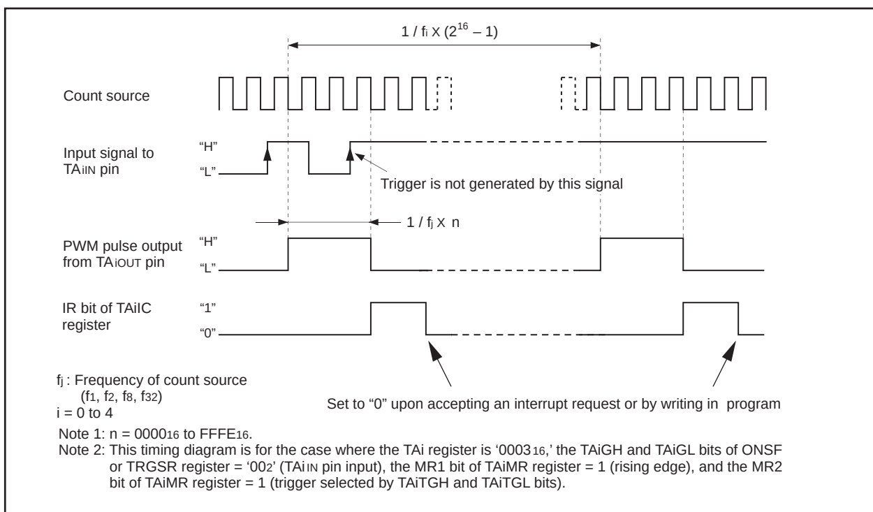
Figure 1.12.11. Example of 16-bit Pulse Width Modulator Operation
