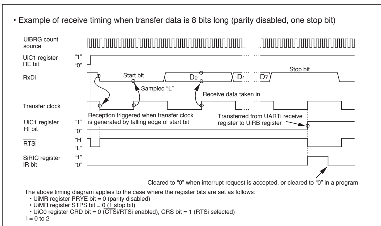
Figure 1.15.2. Receive Operation
