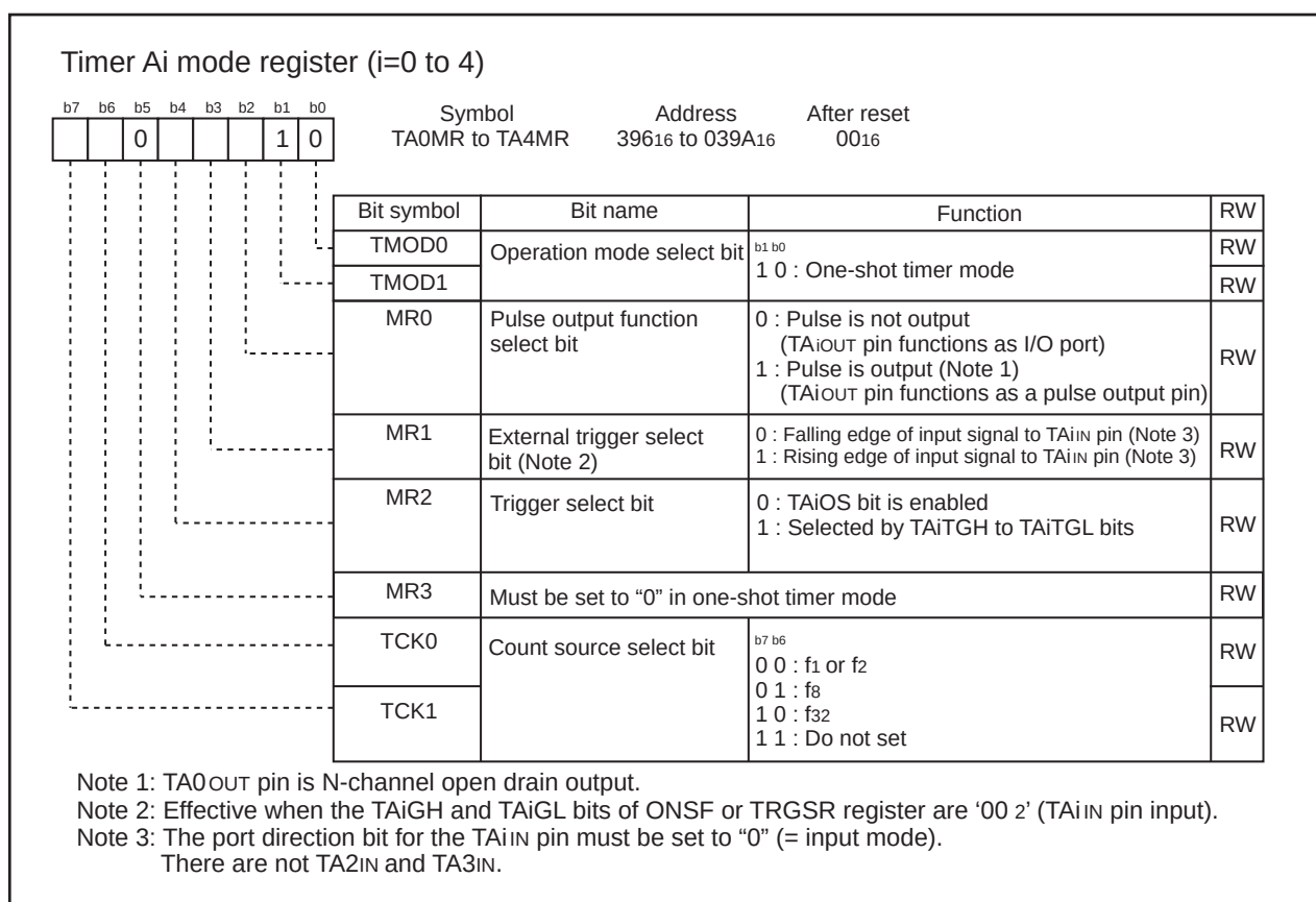
Figure 1.12.9. TAI i MR Register in One-shot Timer Mode
