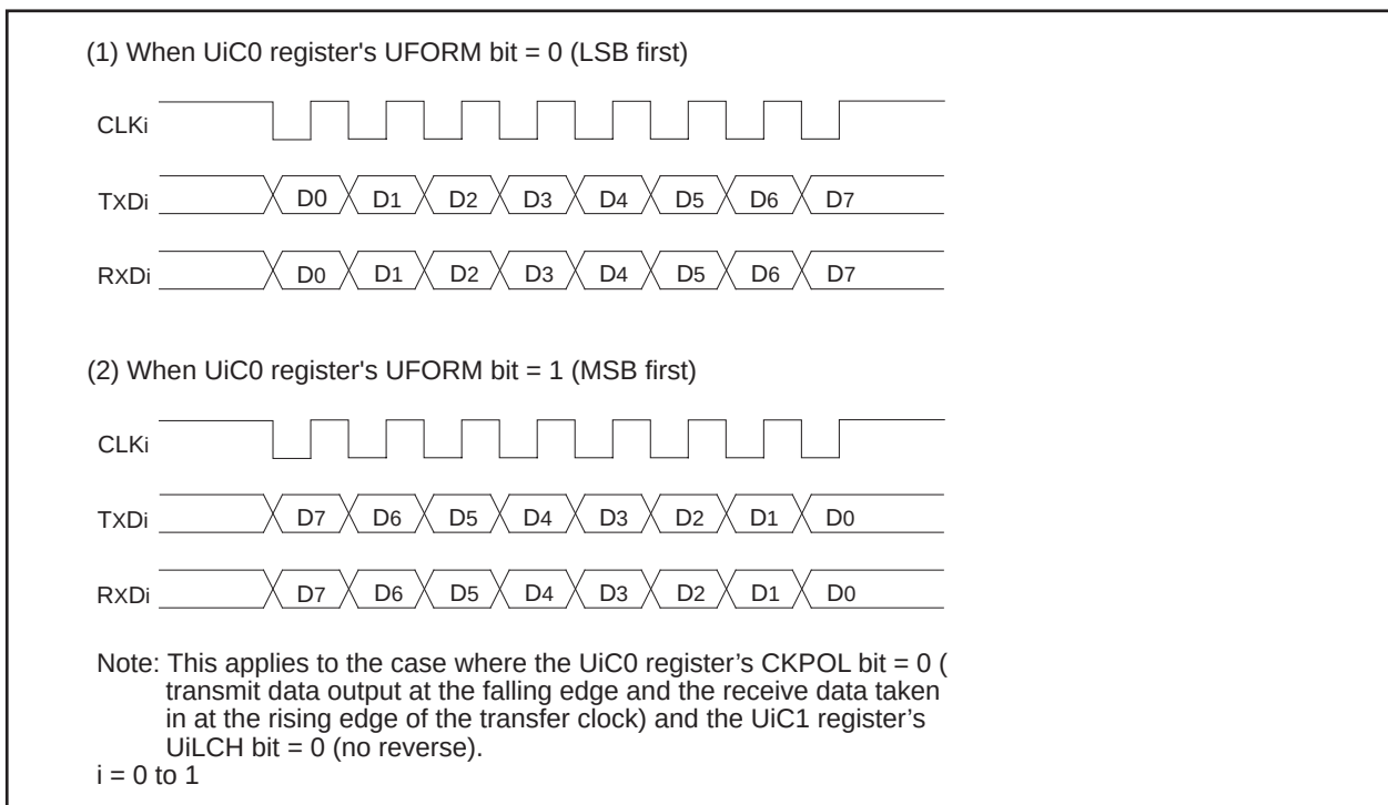
Figure 1.14.3. Transfer Format
