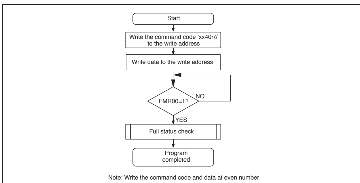
Figure 1.21.4. Program Command
