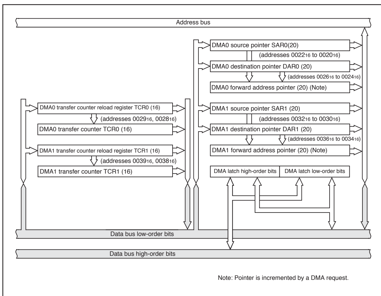
Figure 1.11.1. DMAC Block Diagram
