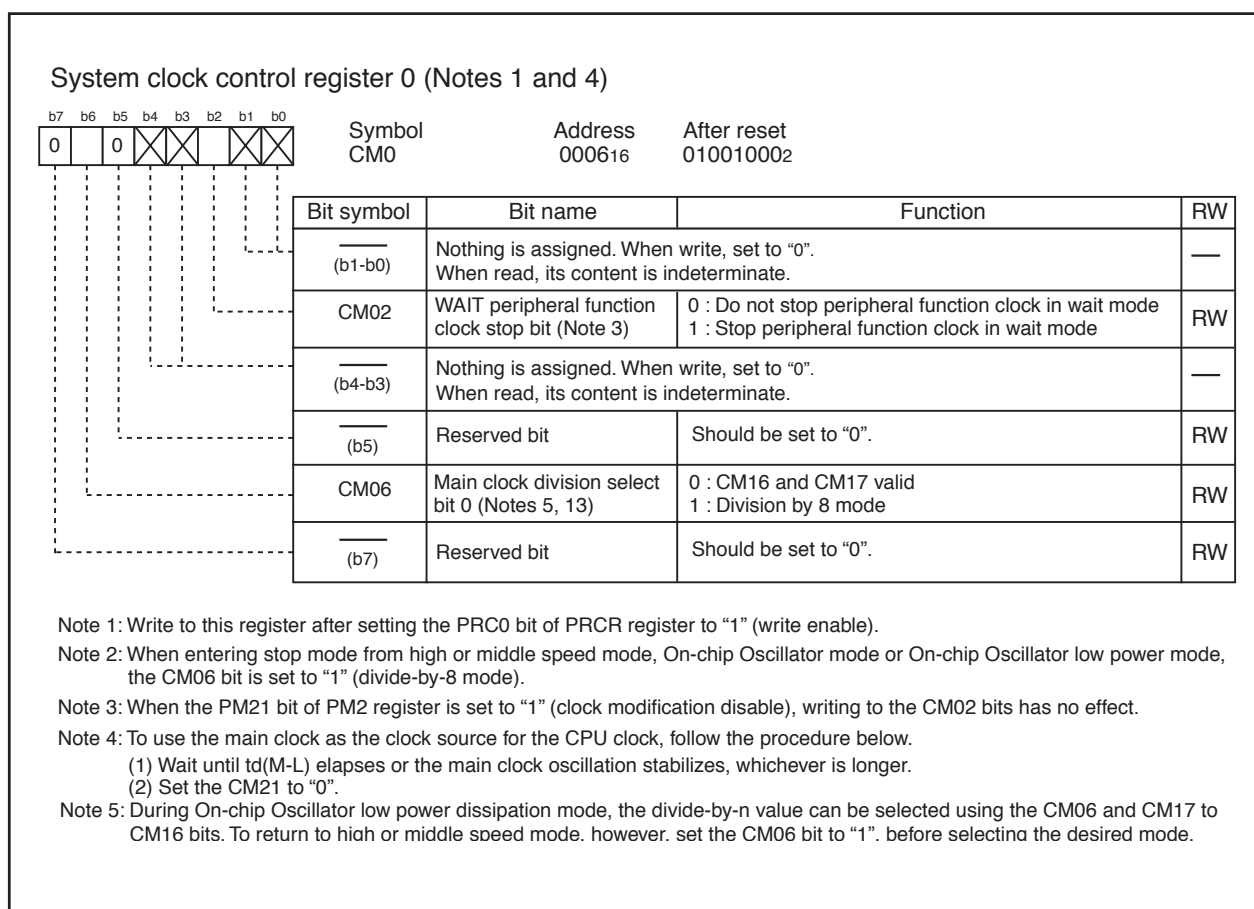
Figure 1.7.2. CM0 Register
