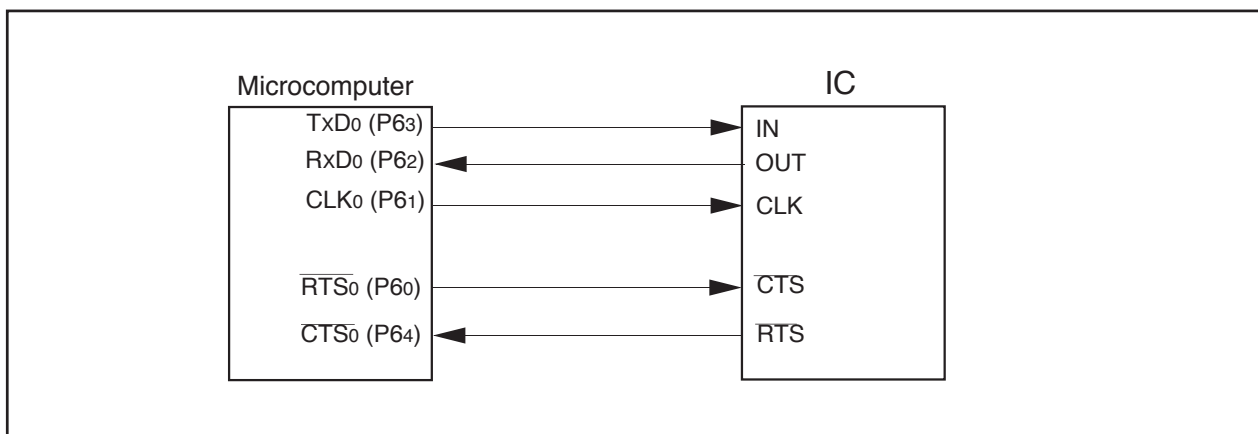
Figure 1.14.6. CTS/RTS Separate Function
