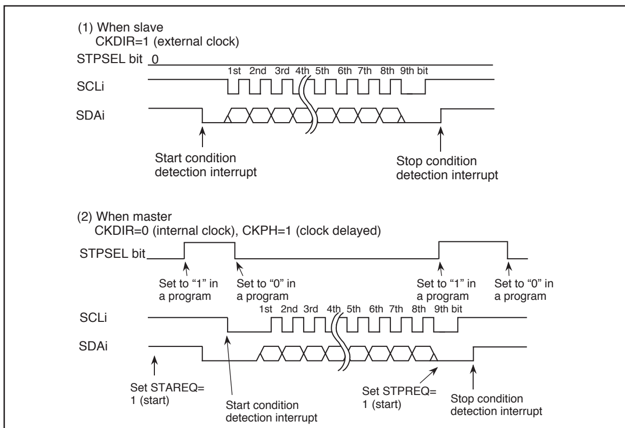
Figure 1.16.4. STSPSEL Bit Functions
