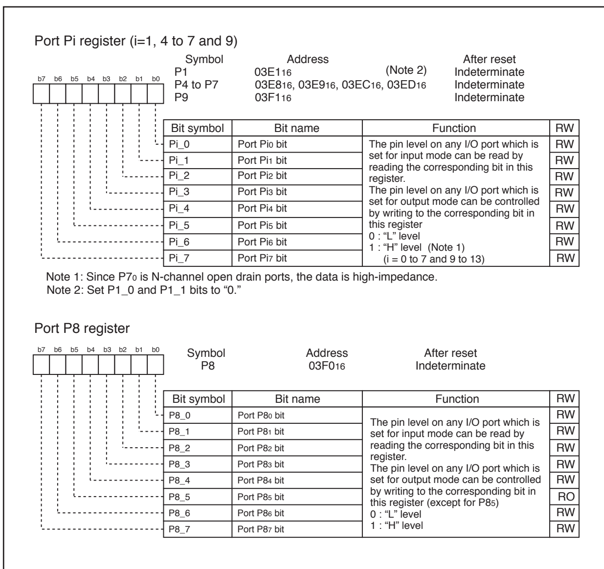
Figure 1.18.7. P1, P4 to P9
