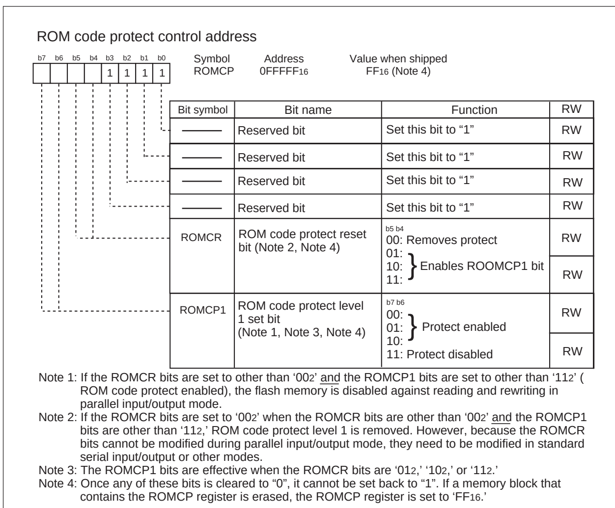
Figure 1.20.3. ROMCP Register
