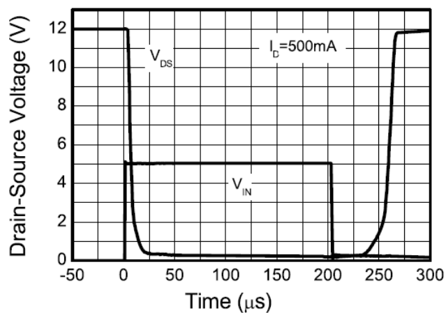
Switching Speed
