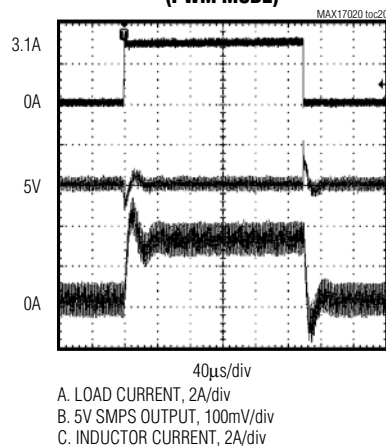
5V SMPS LOAD TRANSIENT (PWM MODE)
