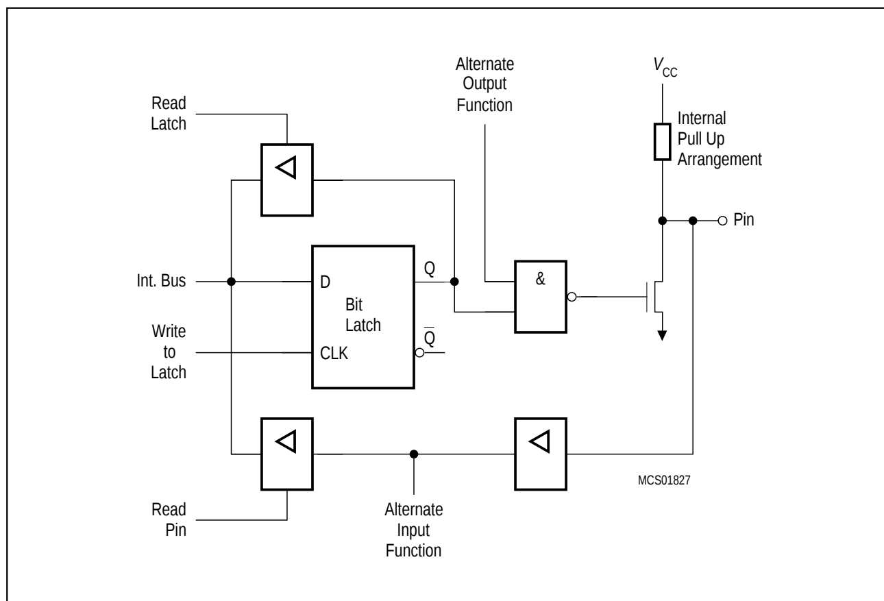
Figure 6-4 Ports 1 and 3
