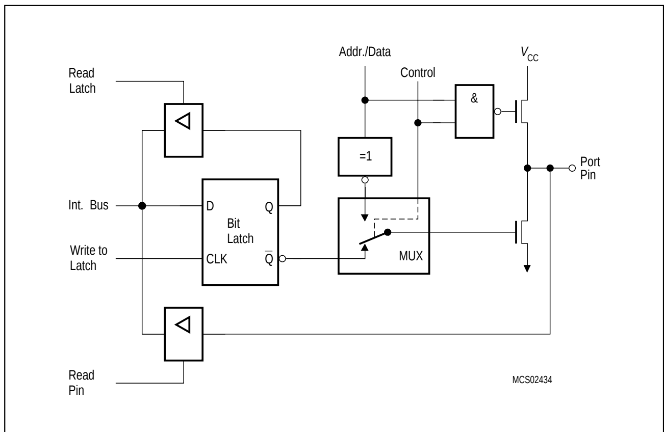
Figure 6-3 Port 0 Circuitry
