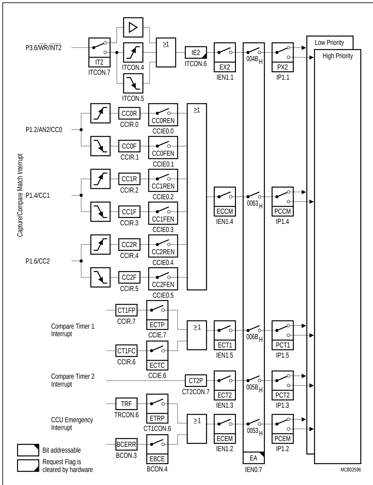
Figure 7-2 Interrupt Request Sources (Part 2)
