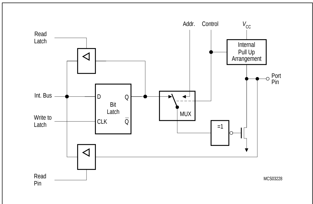
Figure 6-5 Port 2 Circuitry
