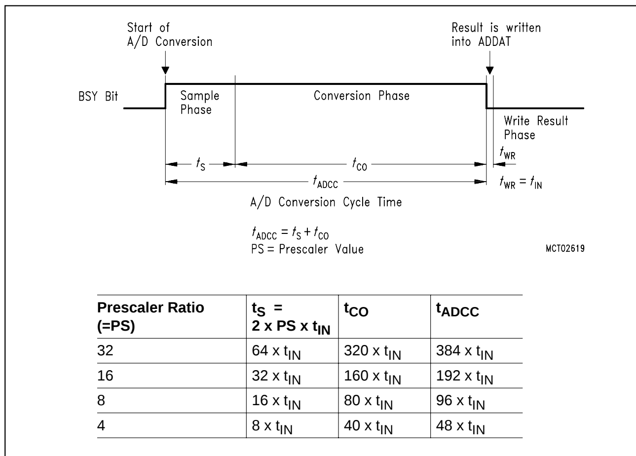
Figure 6-41 A/D Conversion Timing
