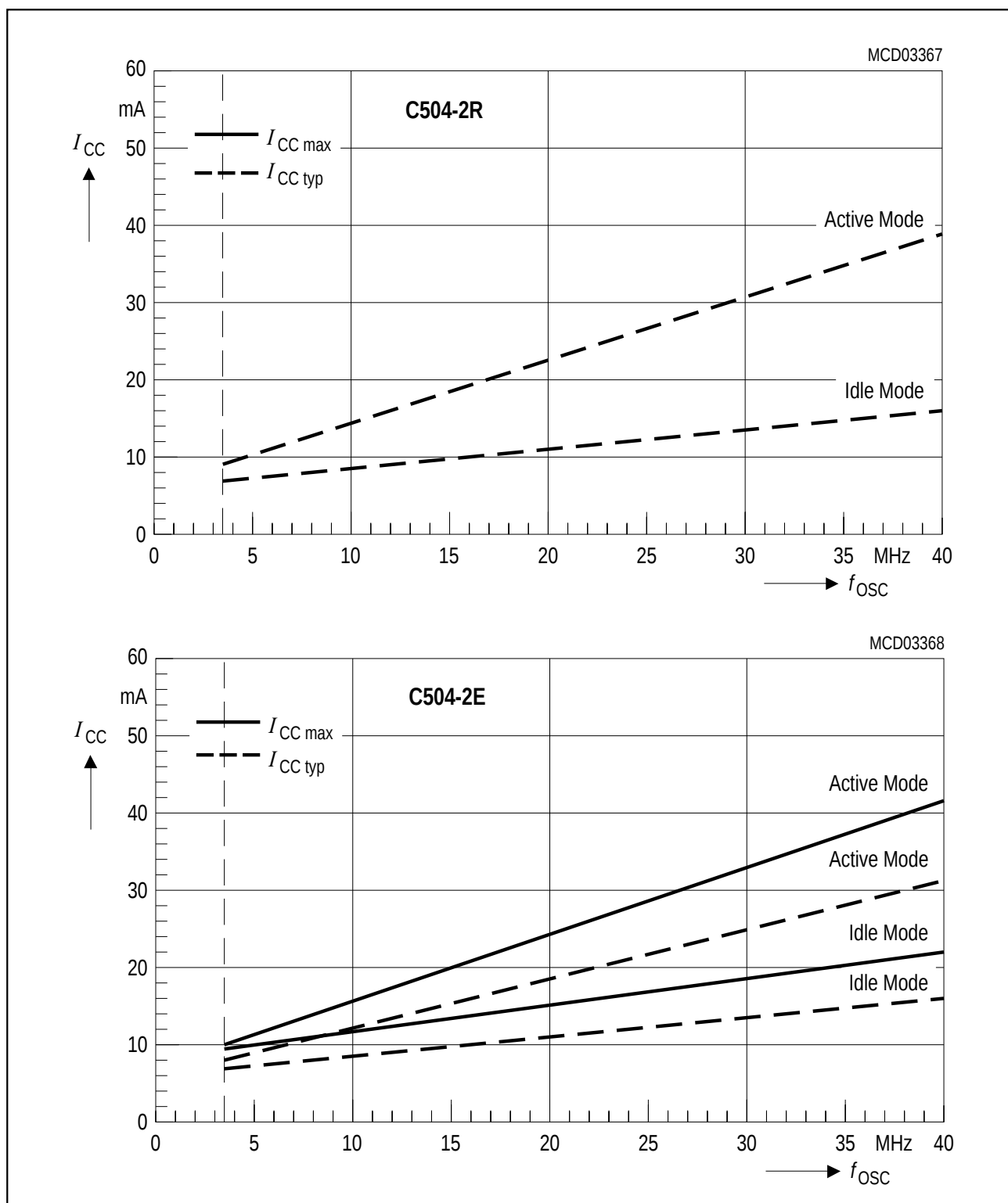
Figure 11-1 ICC Diagram
