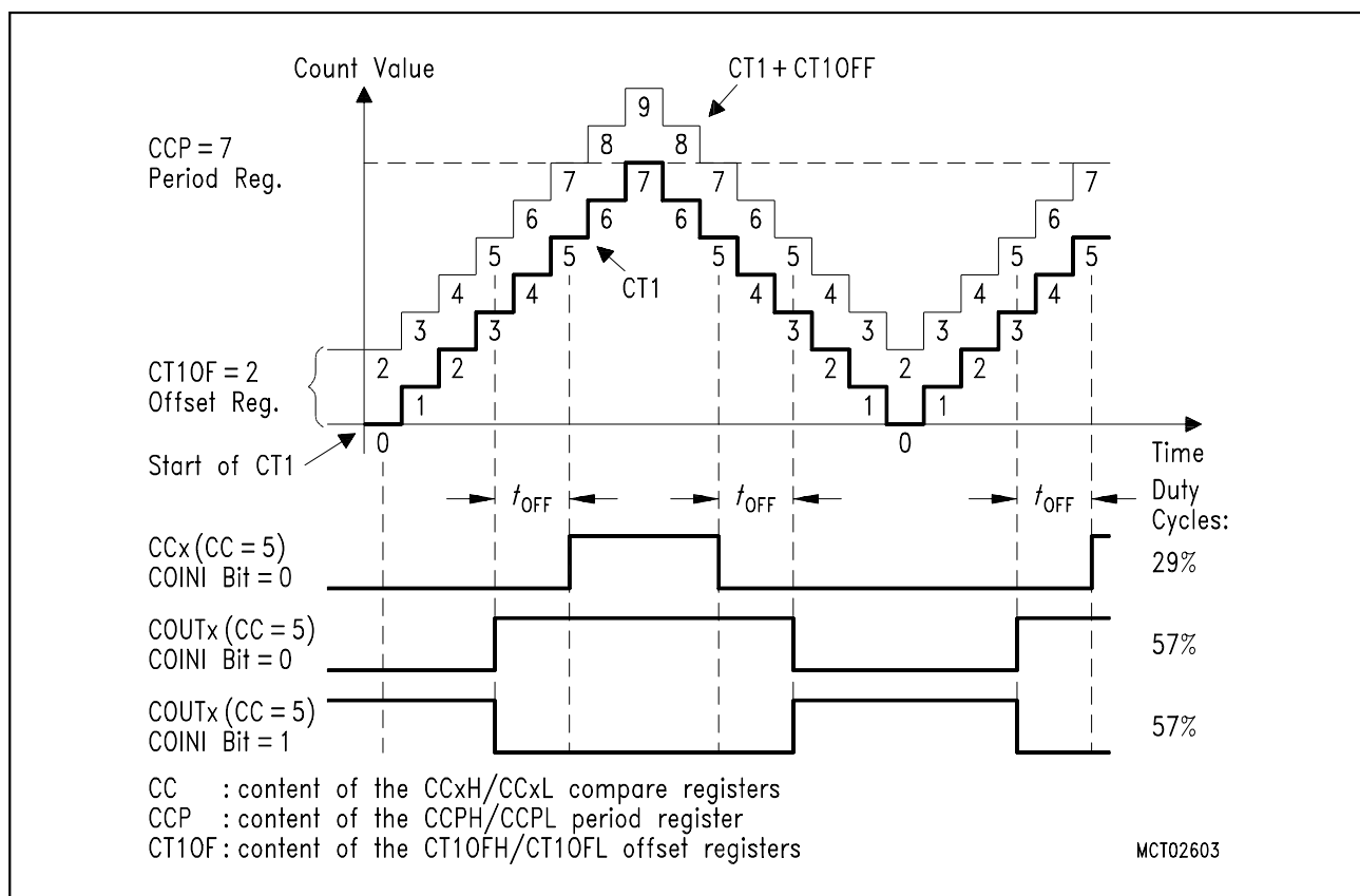
Figure 6-23 Compare Timer 1 with Offset # 0 (Dead Time) - Mode 1
