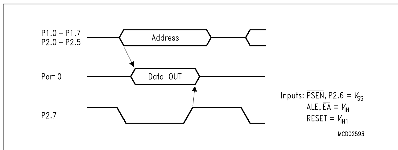
Figure 4-3 ROM Verification Mode 1
