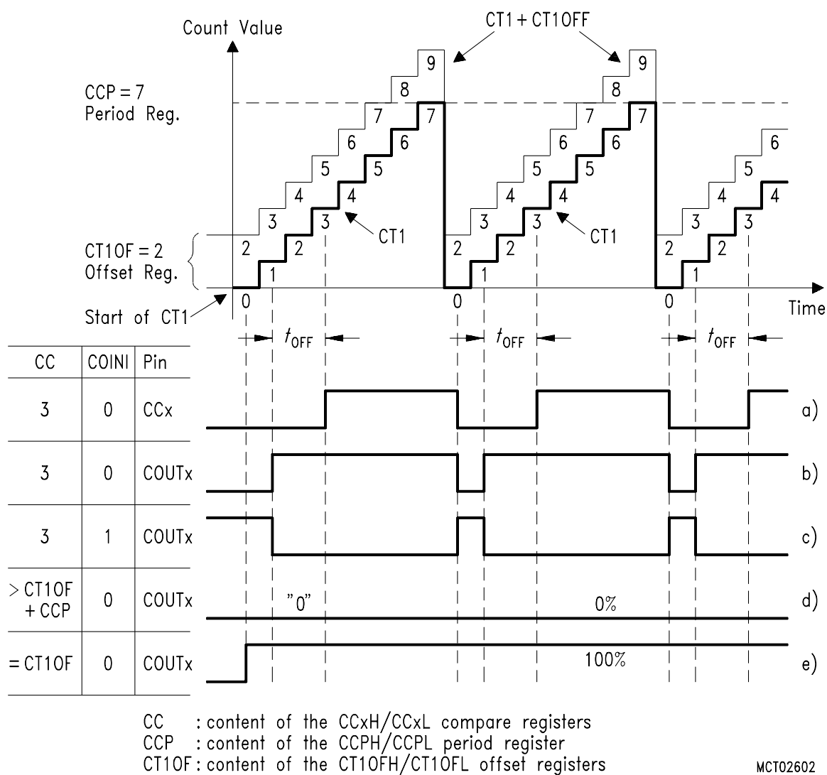
Figure 6-22 Compare Timer 1 with Offset not equal 0 - Mode 0
