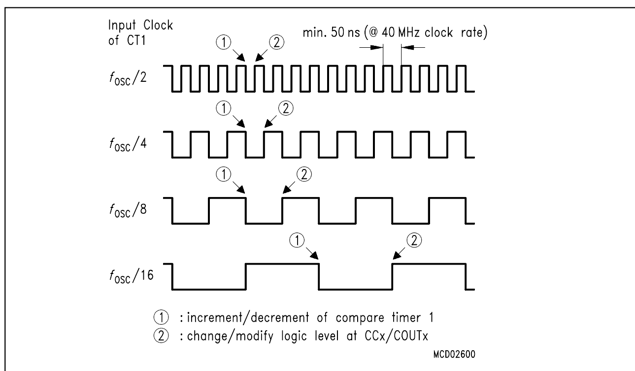
Figure 6-20 CAPCOM Unit Clocking Scheme
