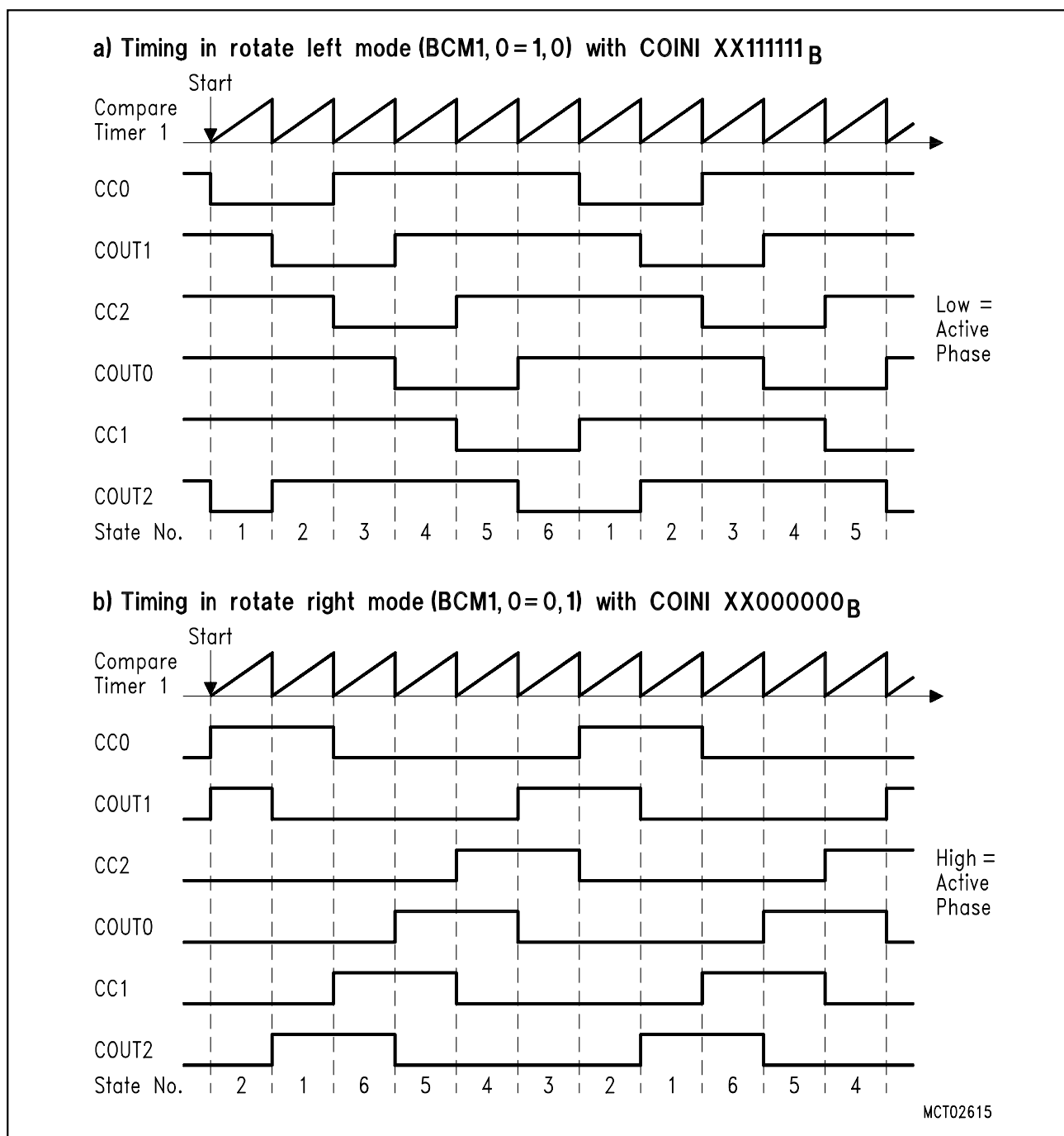
Figure 6-34 Basic Compare Timer 1 Controlled 6-Phase PWM Timing
