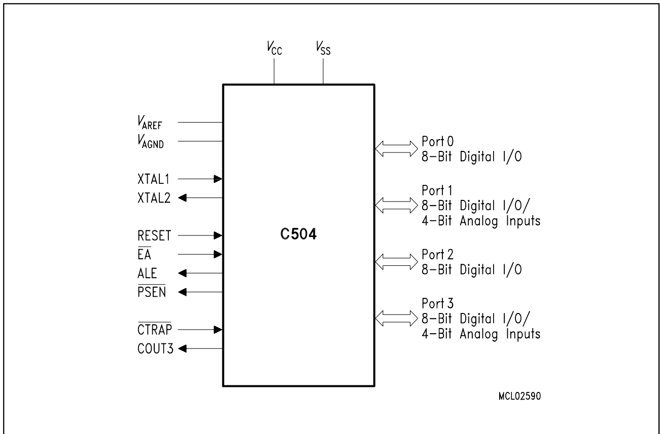
Figure 1-2 Logic Symbol
