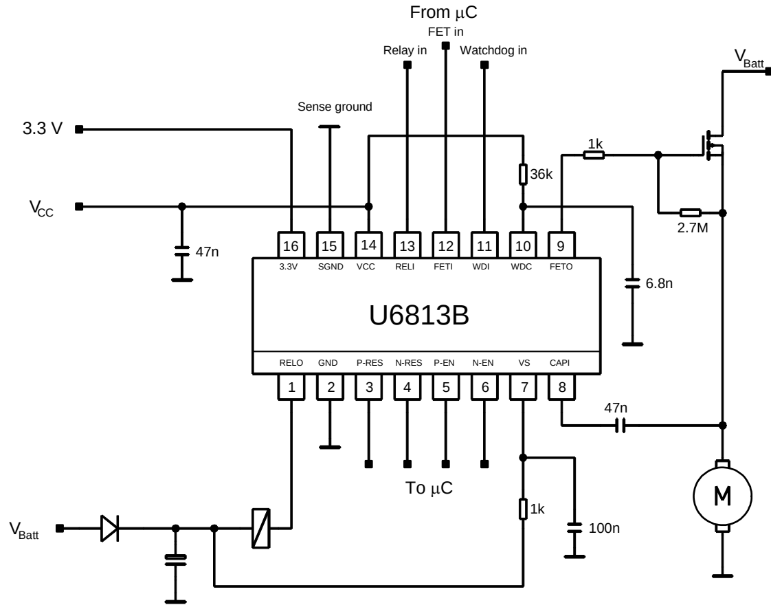
Figure 10. Application Circuit
