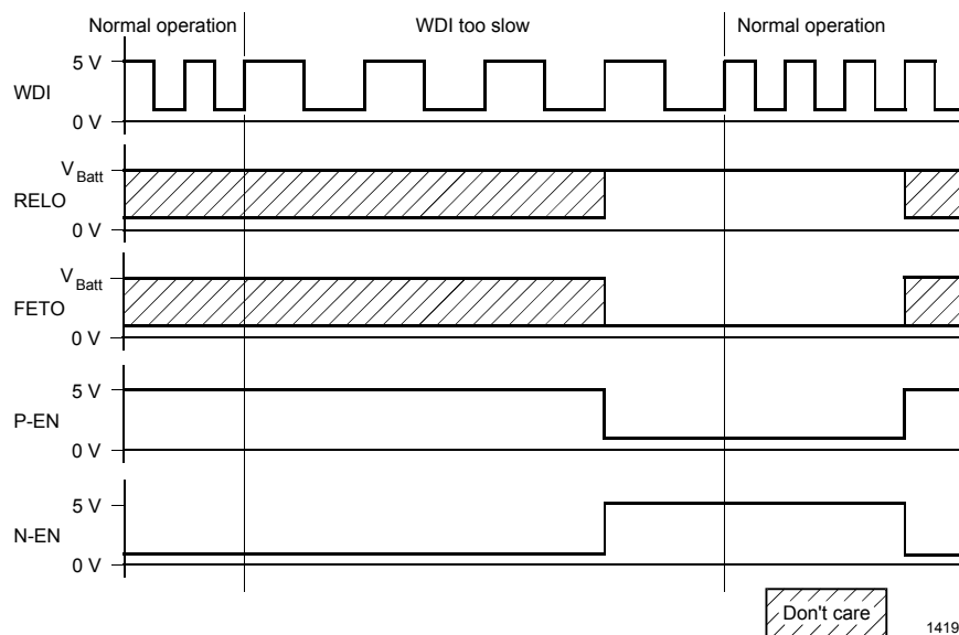
Figure 7. Watchdog in Too-slow Condition
