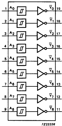
Fig.4 Functional diagram.
