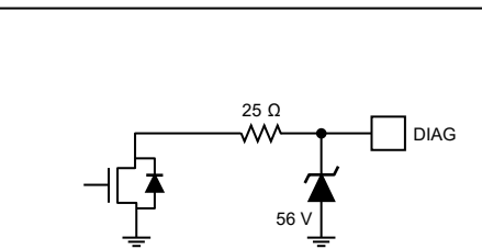
Figure 9g: DIAG Output
