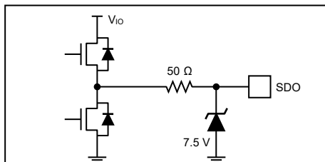
Figure 9f: SDO Output
