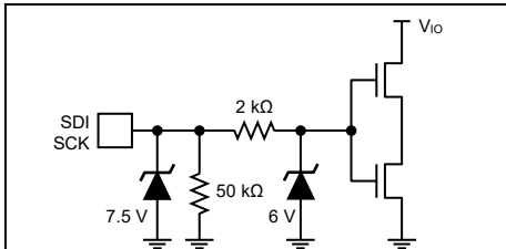
Figure 9c: SDI, SCK Inputs
