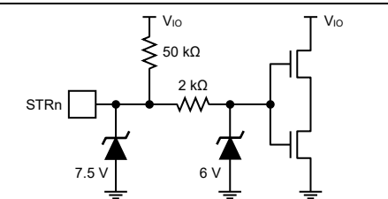
Figure 9d: STRn Inputs
