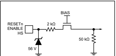
Figure 9e: RESETn, ENABLE, HS Inputs
