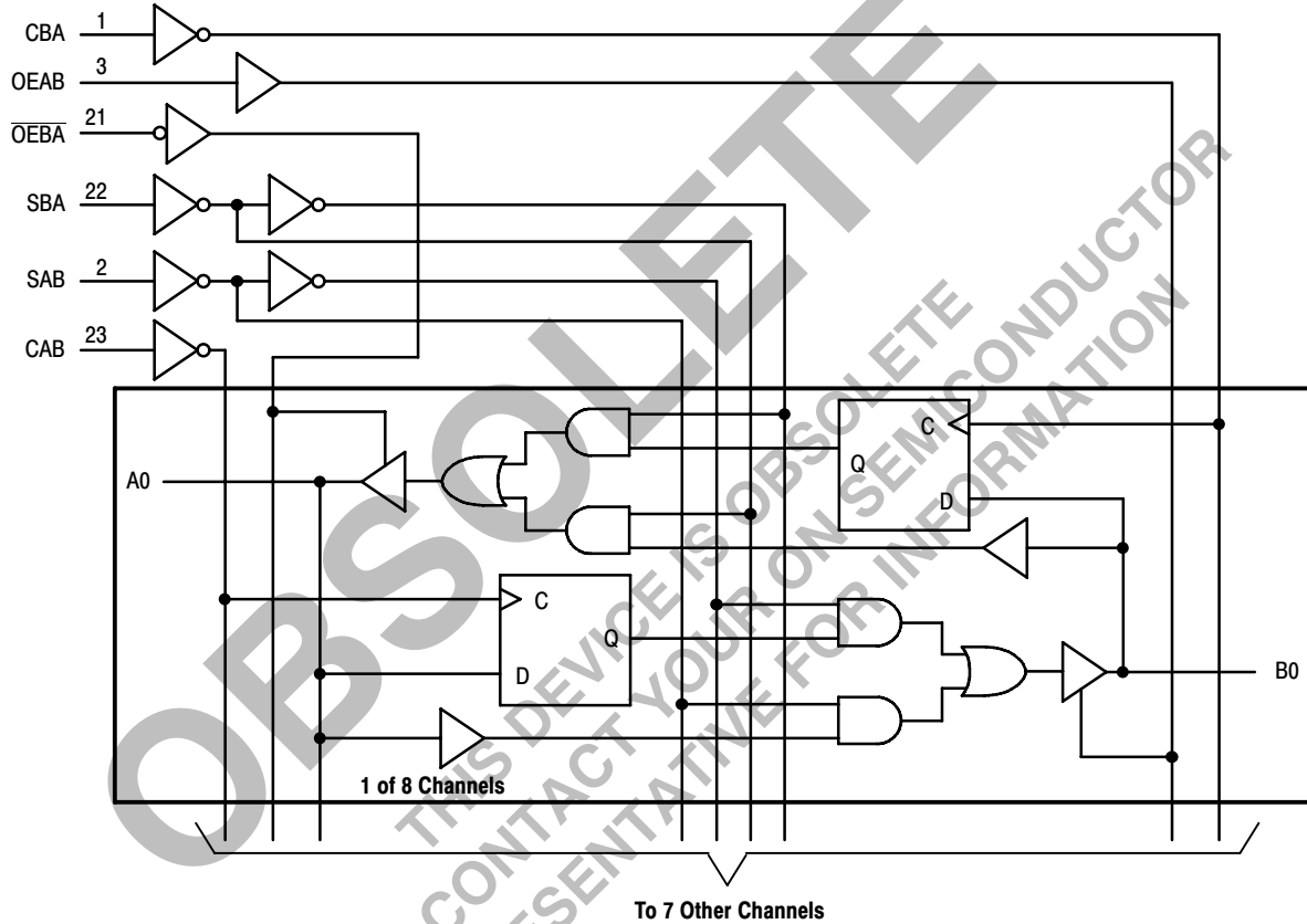
Figure 3. Logic Diagram
