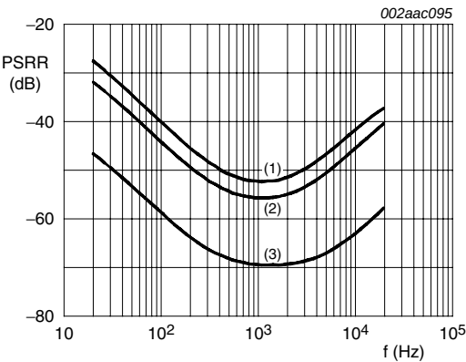
R_s = 0 \Omega ; V_{ripple} = 100 \text{ mV} . (1) G_v = 24 \text{ dB} . (2) G_v = 20 \text{ dB} . (3) G_v = 0 \text{ dB} .
