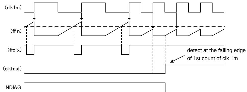
Fig.5-6c Timing chart of frequency monitoring (High frequency)
