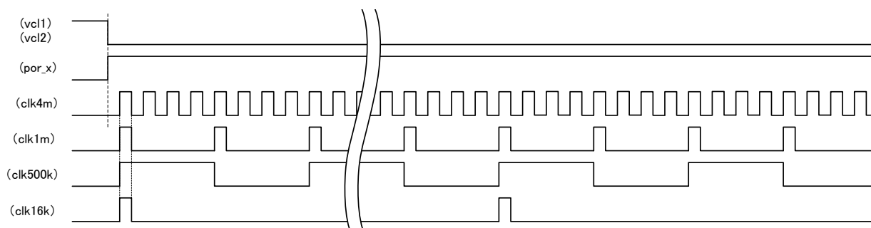
Fig.4-b Timing chart of divider
