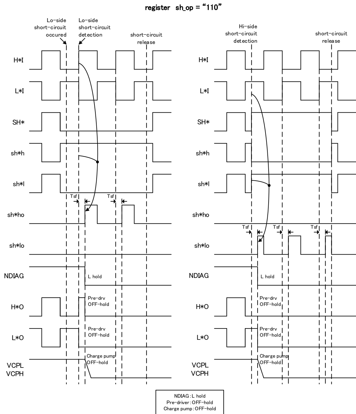
Fig.5-5f Timing chart of short-circuit detection (Register (sh_op) = "110")
