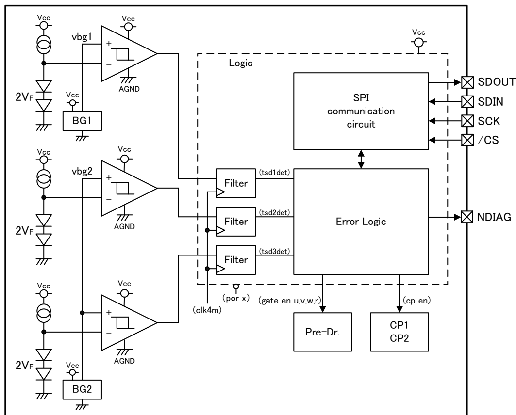
Fig.5-4a Over temperature detection Block Diagram
