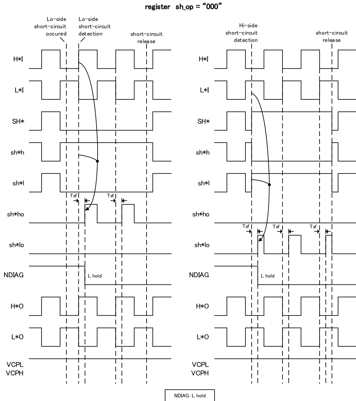
Fig.5-5b Timing chart of short-circuit detection (Register (sh_op) = "000")
