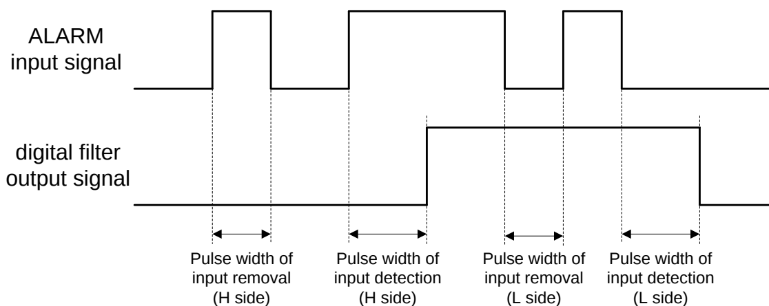
Fig.6-b Pulse width of input removal (with filter) and pulse width of input detection (with filter)
