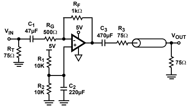
FIGURE 36. SINGLE SUPPLY INVERTING VIDEO LINE DRIVER
