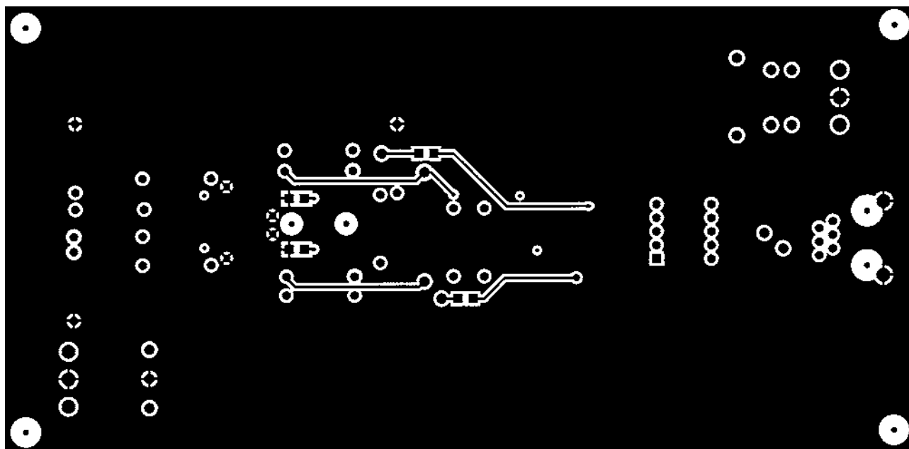
Figure 15. Layer 4—Secondary Side
