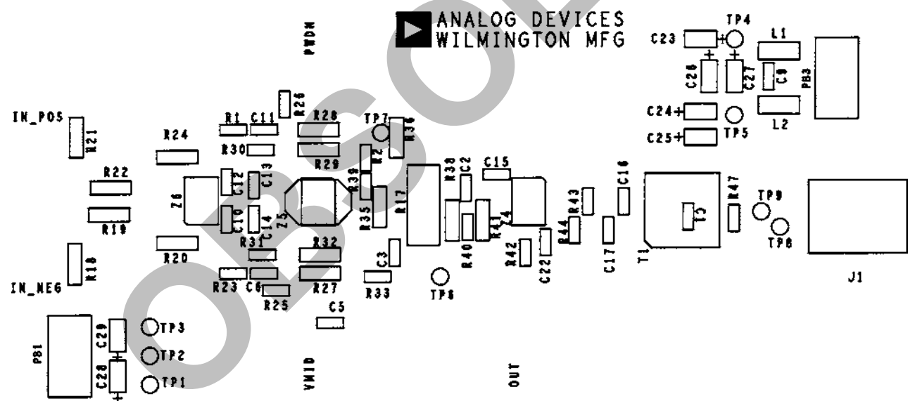
Figure 12. Silkscreen—Primary Side
