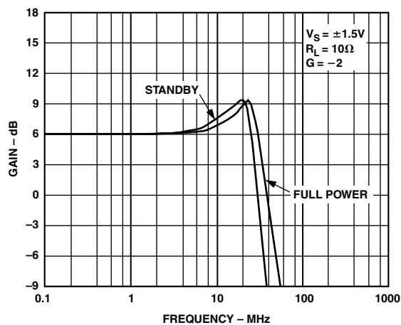
TPC 12. Small Signal Frequency Response
