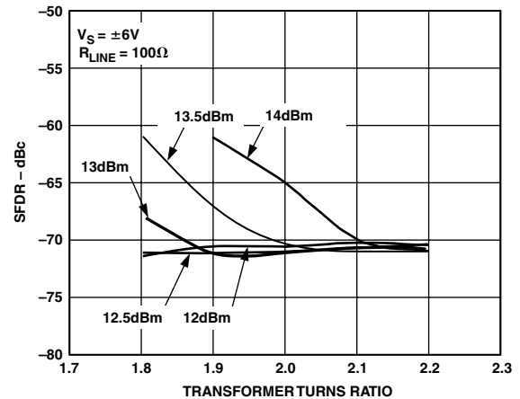
TPC 24. SFDR vs. Transformer Turns Ratio
