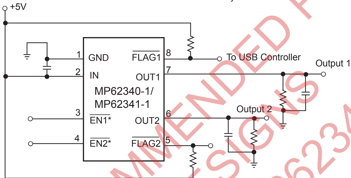
Figure 3—Application Circuit
