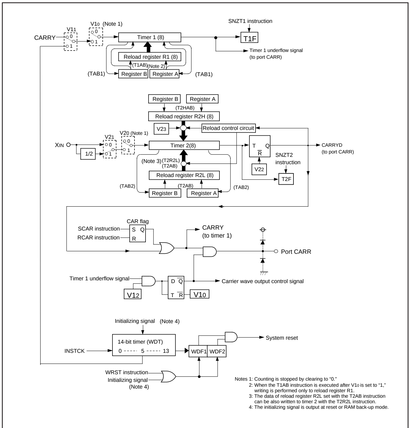
Fig. 13 Timers structure
