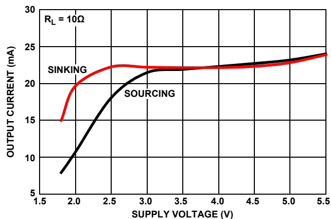
FIGURE 8. SHORT CIRCUIT CURRENT vs SUPPLY VOLTAGE
