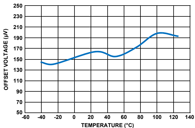
FIGURE 16. V_{OS} vs TEMPERATURE, V+ , GND = \pm 2.5V , V_{CM} = 0V
