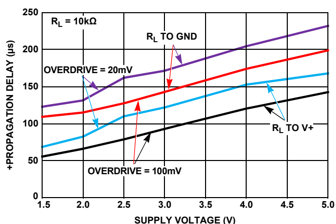
FIGURE 4. PROPAGATION DELAY vs SUPPLY VOLTAGE (RISING EDGE)
