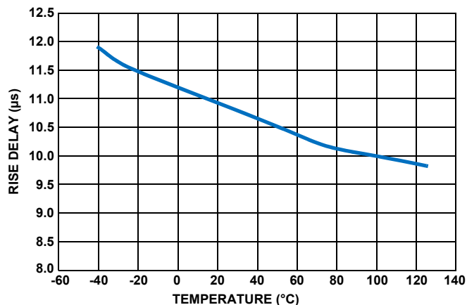
FIGURE 22. RISE TIME vs TEMPERATURE 20% TO 80%, V_+ = 5V
