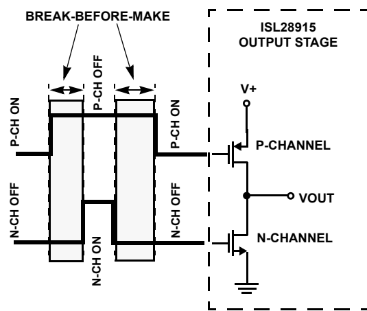
FIGURE 24. MAKE-BEFORE-BREAK ACTION OF THE OUTPUT STAGE
