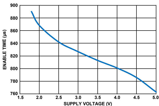
FIGURE 10. ENABLE TO OUTPUT DELAY TIME vs SUPPLY VOLTAGE
