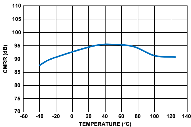
FIGURE 17. CMRR vs TEMPERATURE, V_{CM} = 0.5V TO 3.5 , V+ , GND = \pm 2.5V
