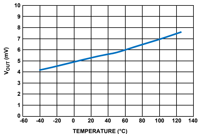
FIGURE 19. V_{OUT} LOW vs TEMPERATURE, V_+ , GND = \pm 2.5V , R_L = 10k
