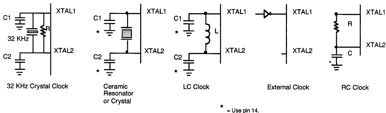
Figure 16. Oscillator Configuration
