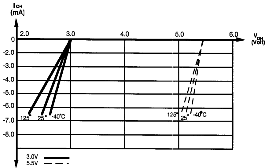
Figure 42. Typical I_{OH} vs. V_{OH}
