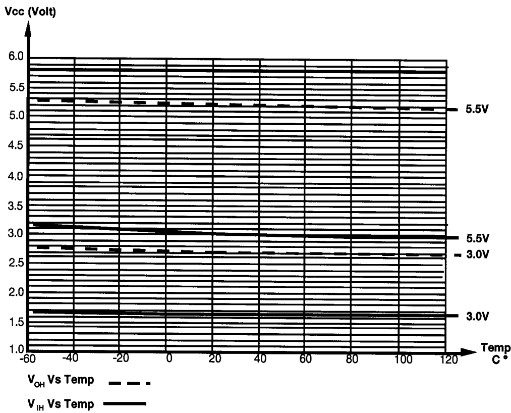
Figure 41. V_{IH} , V_{OH} vs. Temperature
