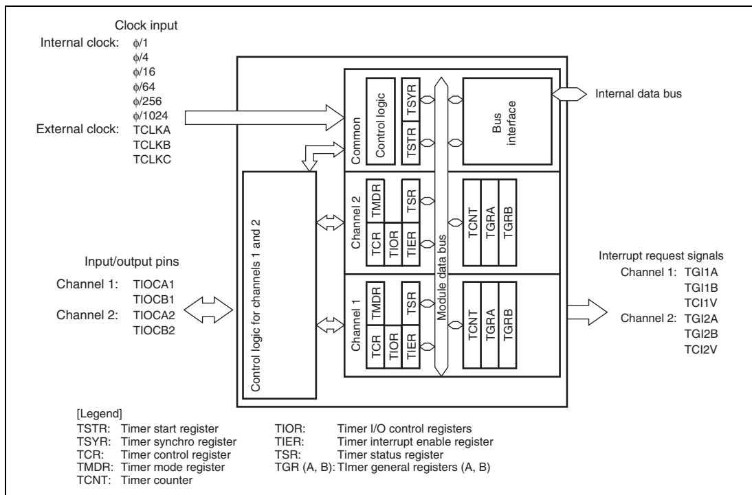
Figure 14.1 Block Diagram of TPU
