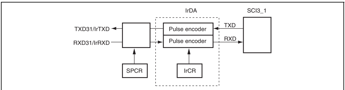
Figure 17.19 IrDA Block Diagram
