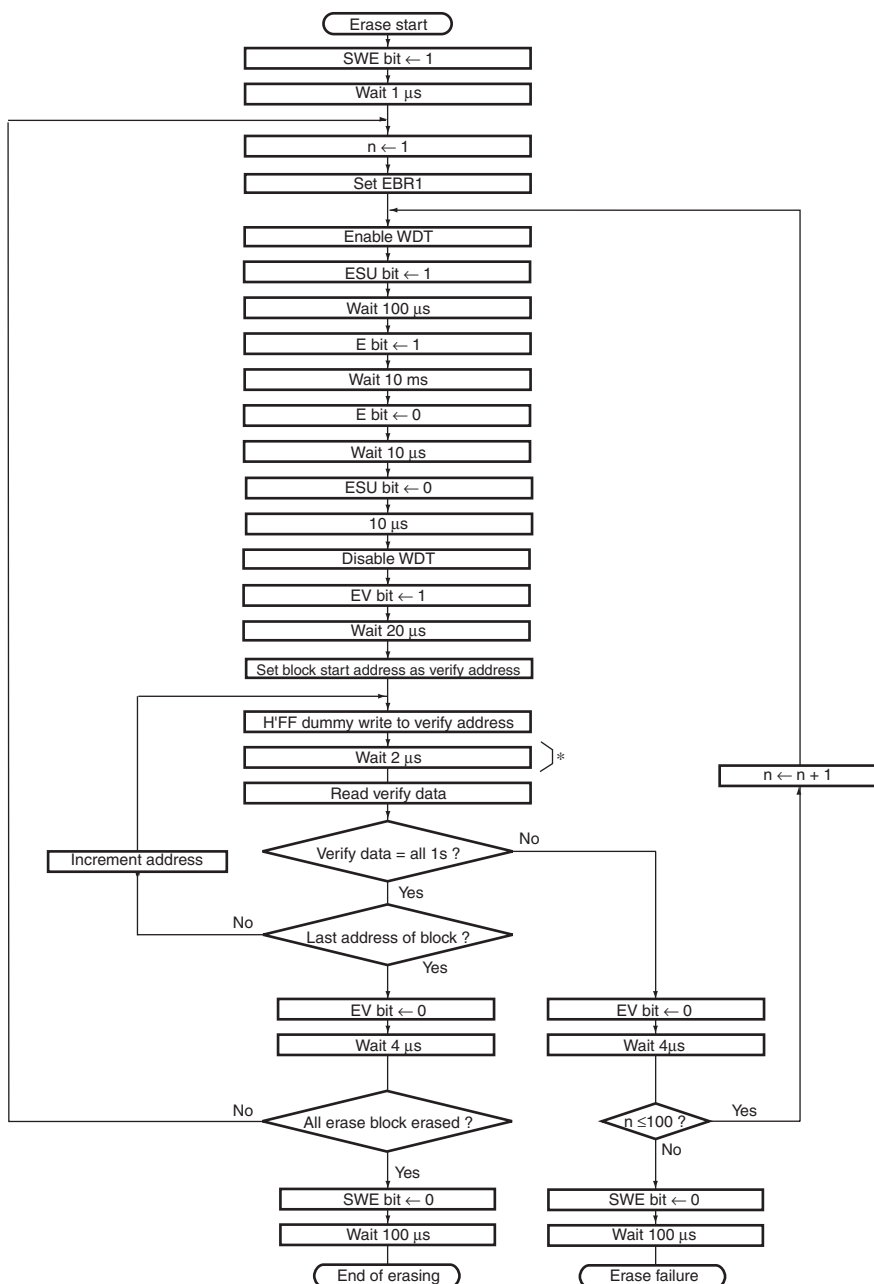
Figure 7.5 Erase/Erase-Verify Flowchart
