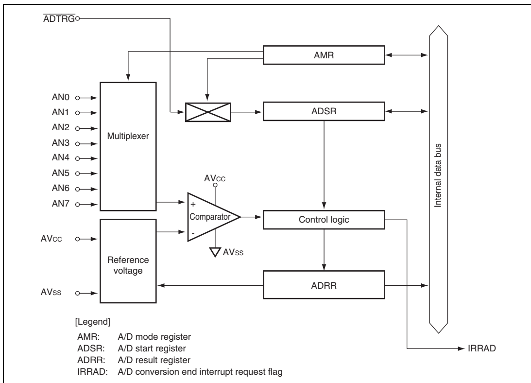
Figure 20.1 Block Diagram of A/D Converter
