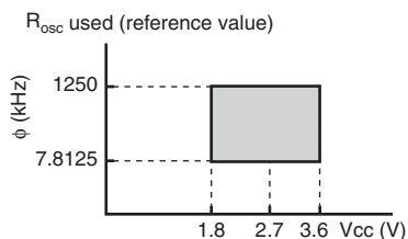
Figure 25.11 Power Supply Voltage and Operating Frequency Range (2)
