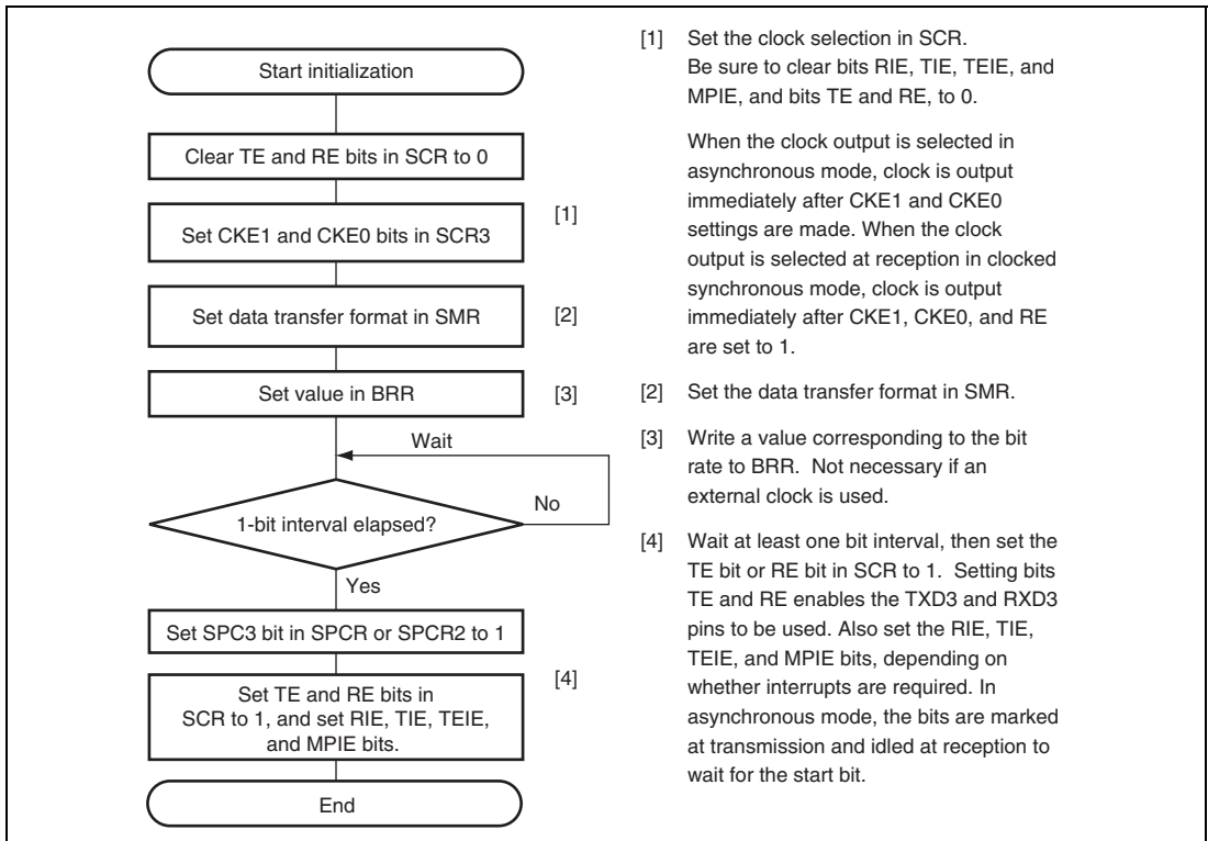
Figure 17.4 Sample SCI3 Initialization Flowchart
