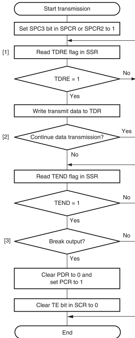
Figure 17.6 Sample Serial Transmission Flowchart (Asynchronous Mode)
