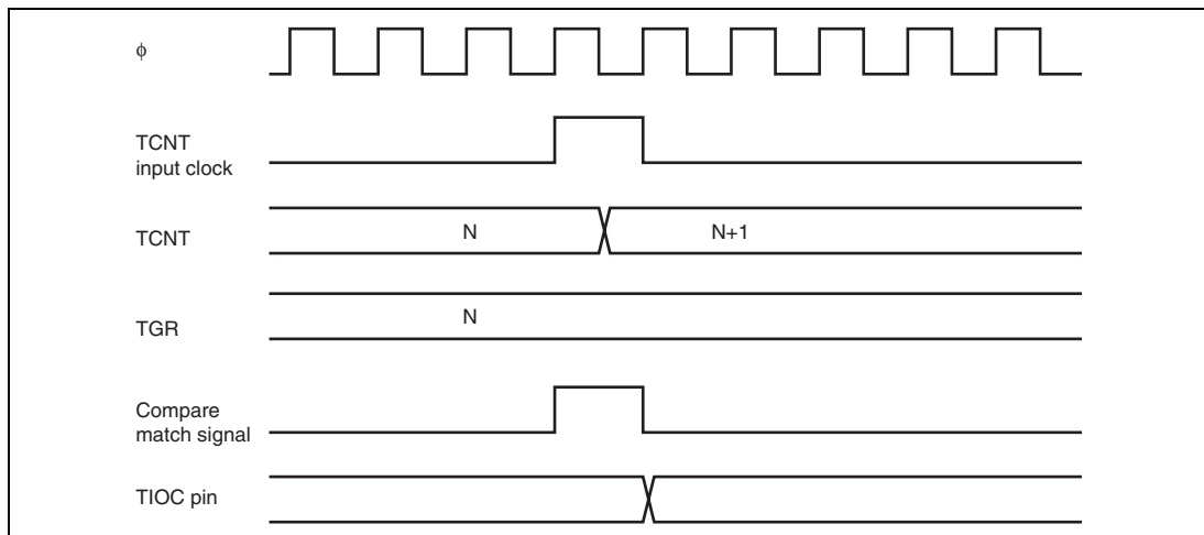
Figure 14.23 Output Compare Output Timing
