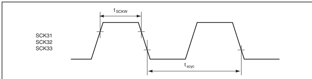
Figure 25.17 SCK3 Input Clock Timing
