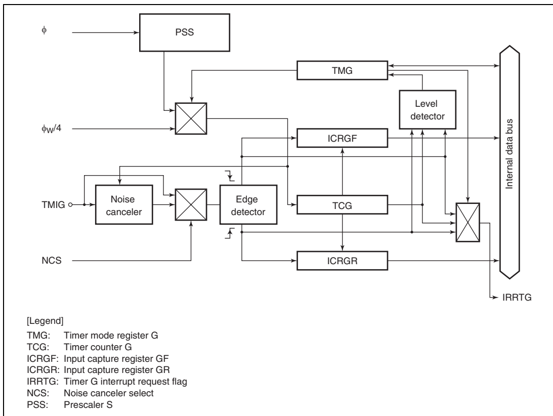
Figure 13.1 Block Diagram of Timer G
