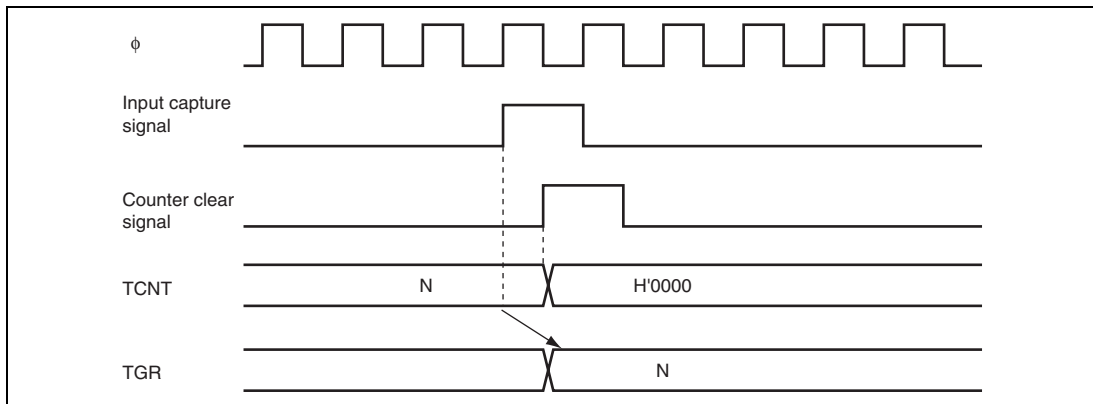
Figure 14.26 Counter Clear Timing (Input Capture)
