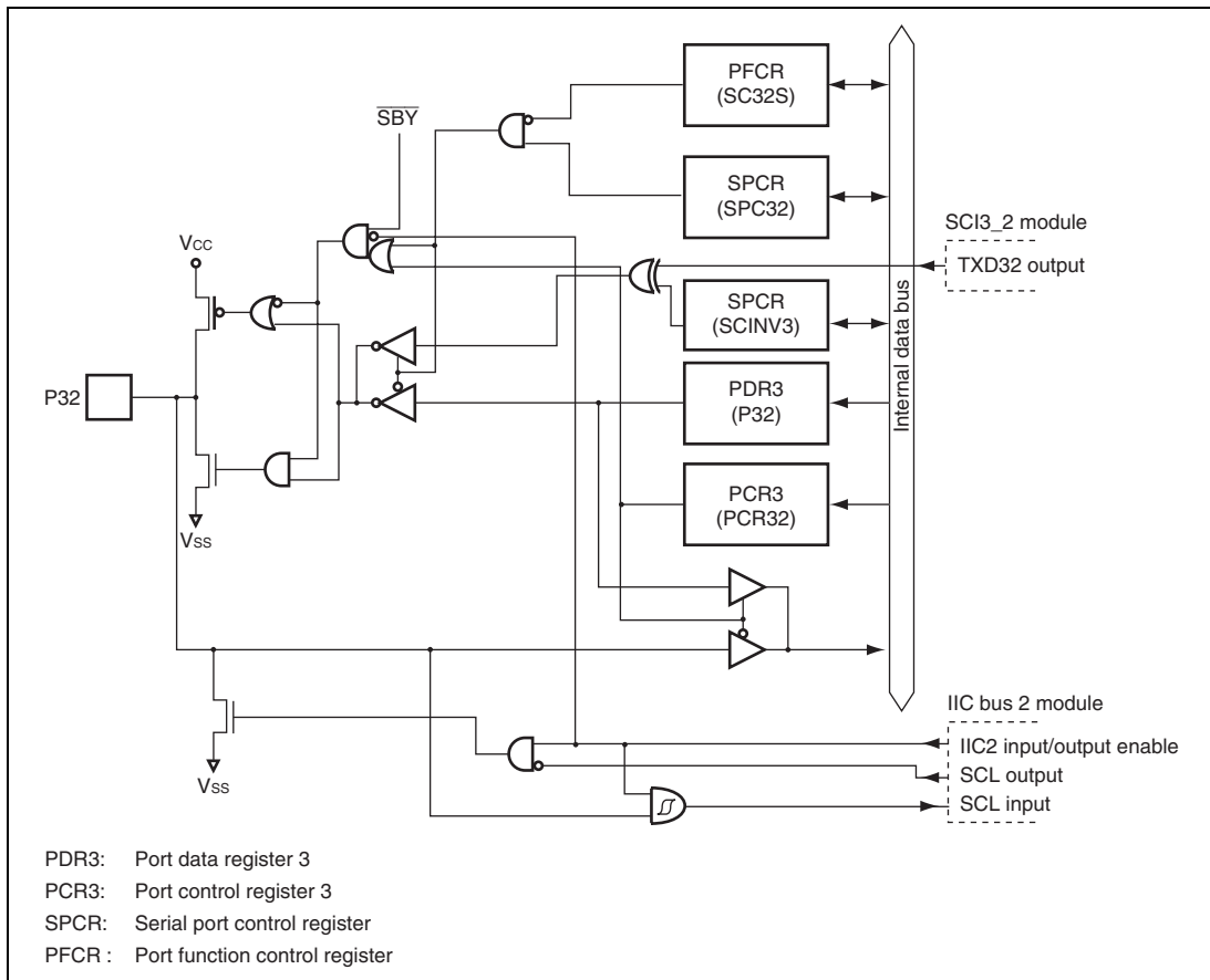
Figure B.2 (e) Port 3 Block Diagram (P32)
