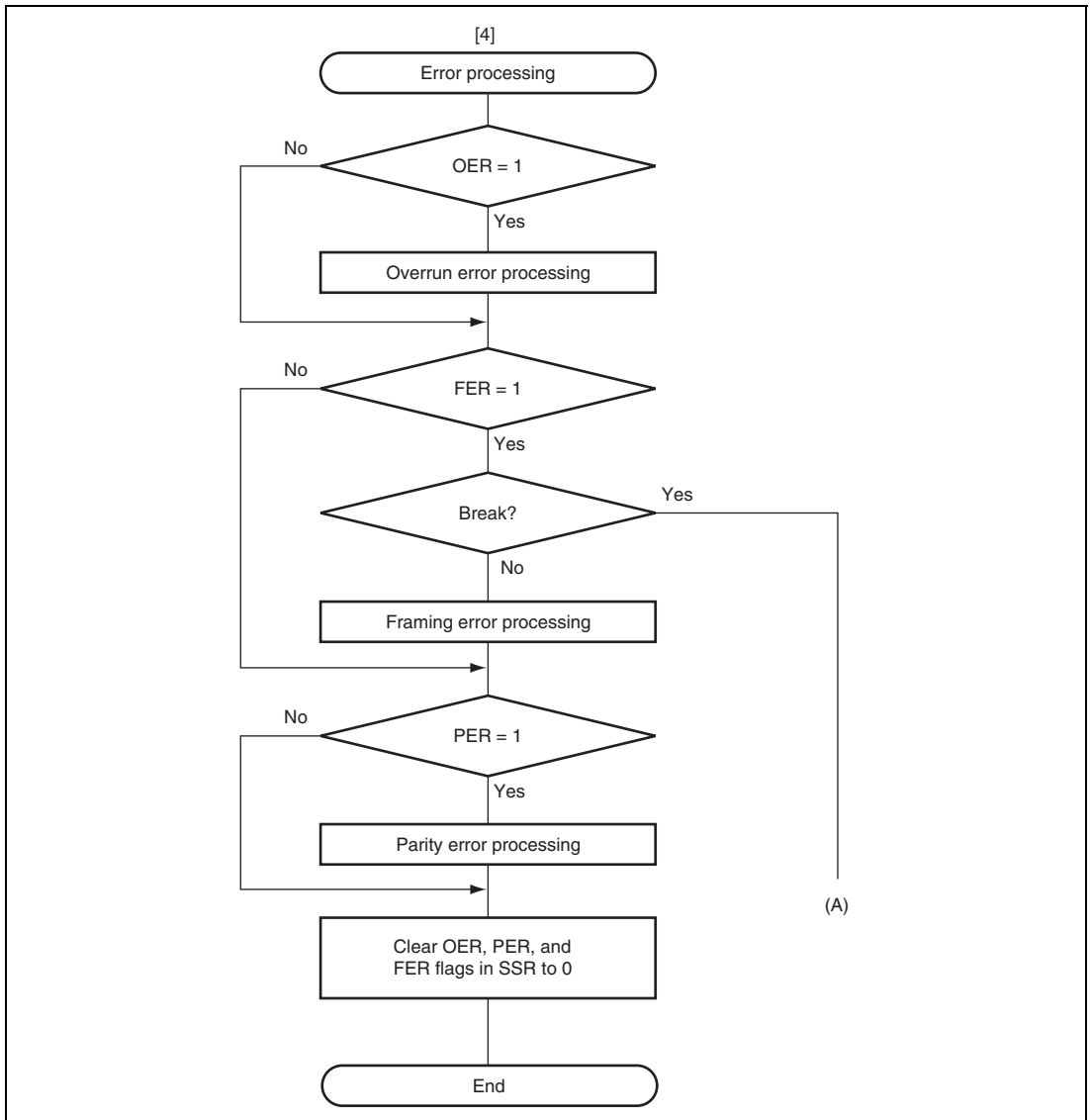
Figure 17.8 Sample Serial Data Reception Flowchart (Asynchronous Mode) (2)
