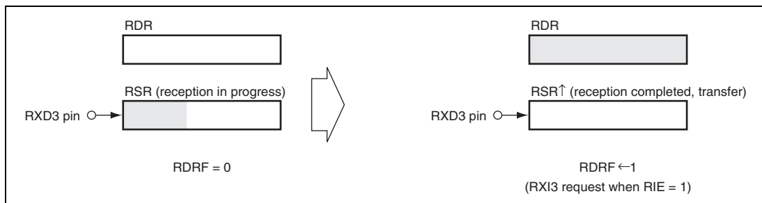
Figure 17.21 (a) RDRF Setting and RXI3 Interrupt
