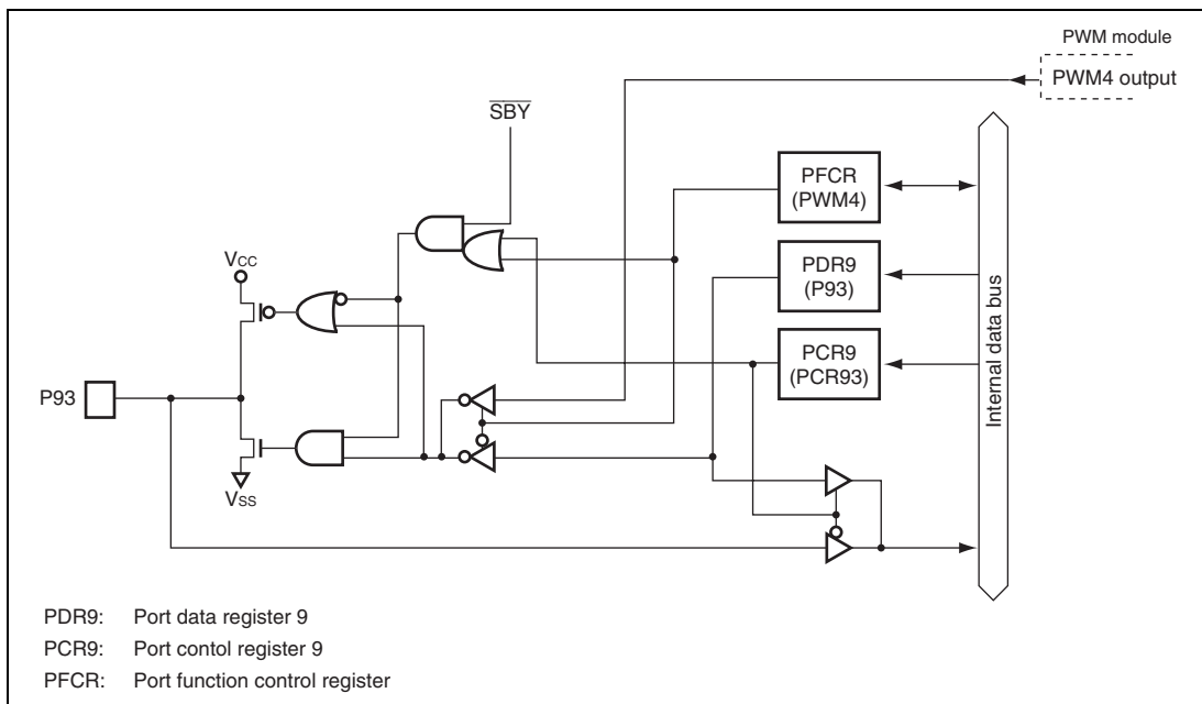
Figure B.8 (a) Port 9 Block Diagram (P93)
