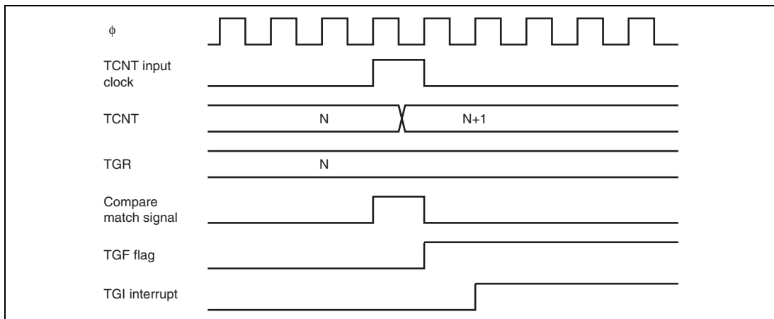
Figure 14.27 TGI Interrupt Timing (Compare Match)
