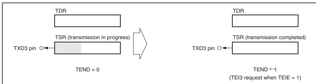
Figure 17.21 (c) TEND Setting and TEI3 Interrupt
