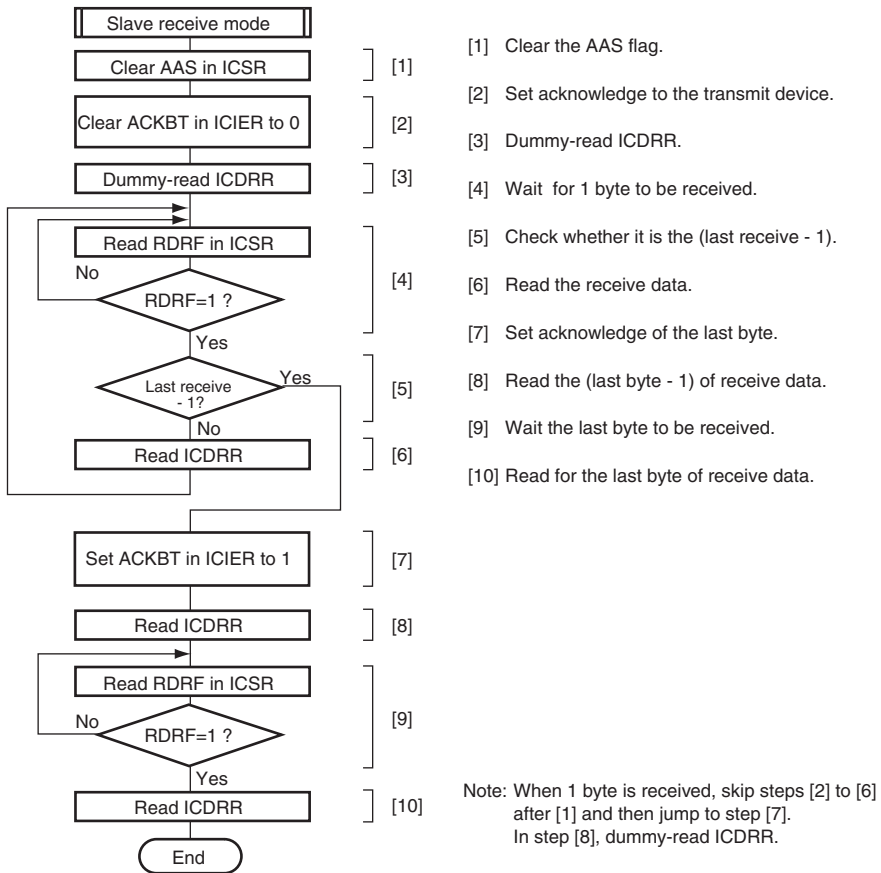
Figure 21.20 Sample Flowchart for Slave Receive Mode
