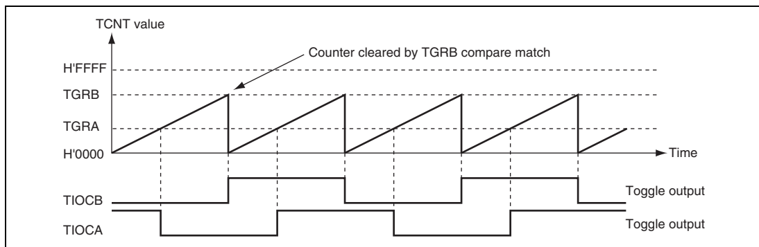
Figure 14.10 Example of Toggle Output Operation
