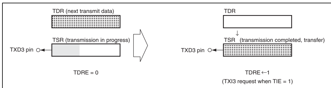
Figure 17.21 (b) TDRE Setting and TXI3 Interrupt
