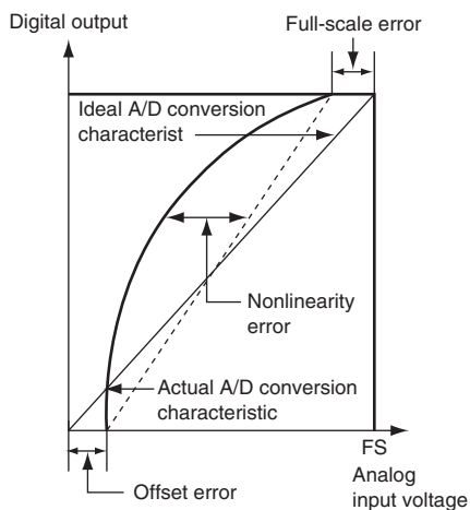
Figure 20.7 A/D Conversion Accuracy Definitions (2)
