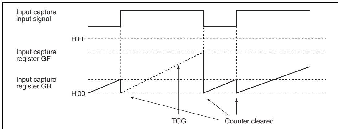
Figure 13.9 Timer G Application Example
