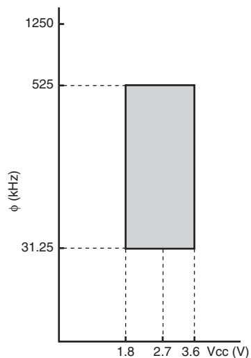
Figure 25.4 Power Supply Voltage and Operating Frequency Range (2)
