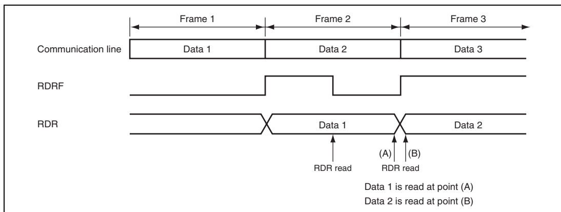
Figure 17.23 Relation between RDR Read Timing and Data
