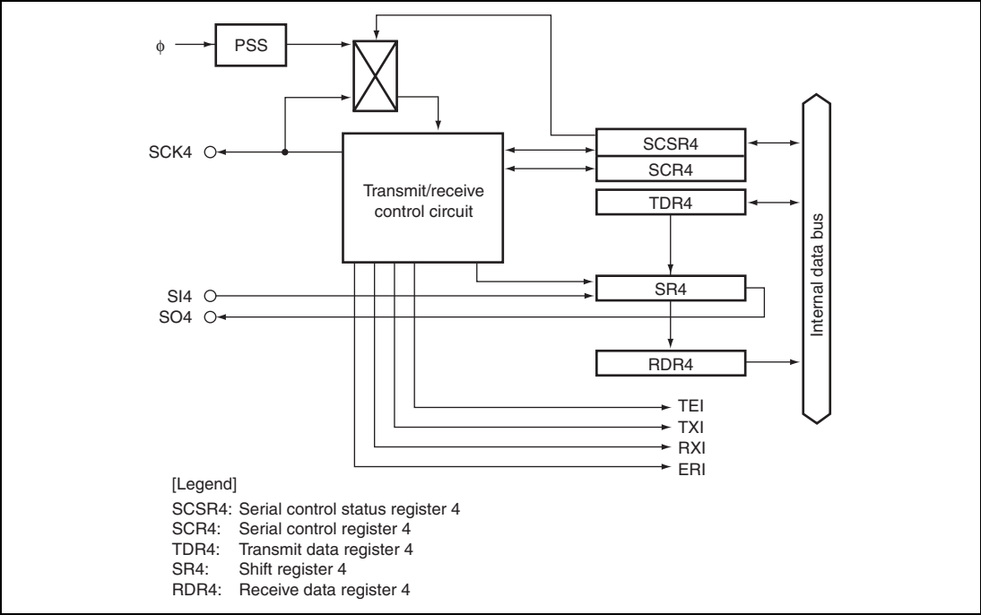
Figure 18.1 Block Diagram of SCI4
