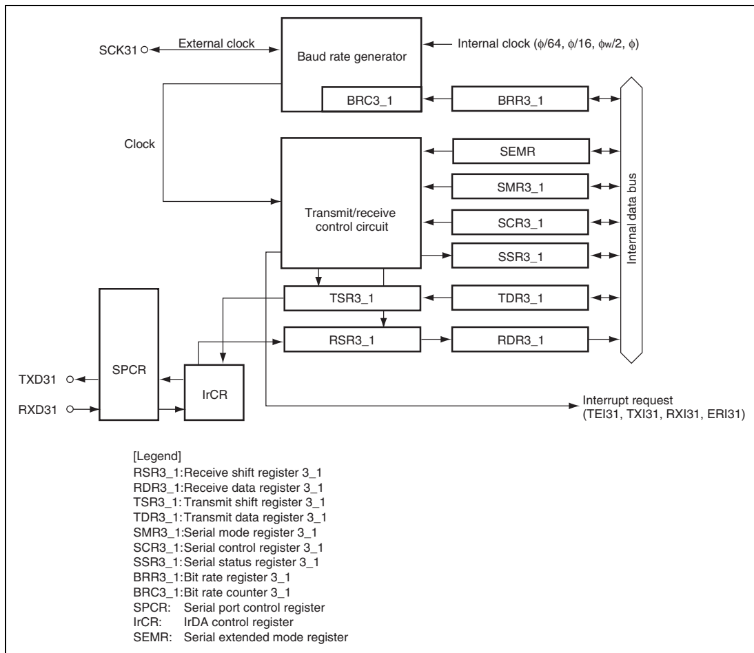
Figure 17.1 (1) Block Diagram of SCI3_1
