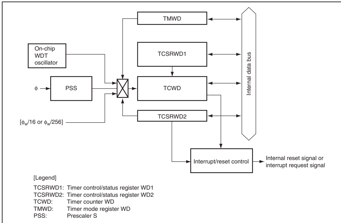
Figure 16.1 Block Diagram of Watchdog Timer
