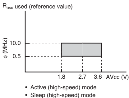
Figure 25.7 Analog Power Supply Voltage and Operating Frequency Range of A/D Converter (2)
