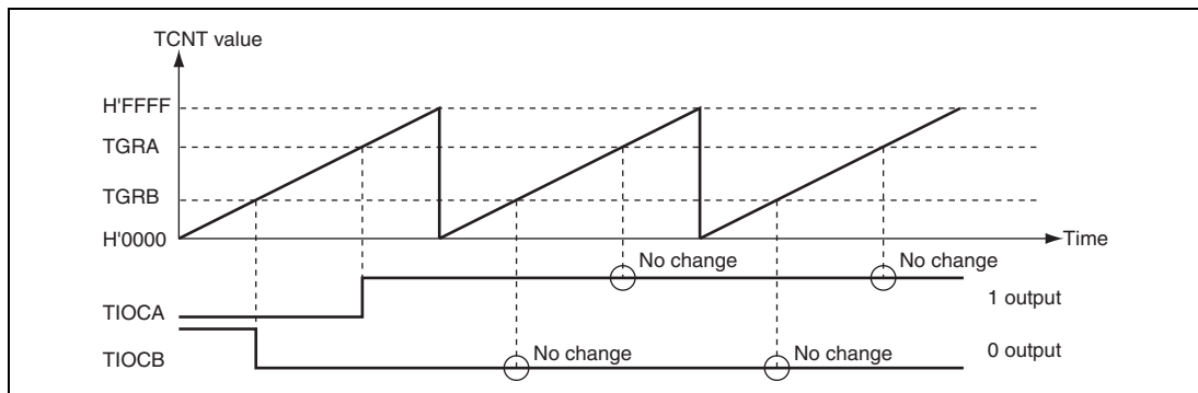
Figure 14.9 Example of 0 Output/1 Output Operation
