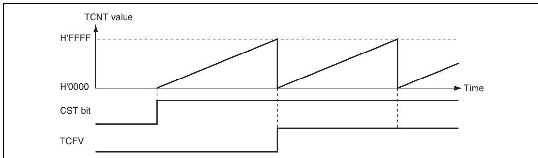
Figure 14.6 Free-Running Counter Operation
