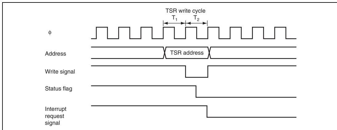
Figure 14.30 Timing for Status Flag Clearing by CPU
