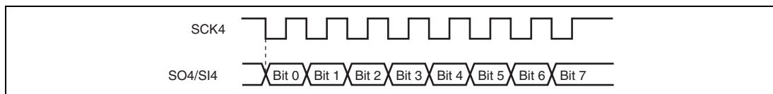
Figure 18.2 Data Transfer Format
