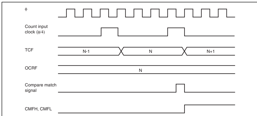
Figure 12.6 Compare Match Flag Set Timing
