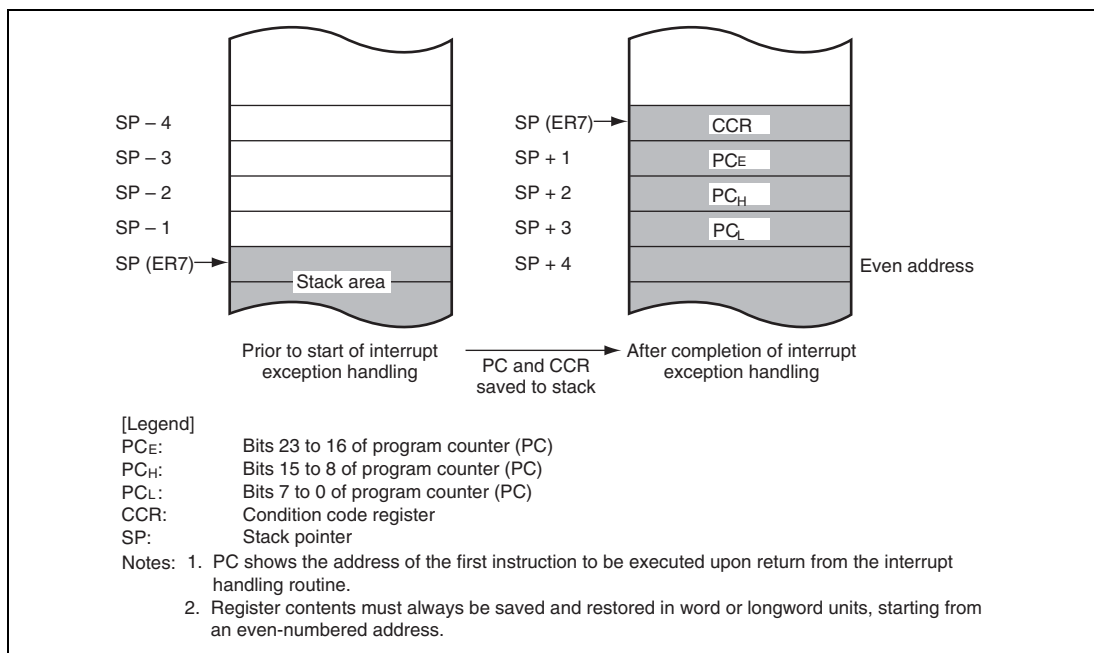
Figure 3.3 Stack Status after Exception Handling
