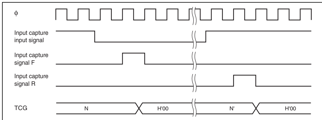
Figure 13.7 TCG Clear Timing
