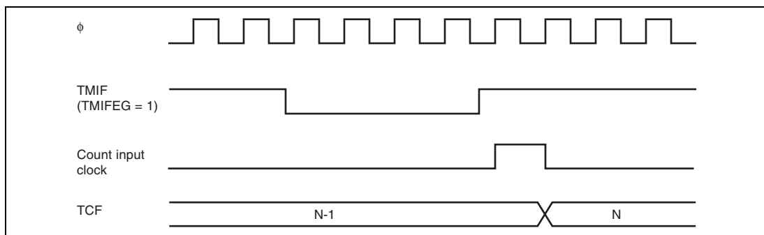
Figure 12.3 Count Timing for External Event Operation
