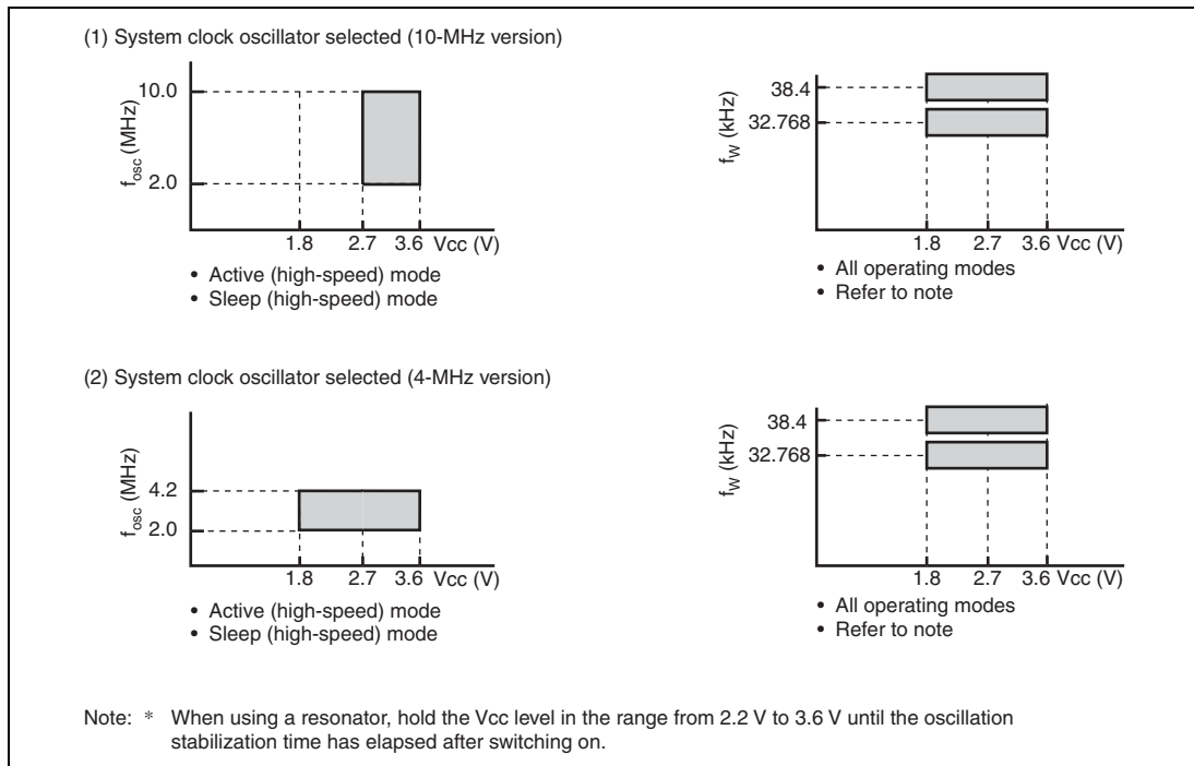
Figure 25.1 Power Supply Voltage and Oscillation Frequency Range (1)
