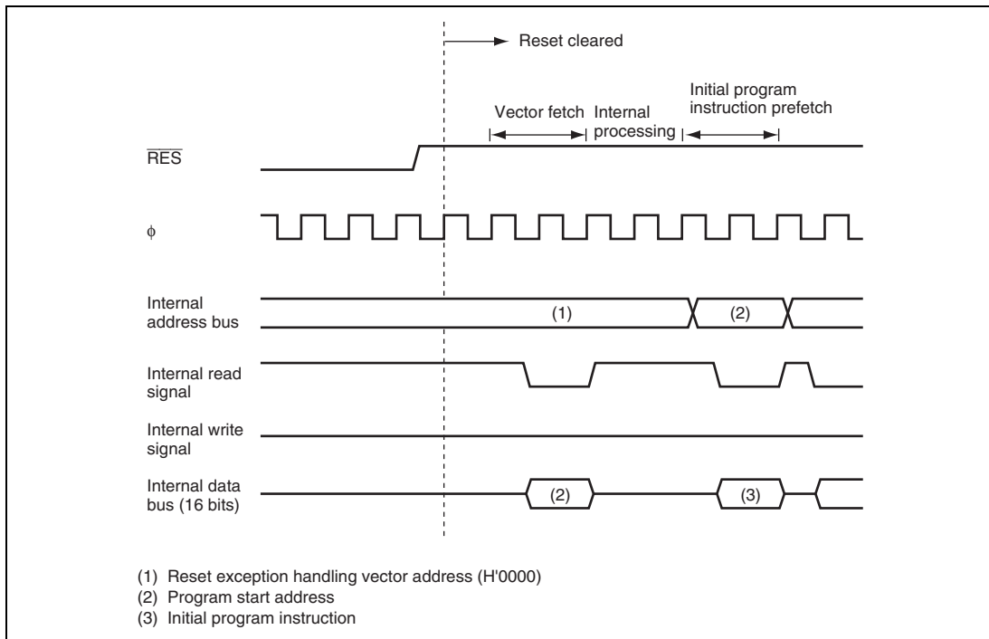
Figure 3.1 Reset Exception Handling Sequence
