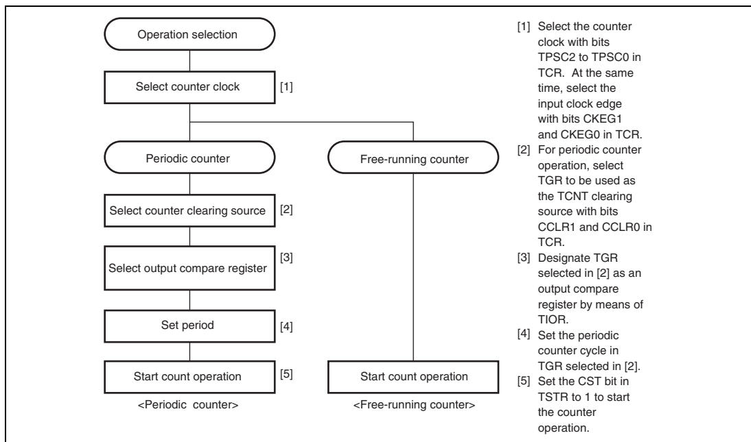
Figure 14.5 Example of Counter Operation Setting Procedure
