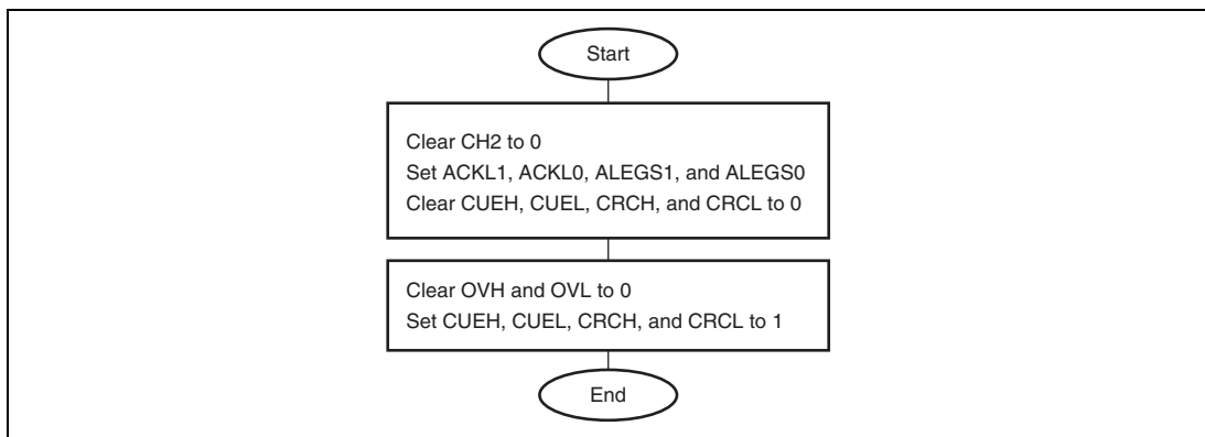
Figure 15.2 Software Procedure when Using ECH and ECL as 16-Bit Event Counter
