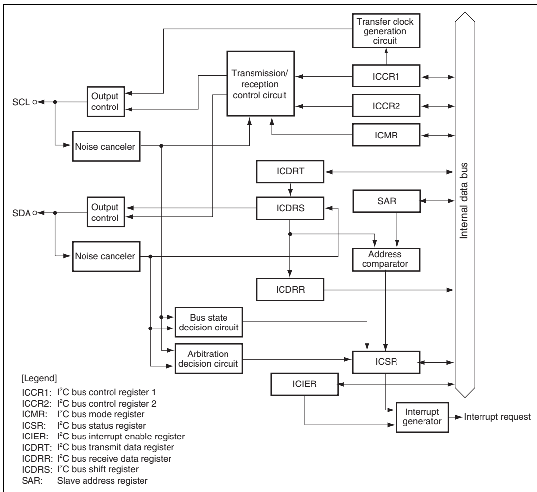
Figure 21.1 Block Diagram of I 2 C Bus Interface 2
