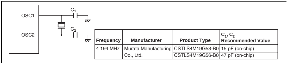
Figure 5.3 Typical Connection to Ceramic Resonator
