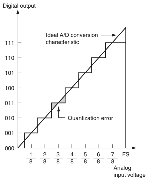
Figure 20.6 A/D Conversion Accuracy Definitions (1)
