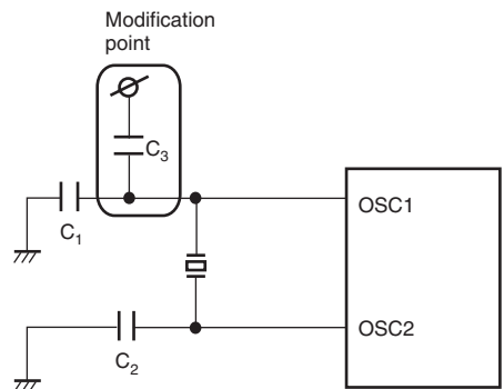
(2) Oscillator Circuit Modification Suggestion 1
