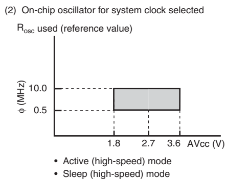
Figure 25.13 Analog Power Supply Voltage and Operating Frequency Range of A/D Converter (2)
