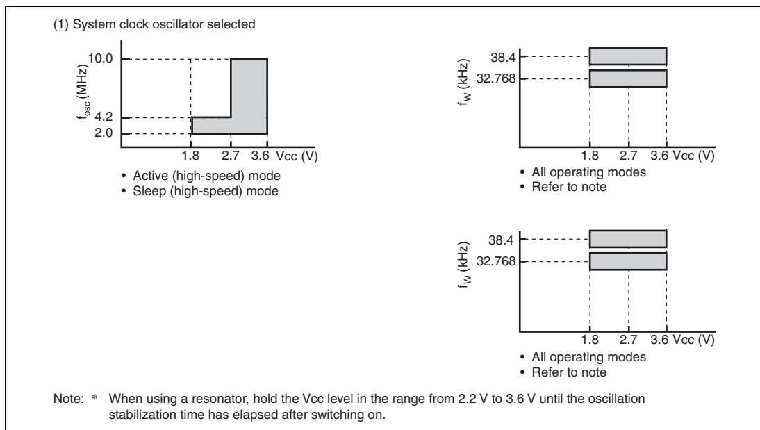
Figure 25.8 Power Supply Voltage and Oscillation Frequency Range (1)
