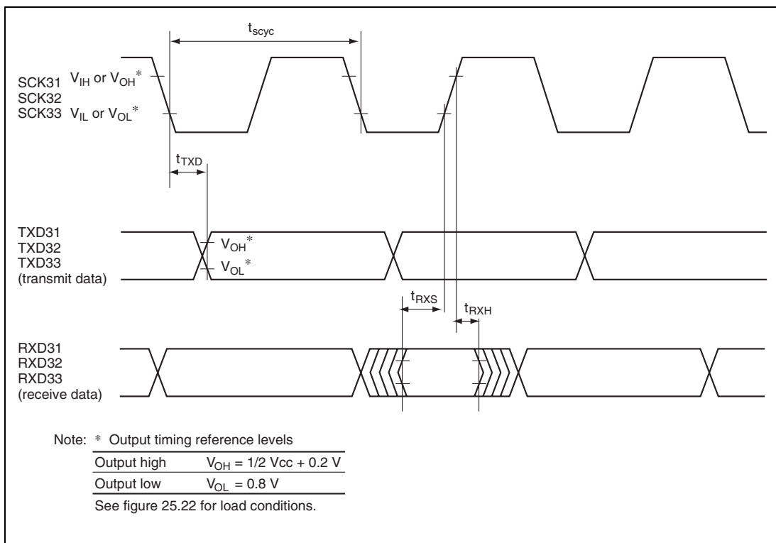
Figure 25.18 SCI3 Input/Output Timing in Clocked Synchronous Mode
