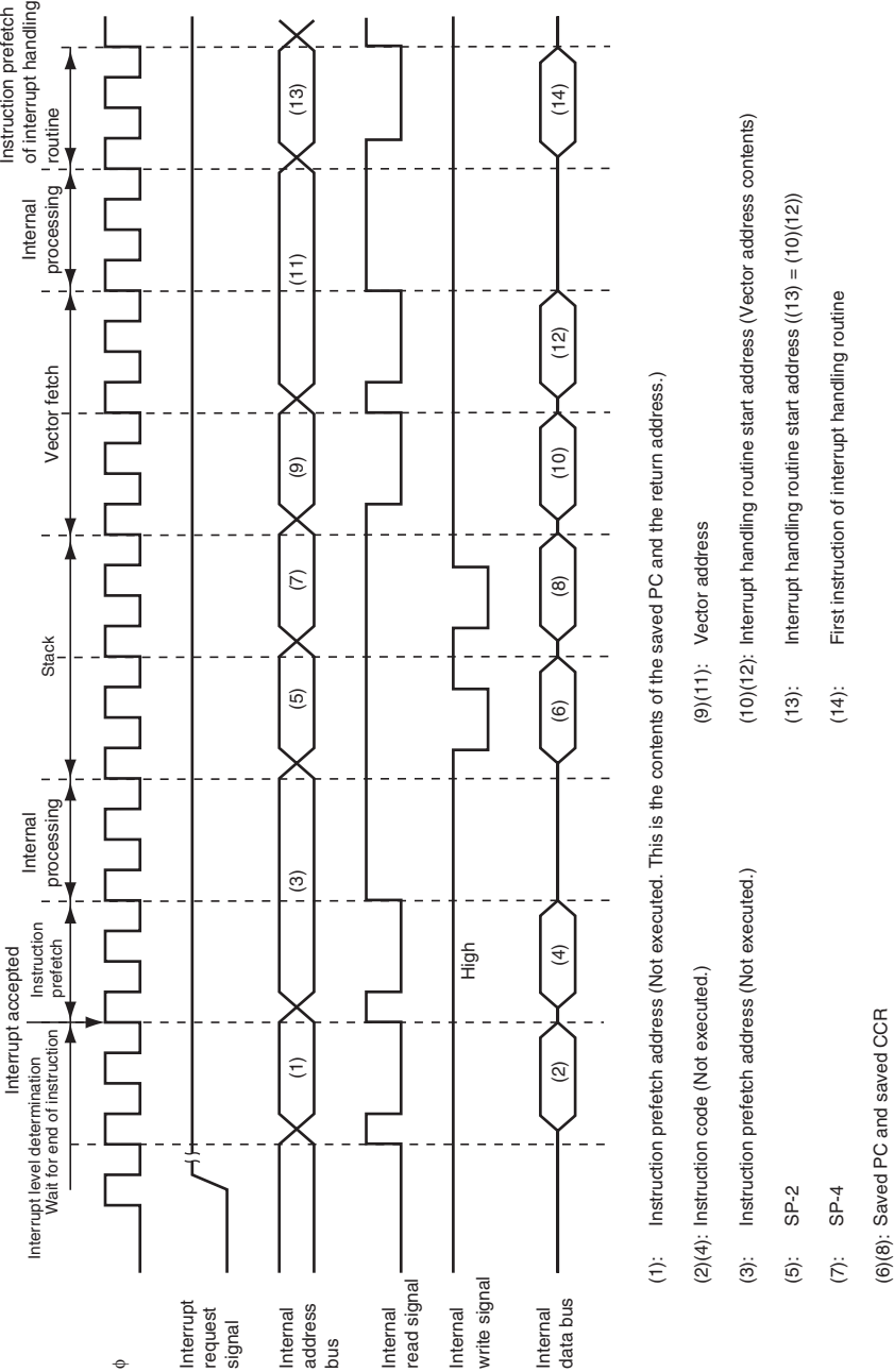
Figure 4.3 Interrupt Exception Handling Sequence
