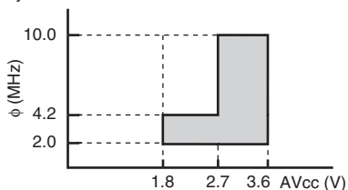
Figure 25.12 Analog Power Supply Voltage and Operating Frequency Range of A/D Converter (1)
