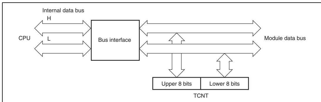
Figure 14.2 16-Bit Register Access Operation [CPU ↔ TCNT (16 Bits)]
