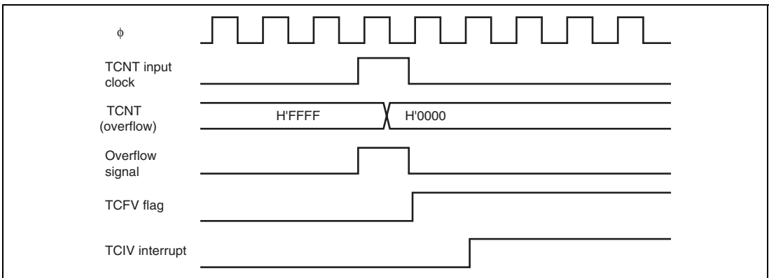
Figure 14.29 TCIV Interrupt Setting Timing
