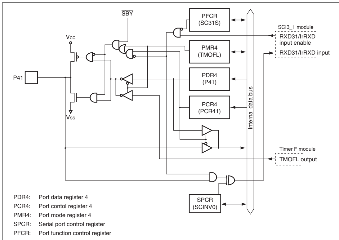
Figure B.3 (b) Port 4 Block Diagram (P41)
