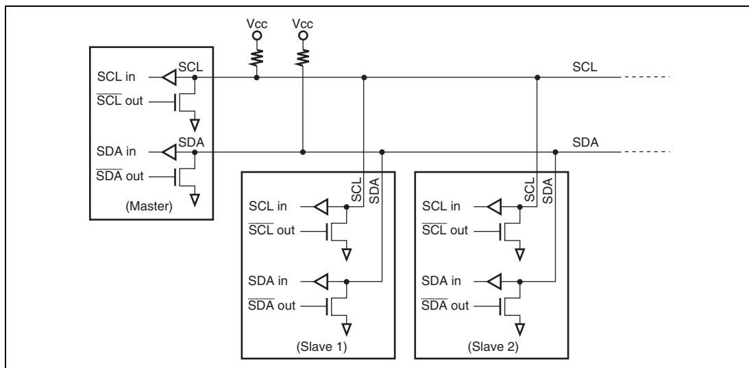
Figure 21.2 External Circuit Connections of I/O Pins
