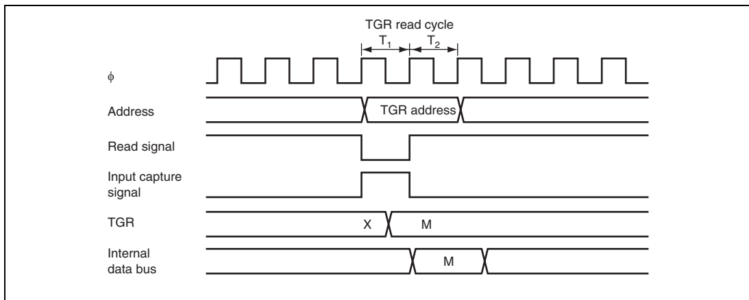
Figure 14.34 Contention between TGR Read and Input Capture
