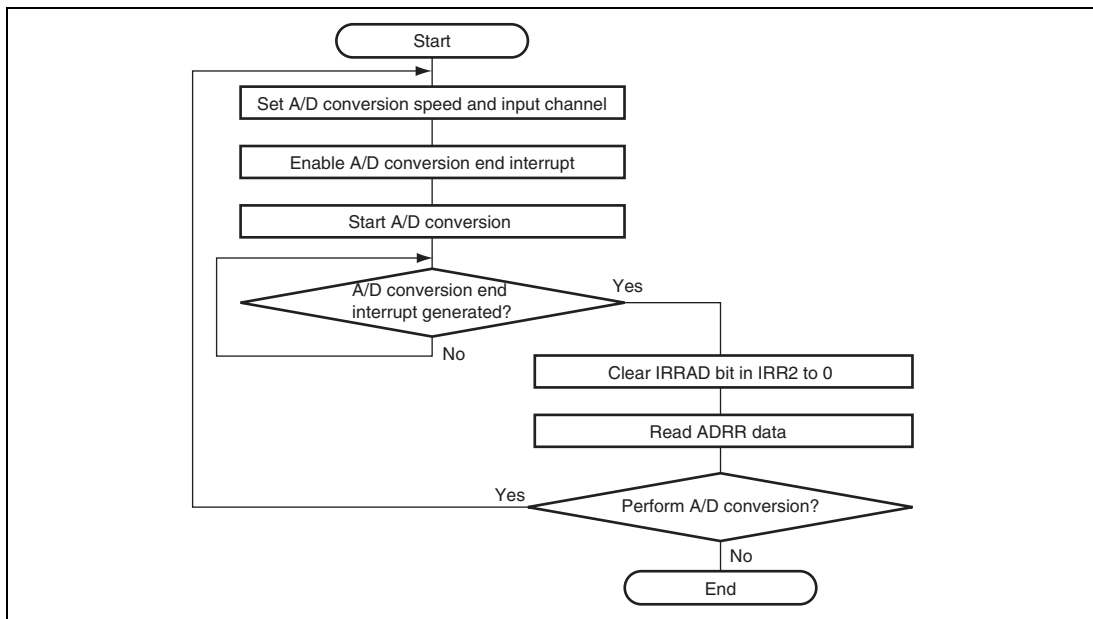
Figure 20.5 Flowchart of Procedure for Using A/D Converter (Interrupts Used)
