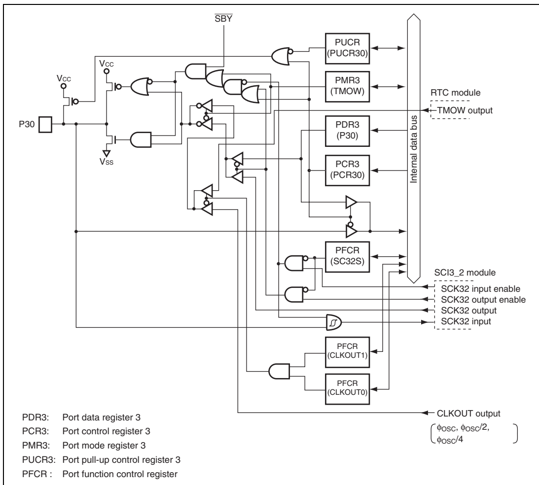
Figure B.2 (g) Port 3 Block Diagram (P30)
