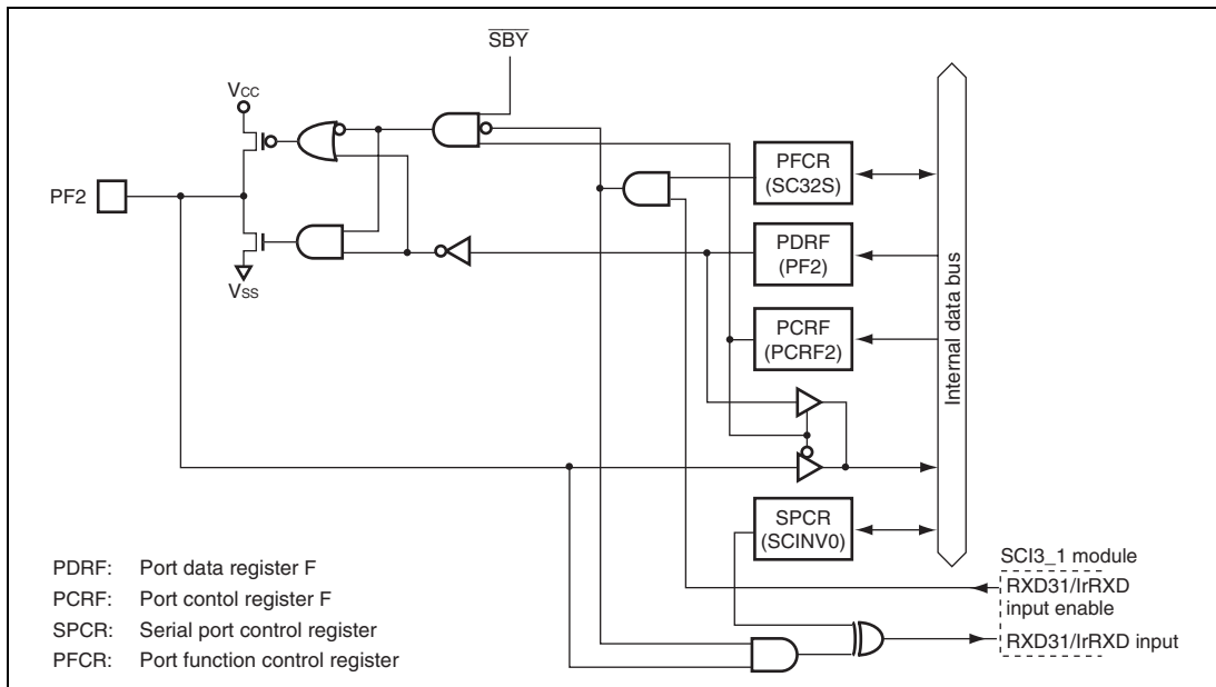
Figure B.13 (b) Port F Block Diagram (PF2)
