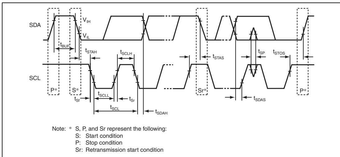
Figure 25.20 I²C Bus Interface Input/Output Timing
