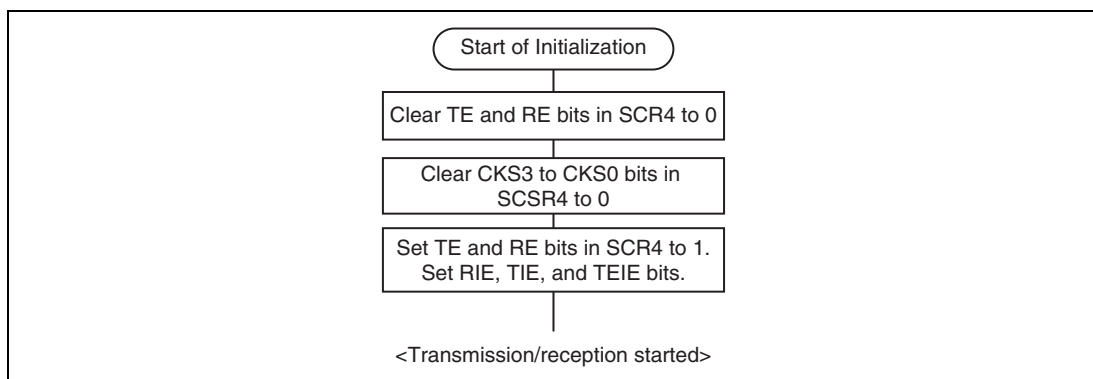
Figure 18.3 Flowchart Example of SCI4 Initialization
