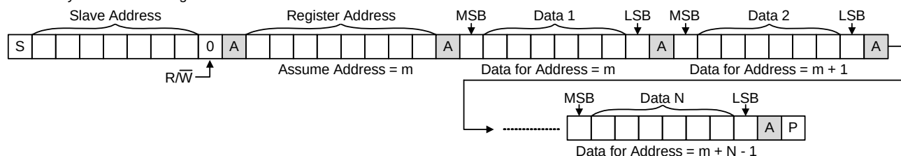
Figure 1. Read and Write Function
