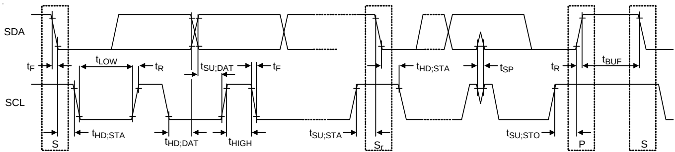
Figure 2. I²C Waveform Information
