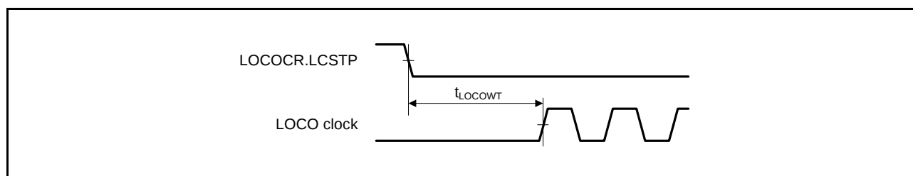
Figure 5.6 LOCO Clock Oscillation Start Timing
