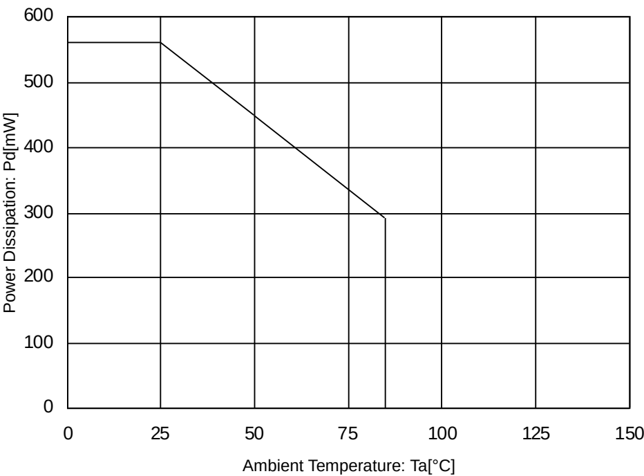
Figure 42. Power Dissipation Curve (Pd-Ta Curve)
