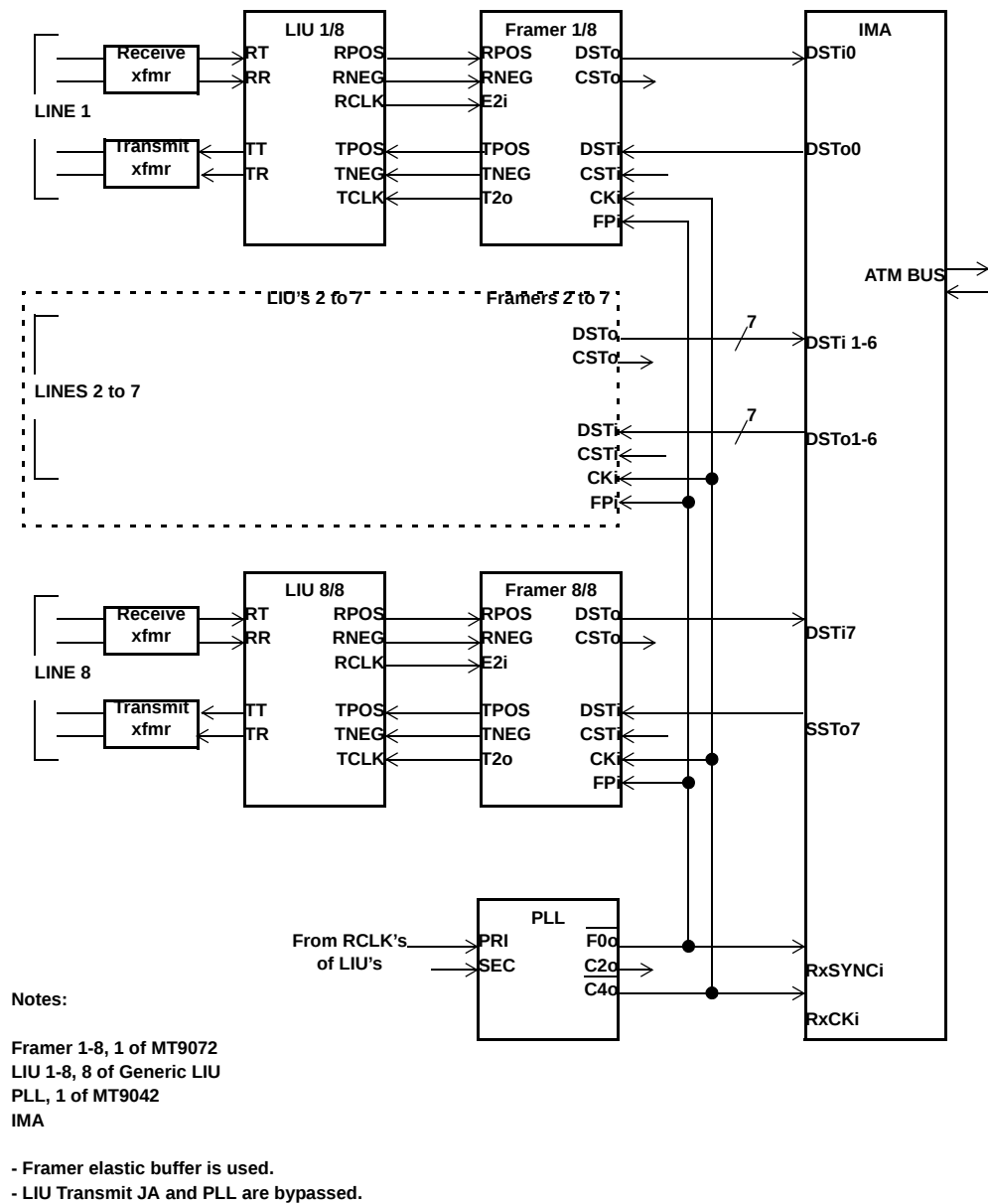
Figure 24 - 8 E1 Links with ATM IMA with Synchronous ST-BUS Mode
