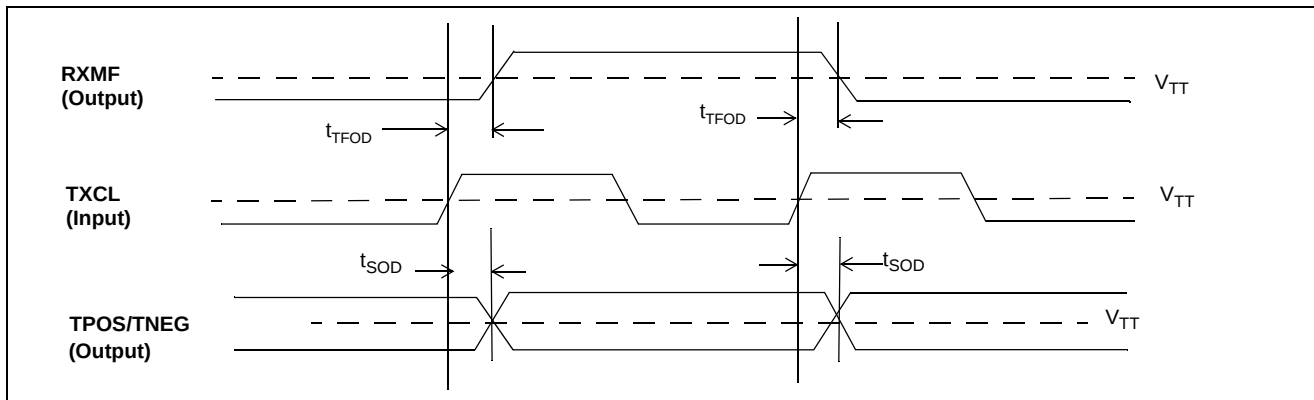
Figure 46 - Receive Multiframing Timing with TX8KEn Set Timing Diagram
