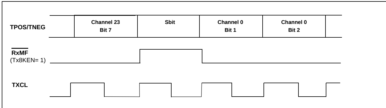
Figure 45 - Receive Multiframing Timing with TX8KEn Set Functional Timing Diagram
