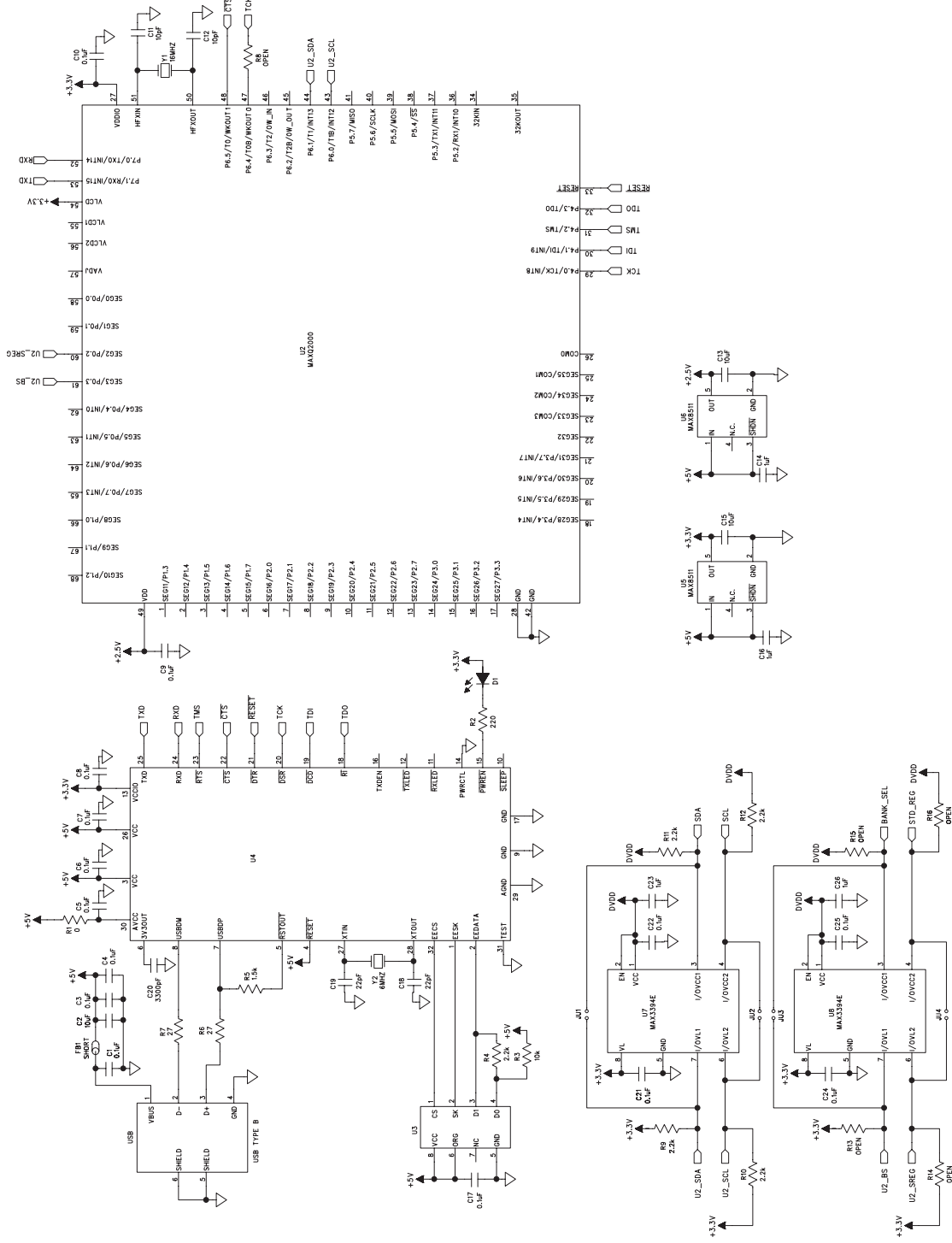
Figure 3b. MAX9591 EV Kit Schematic—USB-to-I 2 C Circuit (Sheet 2 of 2)
