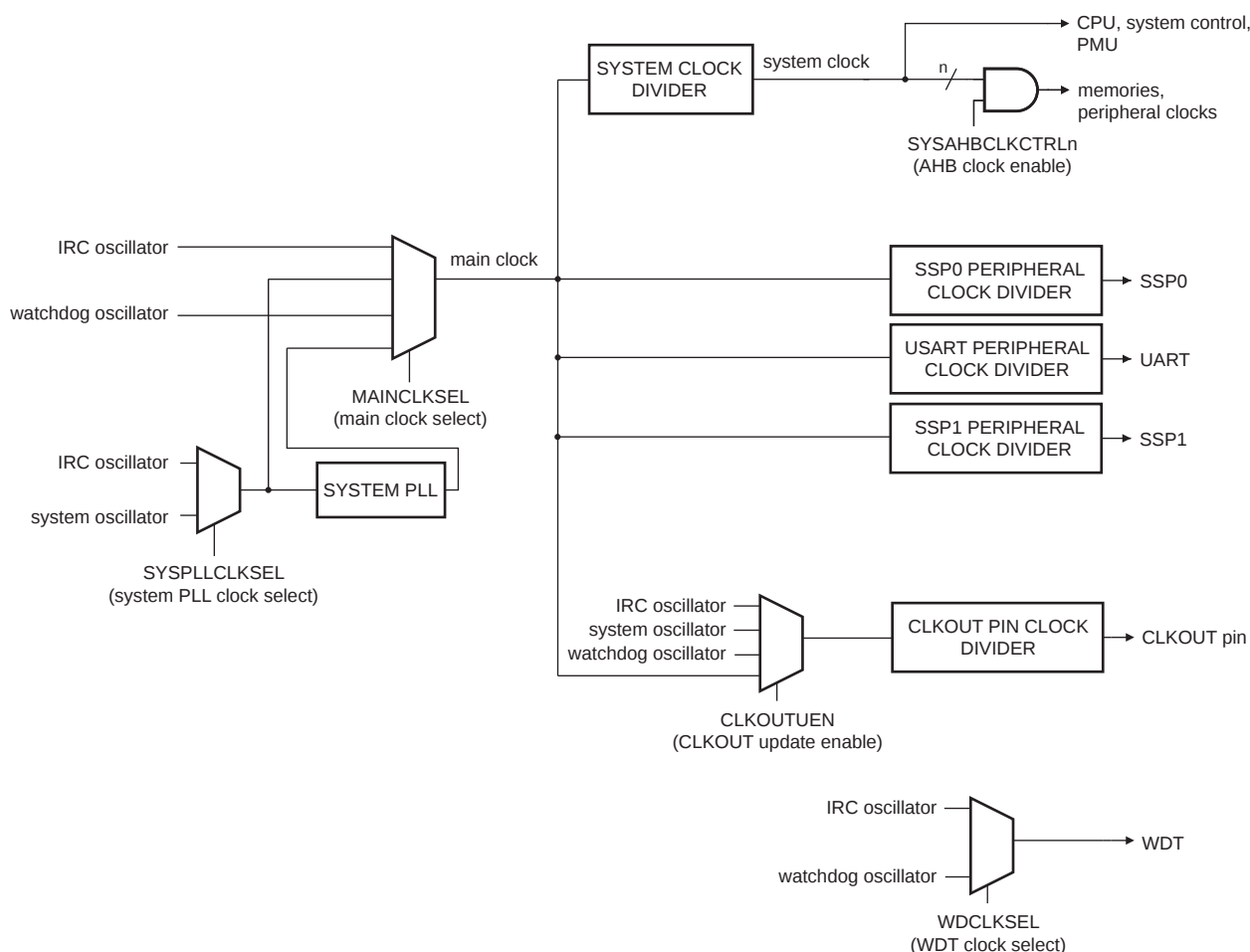
Fig 6. LPC11E3x clocking generation block diagram
