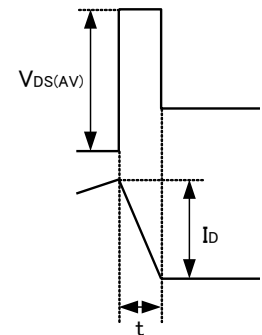
Figure 15-3. Waveform at Avalanche Breakdown
